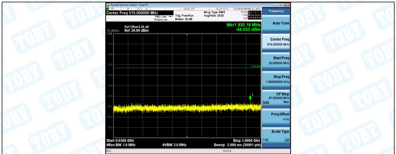
Band4-1413-1-30~1000MHz
