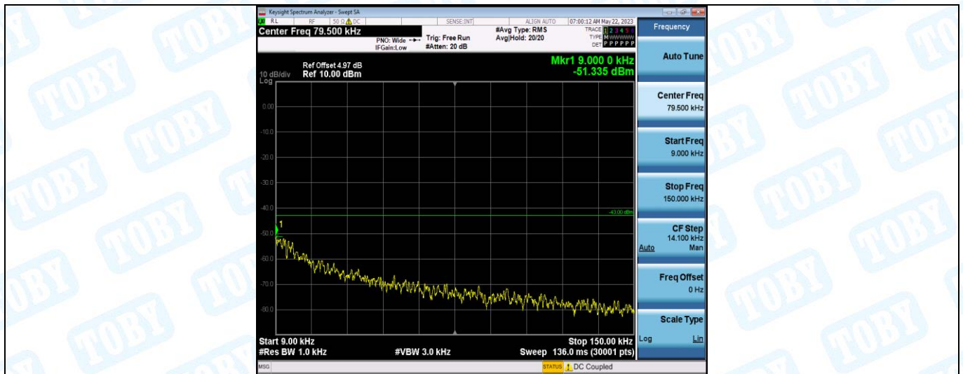
Band4-1513-3-0.009~0.15MHz
