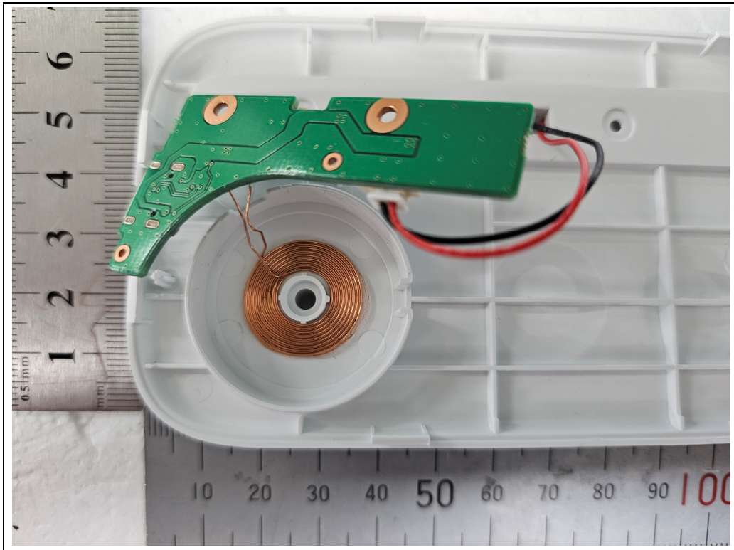
<Coil Antenna 2>
