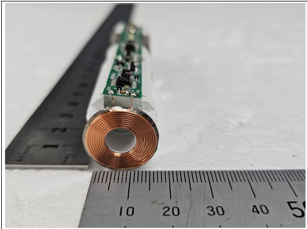
<Coil Antenna 1>
