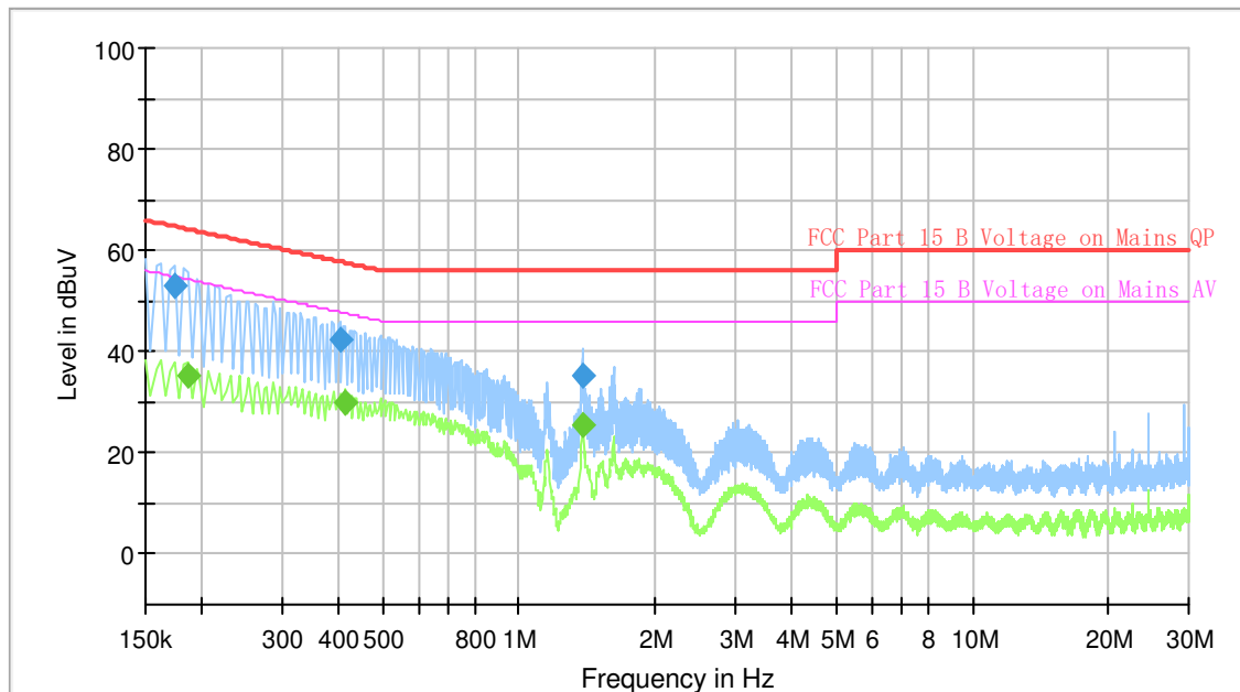
Full Spectrum
