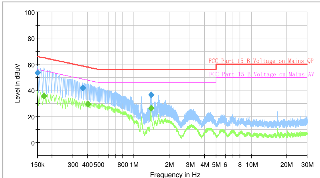
Full Spectrum
