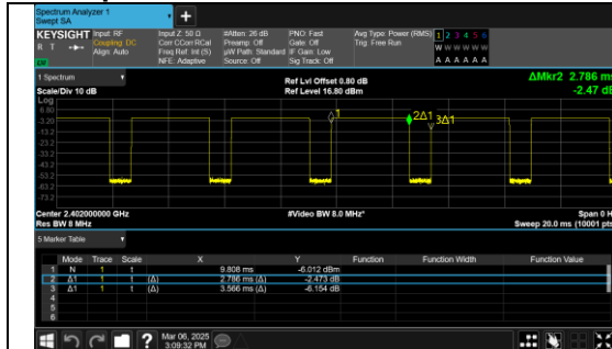
GFSK(DH5)_Channel 0
