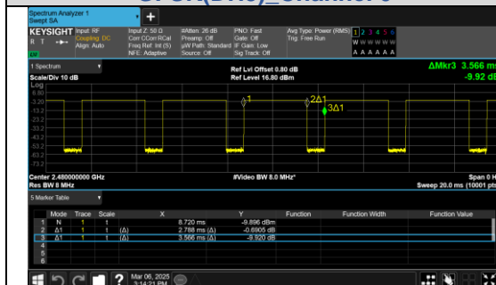
GFSK(DH5)_Channel 78
