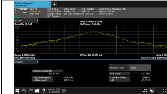
GFSK_DH5_Channel 78
