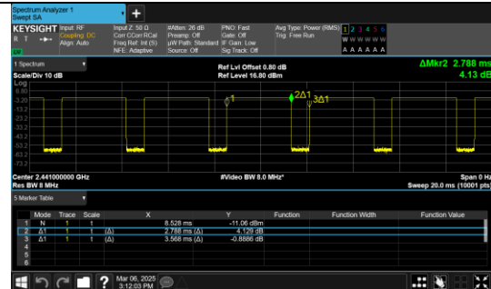
GFSK(DH5)_Channel 39
