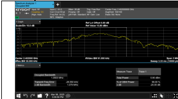
GFSK_DH5_Channel 0
