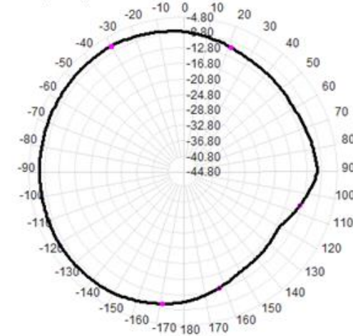
Total(H-XY), Max= -7.32dBi, CirD=8.96
