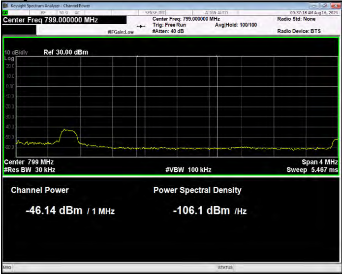
Band14 16QAM BW=5MHz Channel=23355 RB Size=1 Position=#0 Normal
