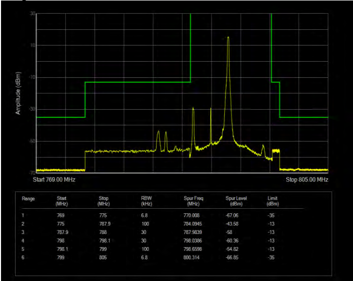
Band14 16QAM BW=5MHz Channel=23305 RB Size=25 Position=#0 Extended
