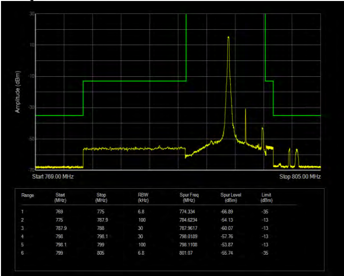
Band14 16QAM BW=5MHz Channel=23355 RB Size=1 Position=#Max Extended
