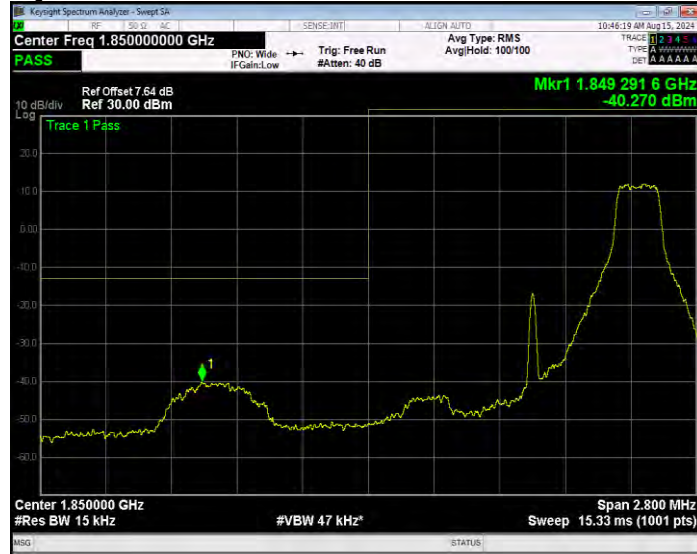
Band2 16QAM BW=1.4MHz Channel=18607 RB Size=6 Position=#0 Extended
