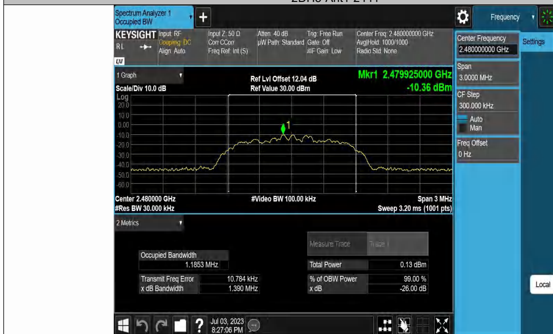
2DH5-Ant1-2480
