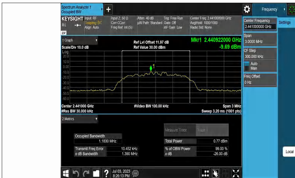
2DH5-Ant1-2441
