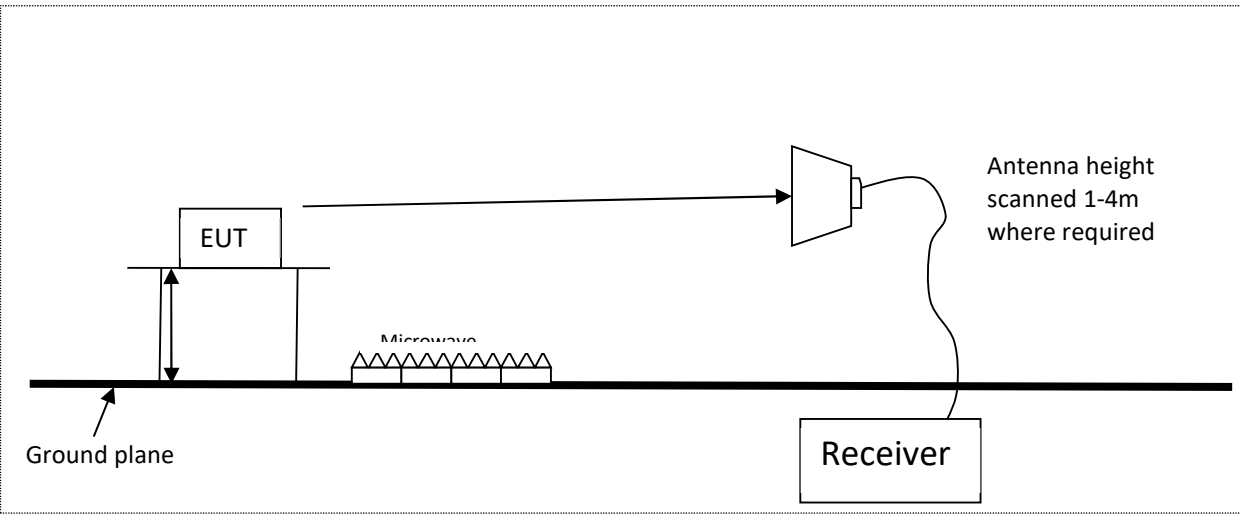
Diagram of the radiated emissions test setup 30 – 1000 MHz
