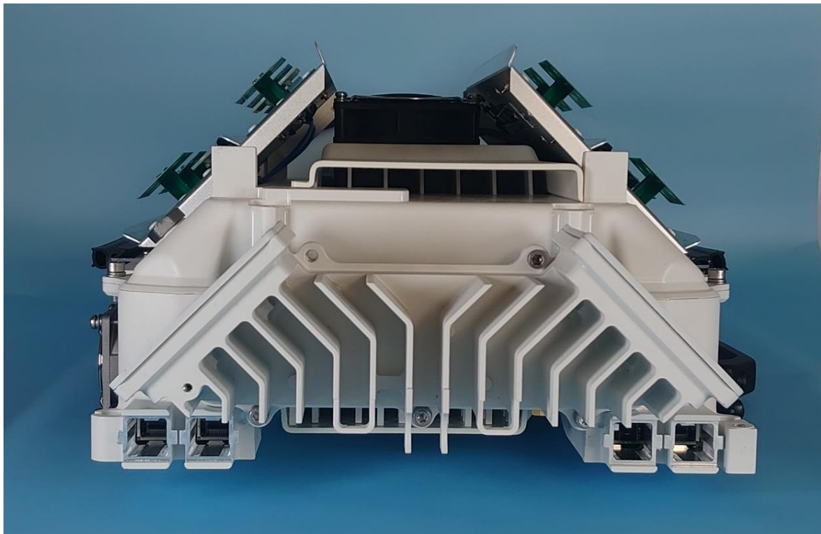
Figure 6: streetCell v1.1 Bottom View
