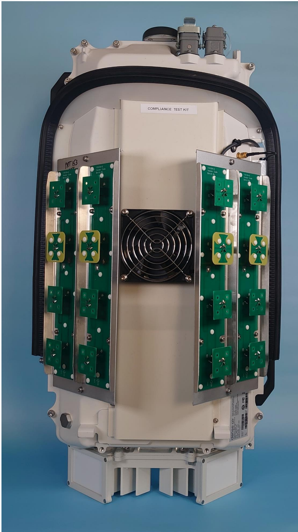
Figure 1: streetCell v1.1 Front View
