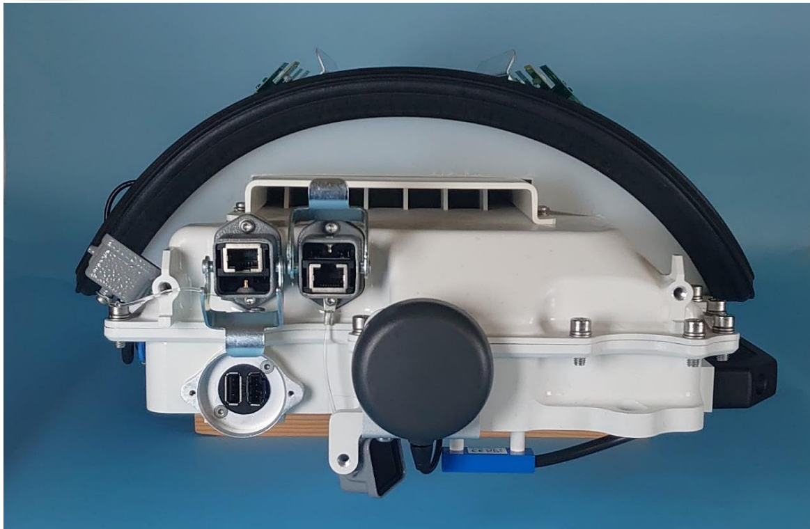
Figure 5: streetCell v1.1 Top View
