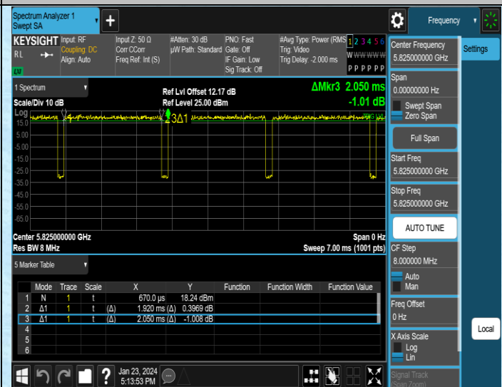
NTNV-11N20SISO-Ant1-5825
