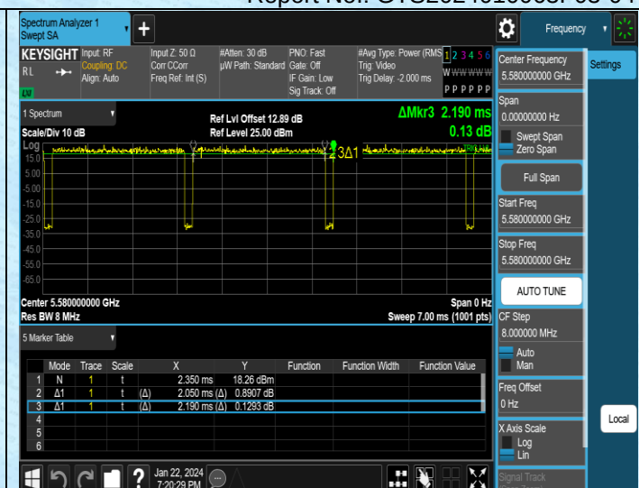
NTNV-11A-Ant1-5580
