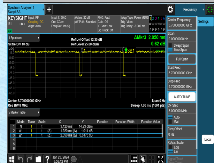
NTNV-11N20SISO-Ant1-5700
