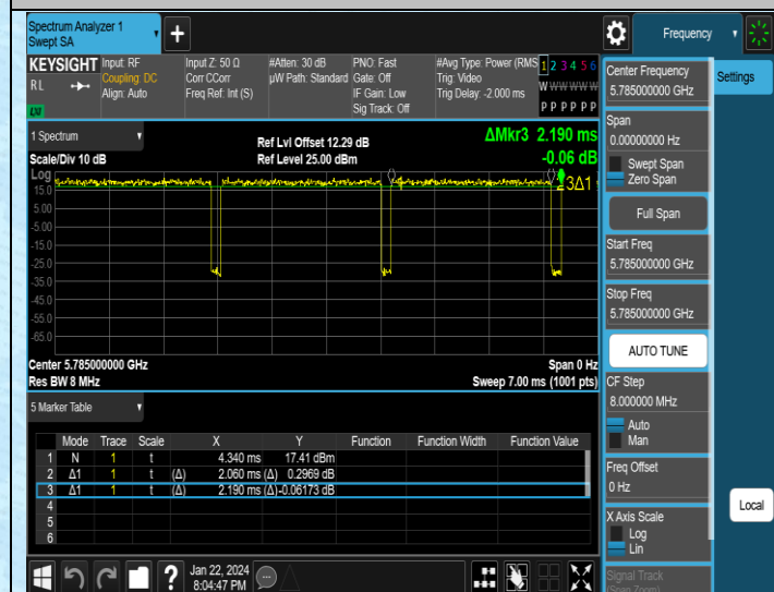
NTNV-11A-Ant1-5785
