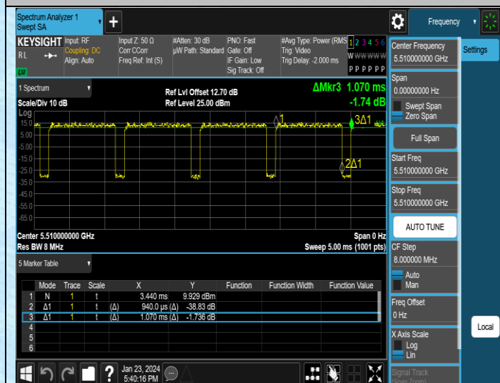
NTNV-11N40SISO-Ant1-5510
