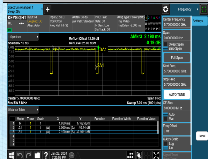
NTNV-11A-Ant1-5700
