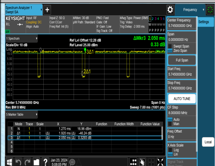
NTNV-11N20SISO-Ant1-5745
