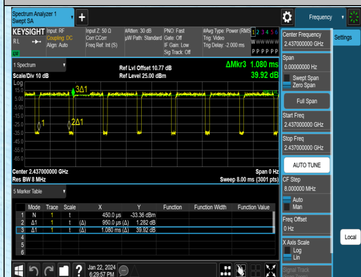
NTNV-11N40SISO-Ant1-2437
