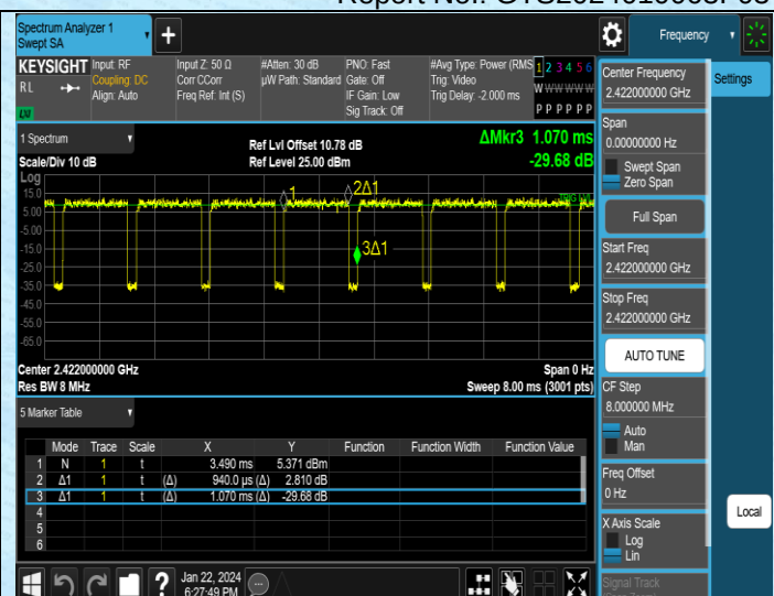
NTNV-11N40SISO-Ant1-2422
