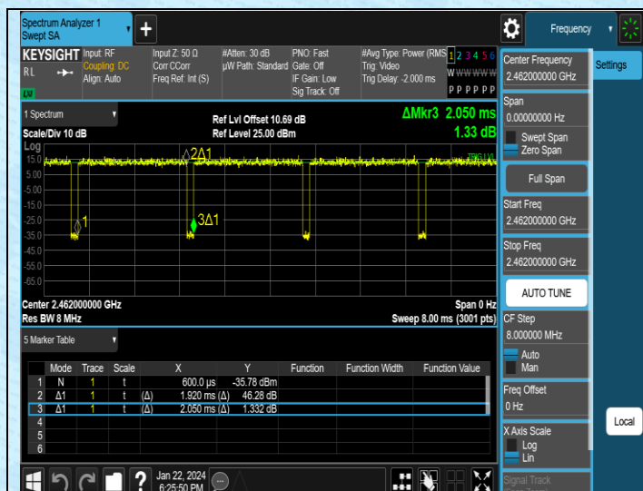
NTNV-11N20SISO-Ant1-2462
