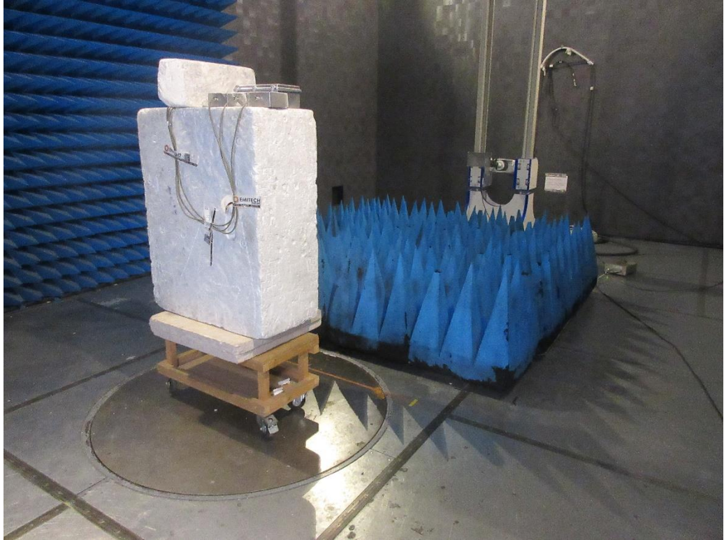
TEST SETUP PHOTOS – E.U.T. ON AZIMUTH 0° / FROM 1 GHz TO 2 GHz / VP
