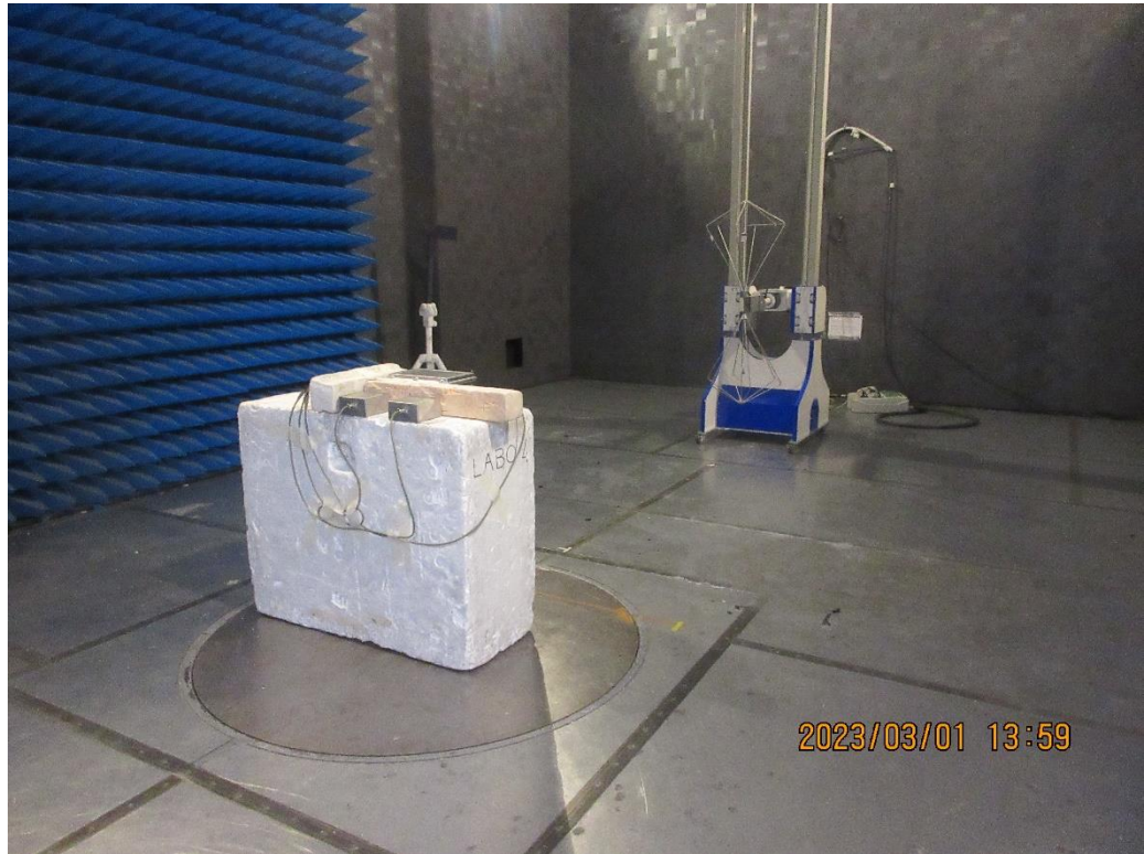
TEST SETUP PHOTOS – E.U.T. ON AZIMUTH 0° / FROM 30 MHz TO 200 MHz / VP
