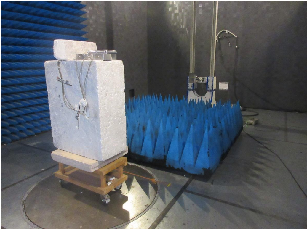
TEST SETUP PHOTOS – E.U.T. ON AZIMUTH 0° / FROM 1 GHz TO 2 GHz / HP
