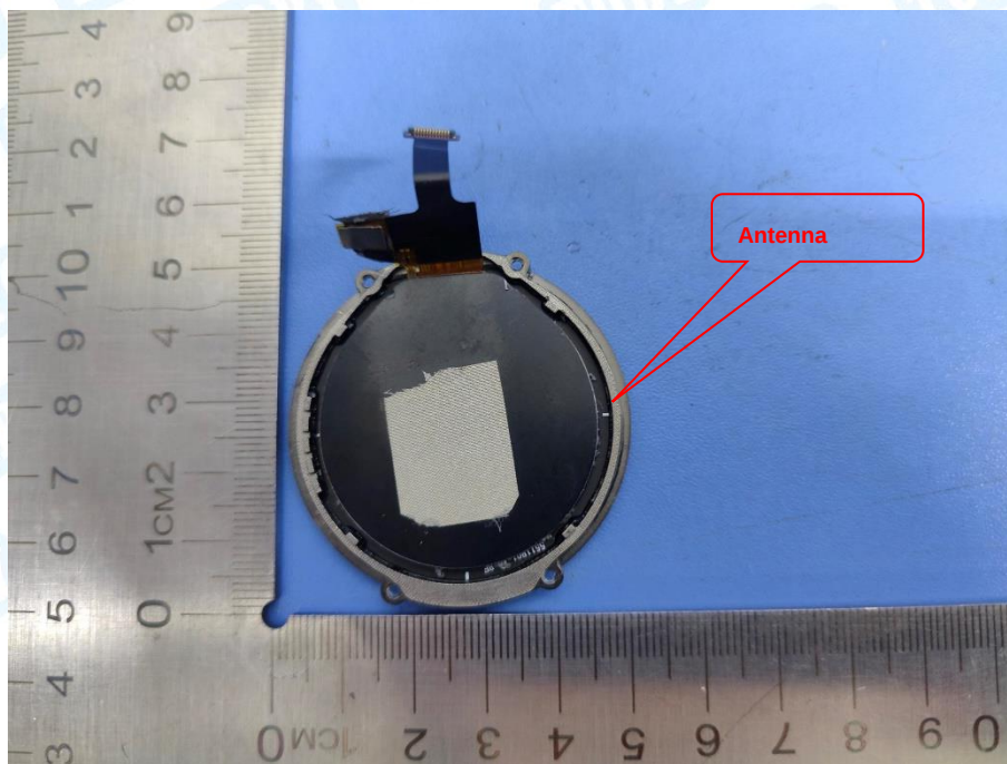
Photo 13 Antenna Appearance
