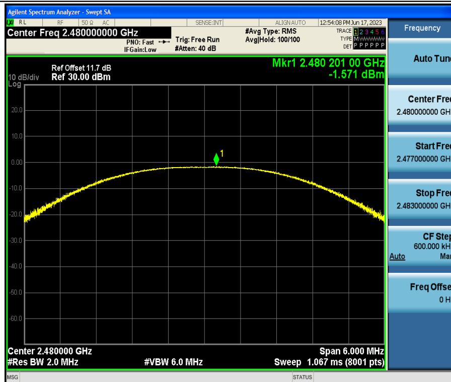
BLE_1M-Ant1-2480
