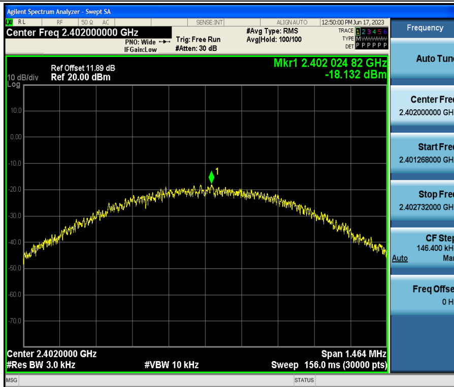
BLE_1M-Ant1-2402
