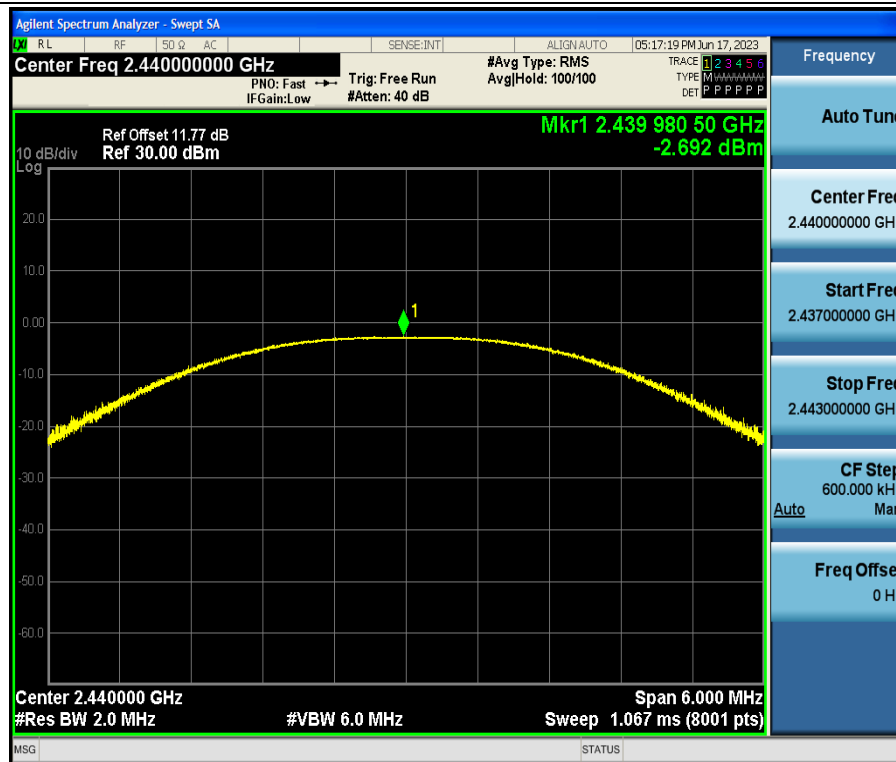
BLE_1M-Ant1-2440
