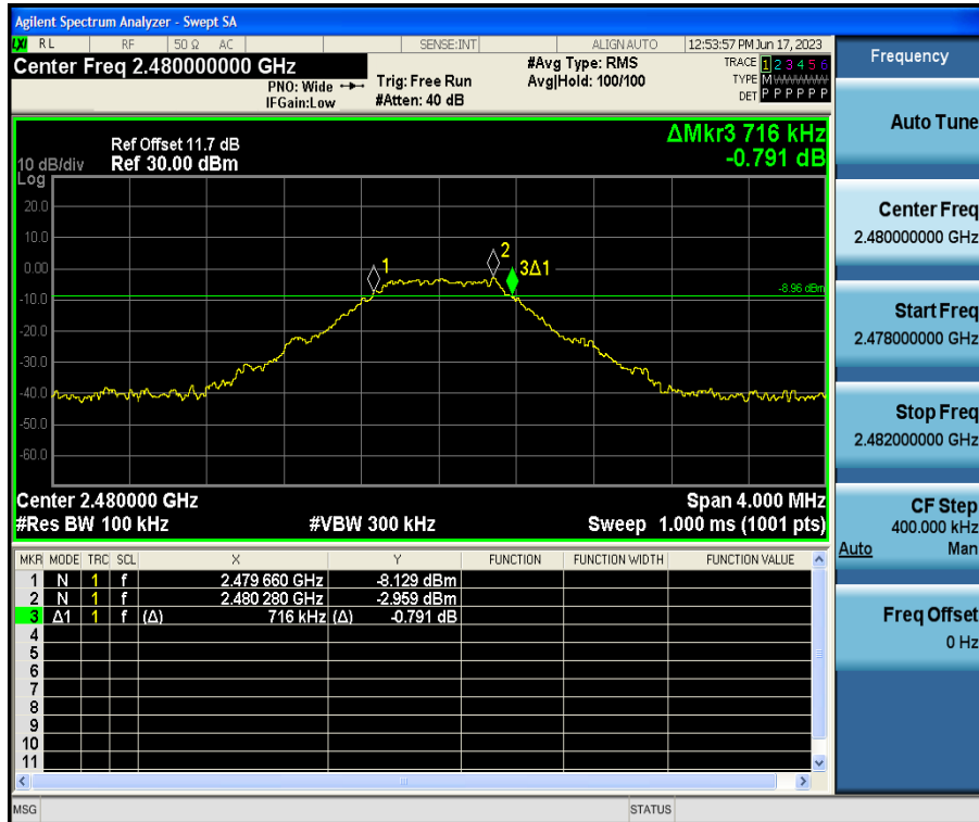
BLE_1M-Ant1-2480
