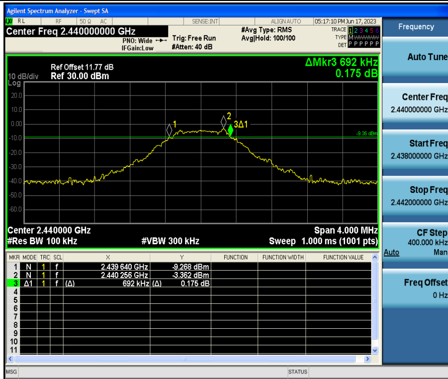
BLE_1M-Ant1-2440
