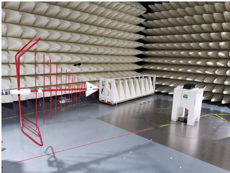
Figure B4: Radiated Emission test setup Low Range 1.
