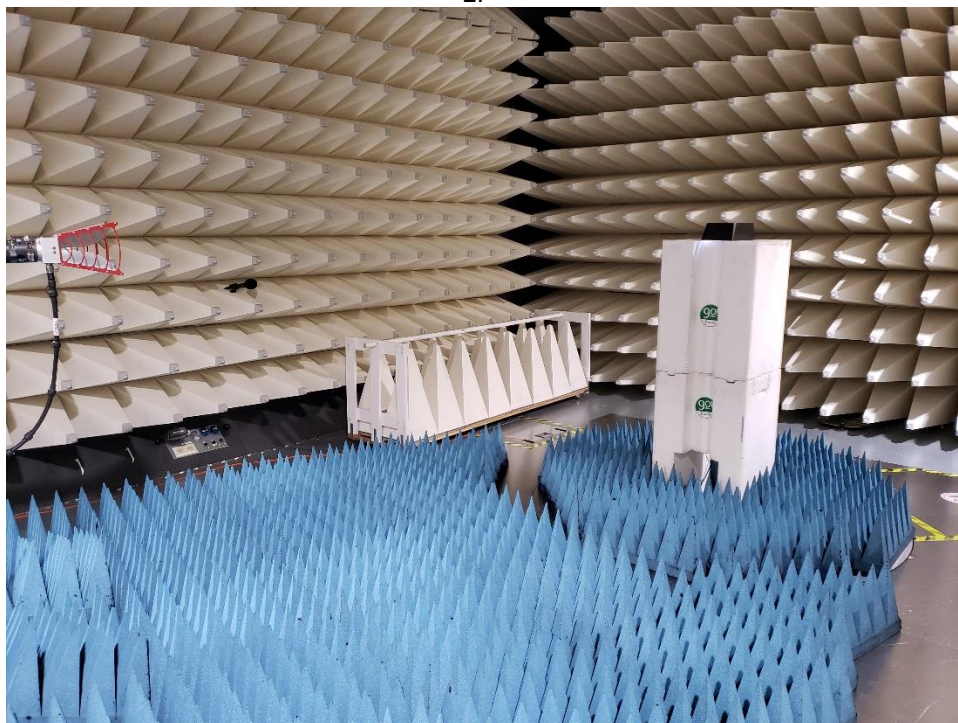
Figure B5: Radiated Emission test setup High Range 1
