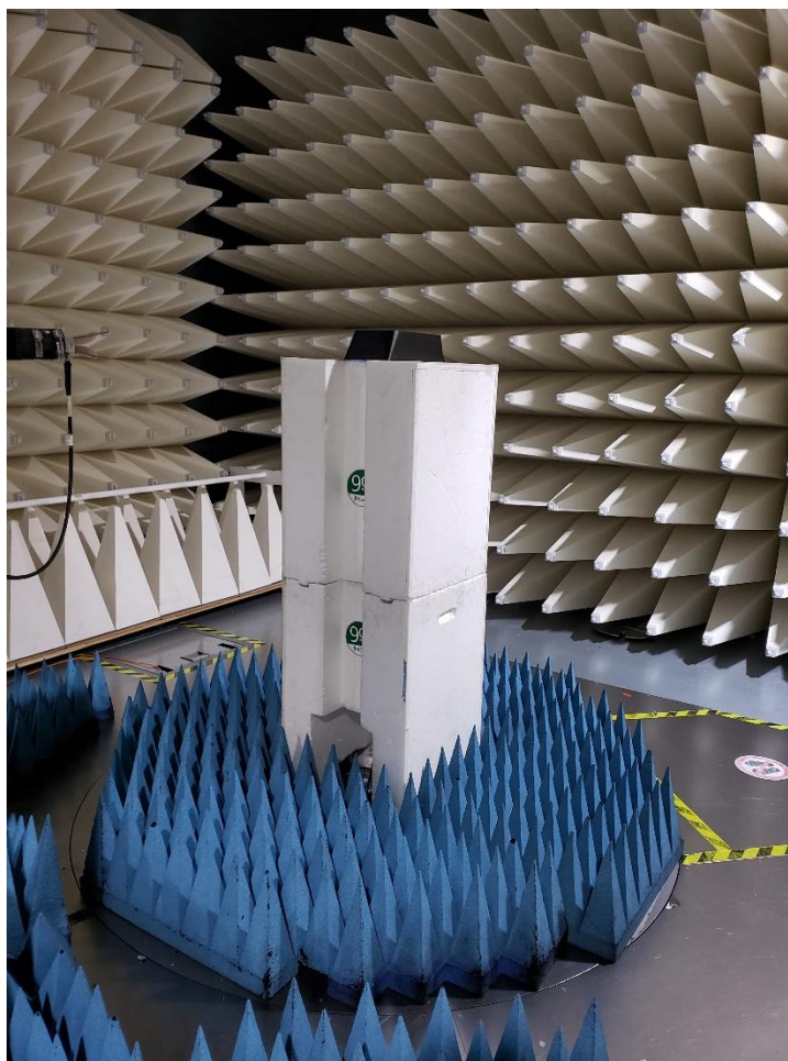
Figure B6: Radiated Emission test setup High Range 2
