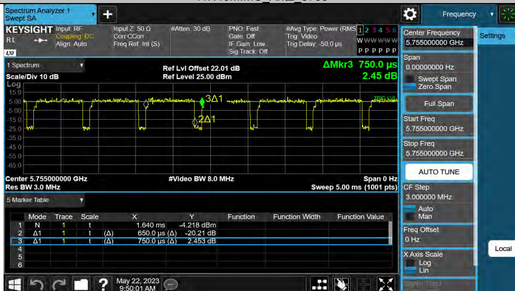
11N40MIMO Ant2 5755
