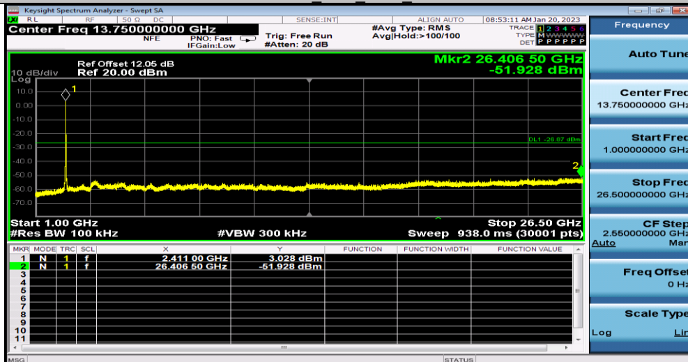
11N20SISO Ant1 2412 1000-26500
