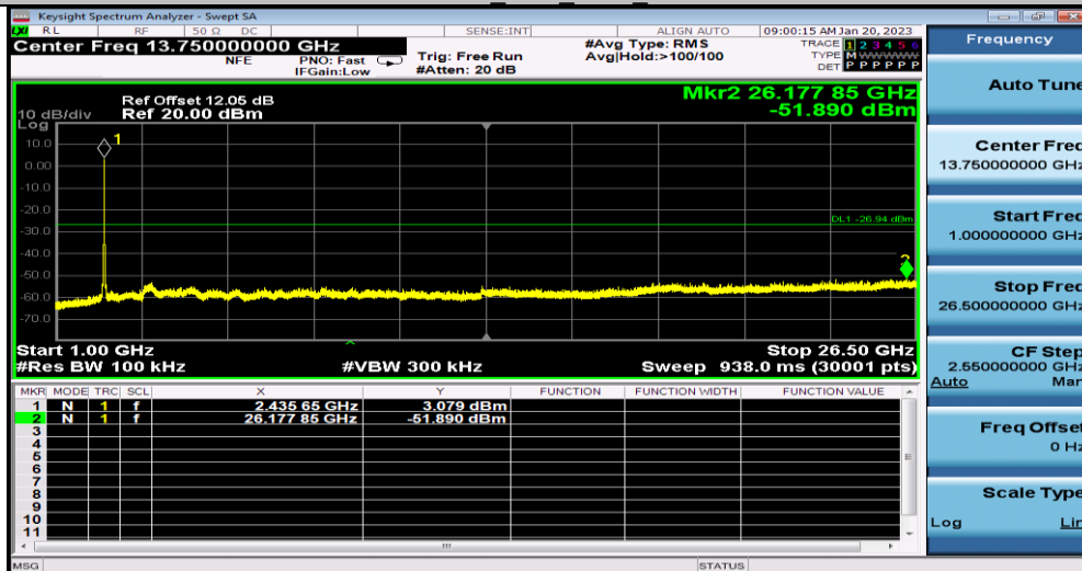
11N20SISO Ant1 2437 1000-26500
