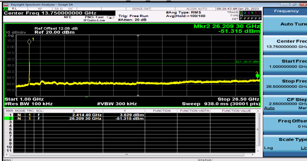
11G_Ant1_2412_1000-26500
