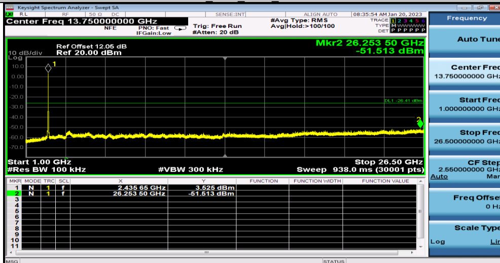
11G_Ant1_2437_1000-26500
