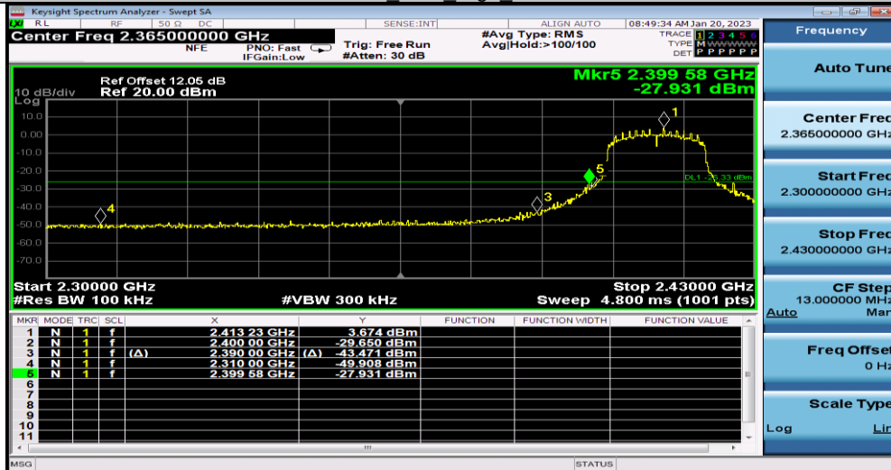
11N20SISO_Ant1_Low_2412
