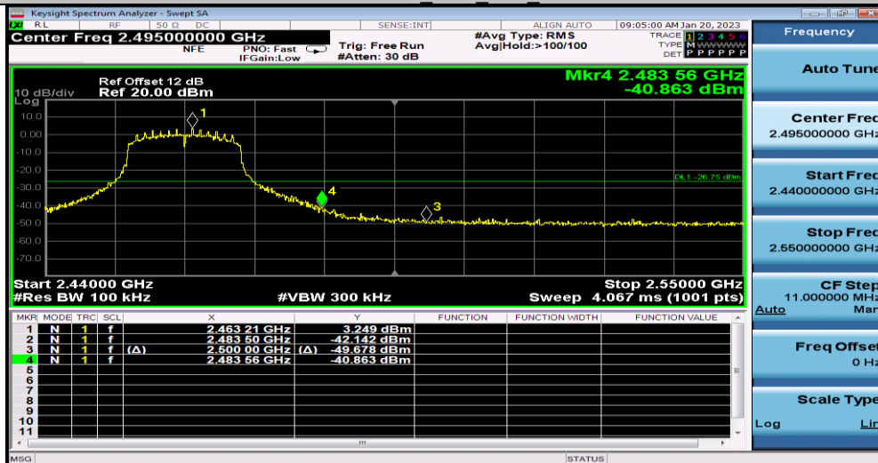
11N20SISO_Ant1_High_2462
