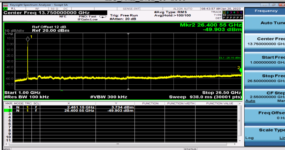
11G_Ant1_2462_1000-26500
