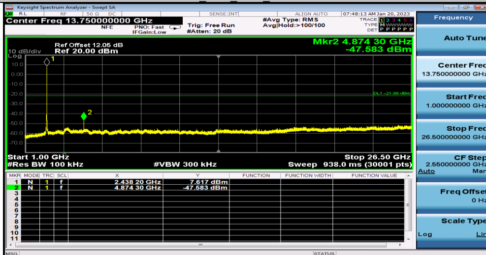
11B_Ant1_2437_1000-26500
