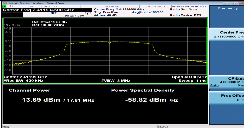
11N20SISO_Ant1_2412
