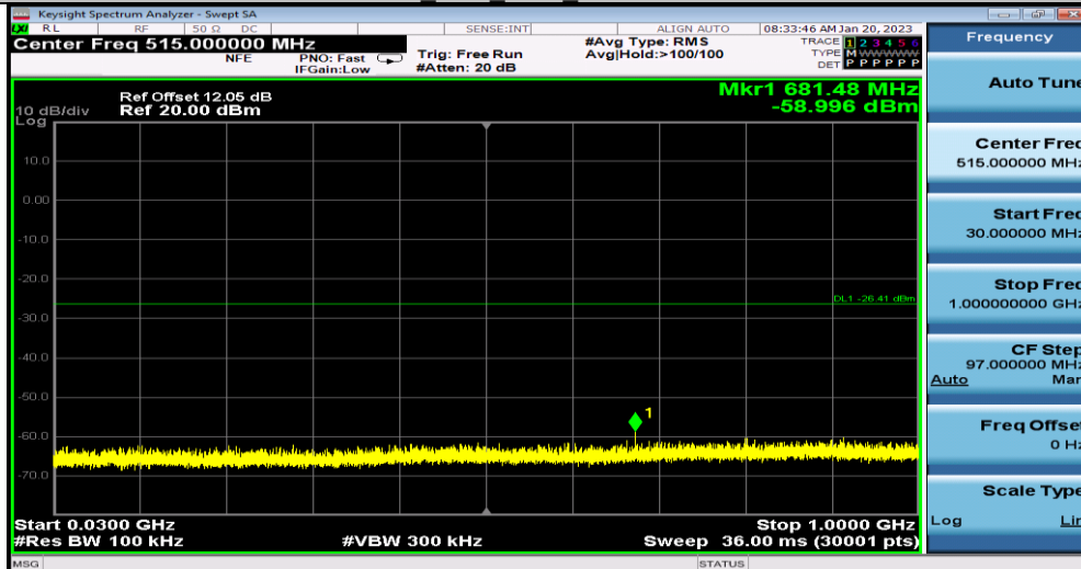
11G_Ant1_2437_30-1000
