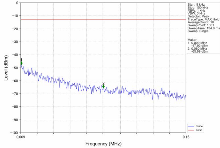
Band66_5MHz_16QAM_LCH_1712.5MHz_RB_1_0_NTNV
