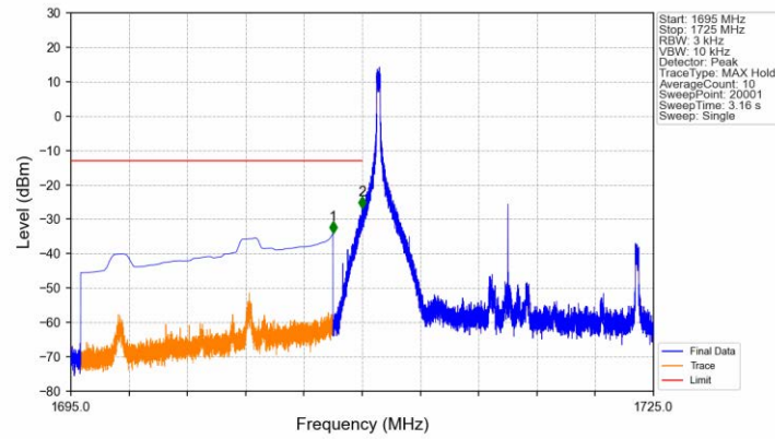
Band66_15MHz_QPSK_LCH_1717.5MHz_RB_1_0_NTNV
