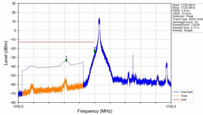
Band66_10MHz_QPSK_LCH_1715MHz_RB_1_0_NTNV
