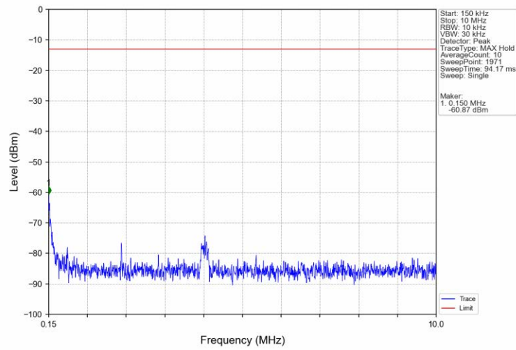
Band66_3MHz_16QAM_LCH_1711.5MHz_RB_1_0_NTNV
