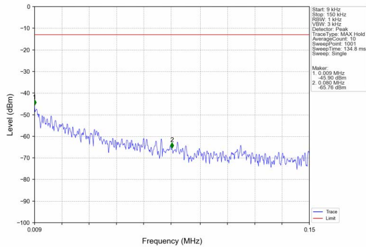
Band66_3MHz_QPSK_LCH_1711.5MHz_RB_1_0_NTNV
