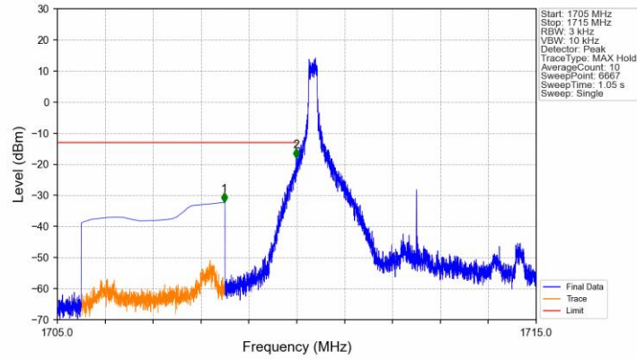
Band66_5MHz_QPSK_LCH_1712.5MHz_RB_1_0_NTNV
