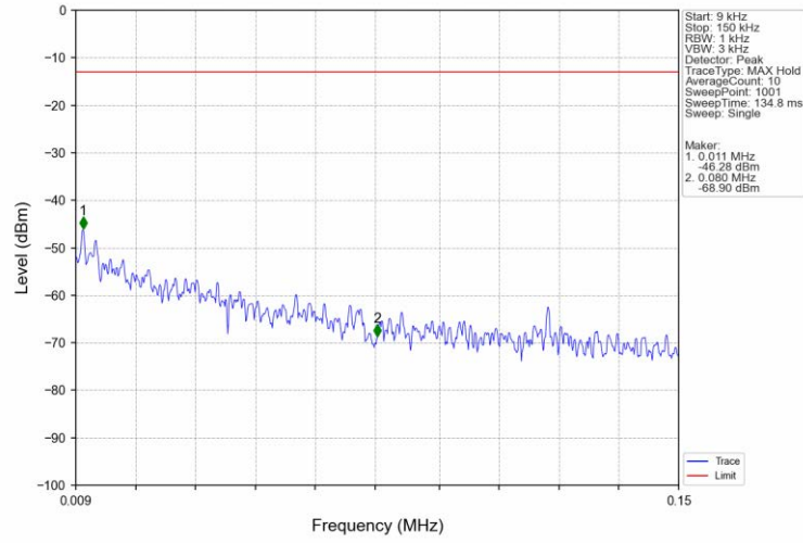
Band66_3MHz_16QAM_LCH_1711.5MHz_RB_1_0_NTNV
