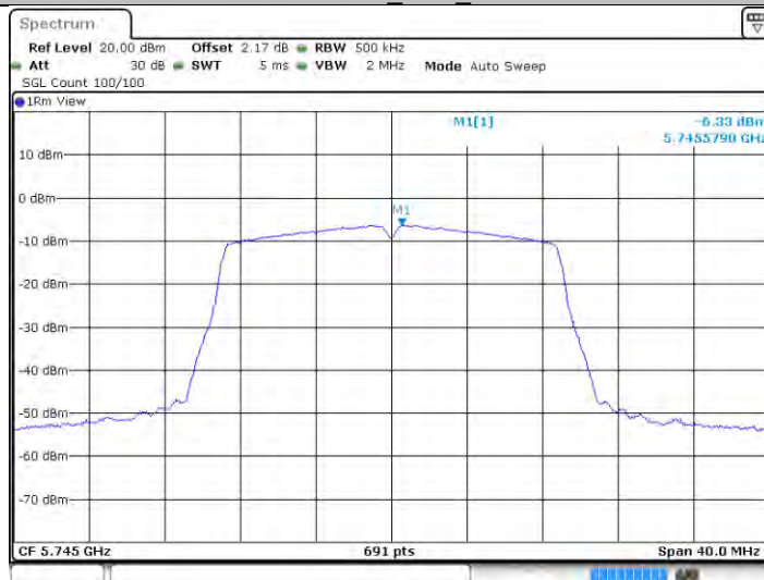
11n20SISO_Ant3_5745
