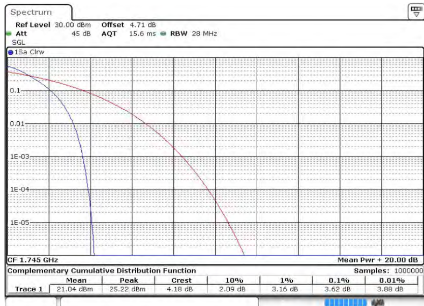
Band66-20MHz-QPSK-132322-100RB#0
