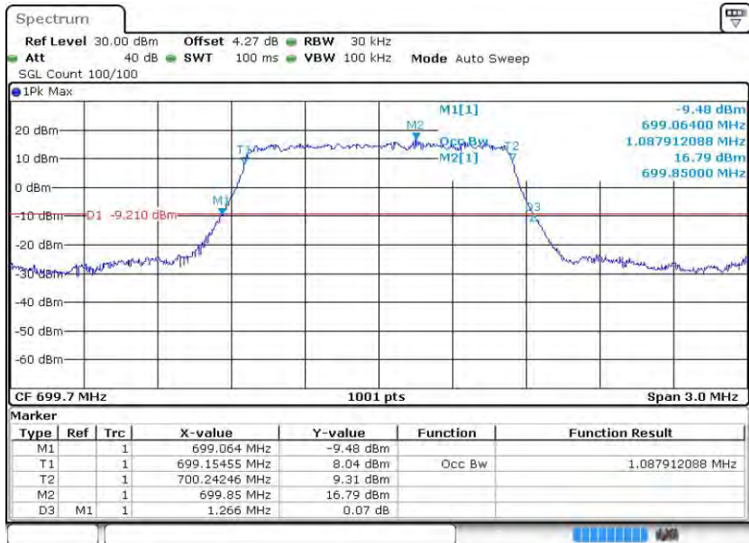
Band12-1.4MHz-QPSK-23017-6RB#0
