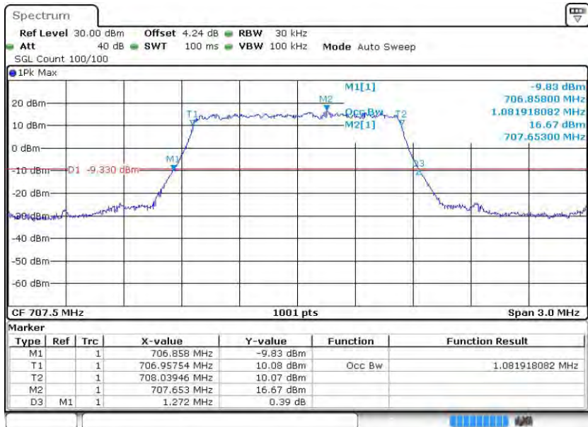
Band12-1.4MHz-QPSK-23095-6RB#0
