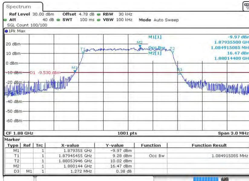
Band2-1.4MHz-QPSK-18900-6RB#0
