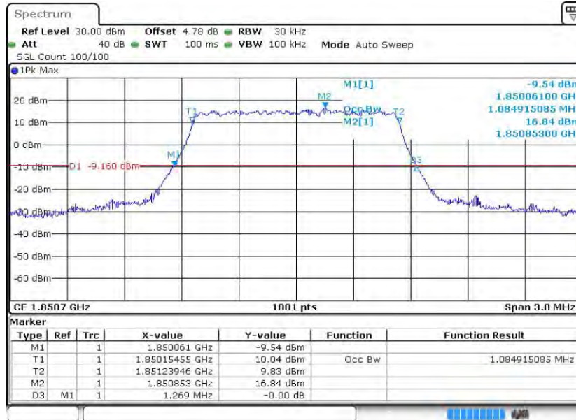
Band2-1.4MHz-QPSK-18607-6RB#0
