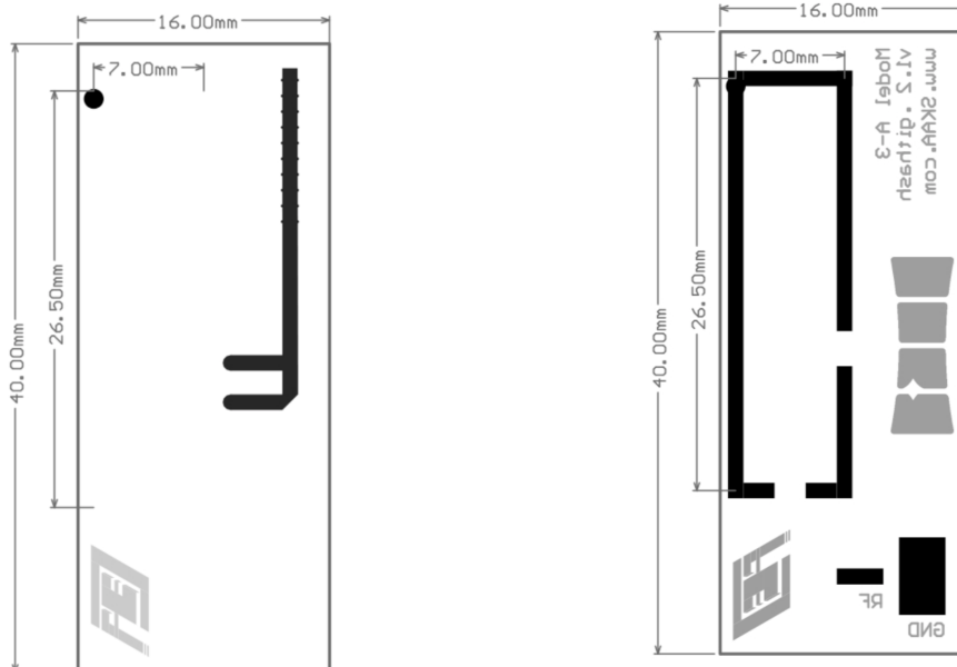
Cable Assembly with Antenna Board
