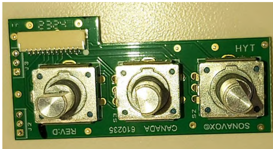
Figure 4 – Knob Board -Top
