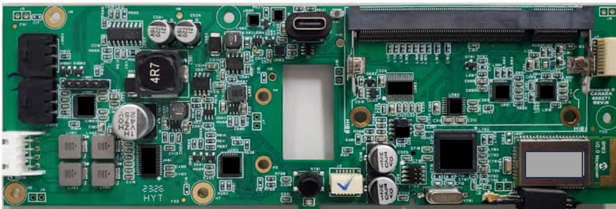
Figure 3 – Main PCB with Transmitter -Top with daughter board removed
