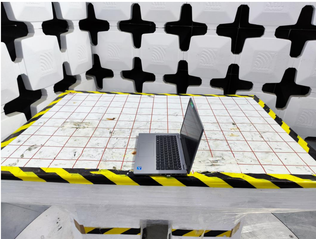
Up to 1GHz The EUT is placed at the center of turntable
