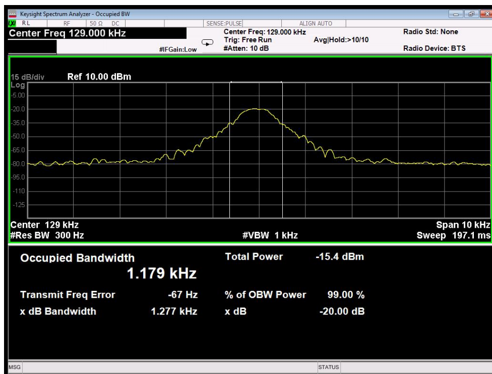
20dB Bandwidth
