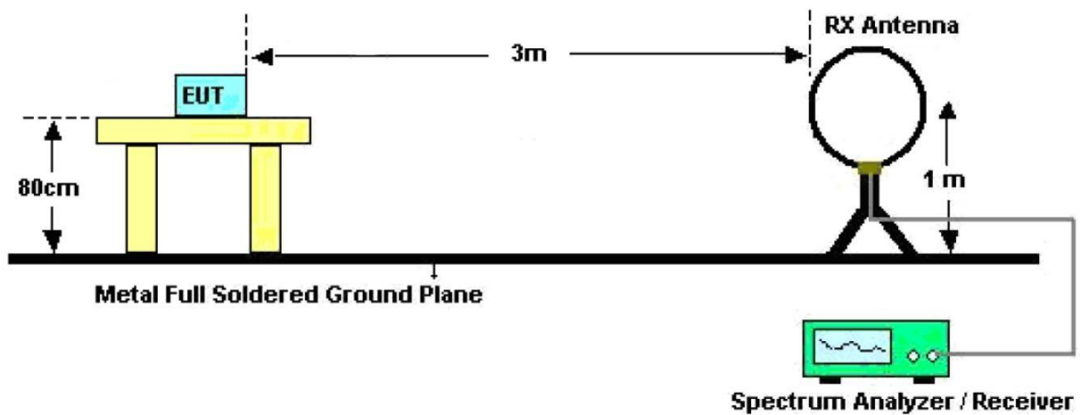
Figure 1. Below 30MHz
