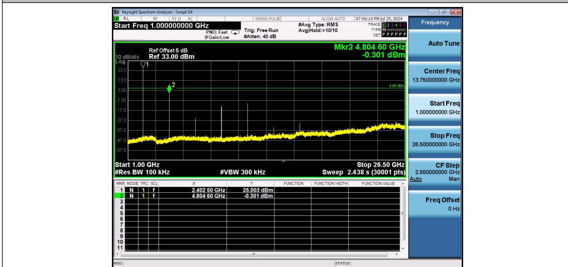
2.4G-Ant1-2402.4-1000~26500-PASS
