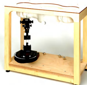
Photo of SAM Phantom
