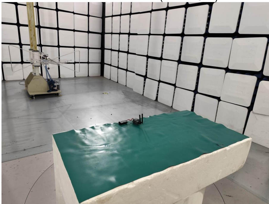
Radiation Emission Test (below 1GHz)
