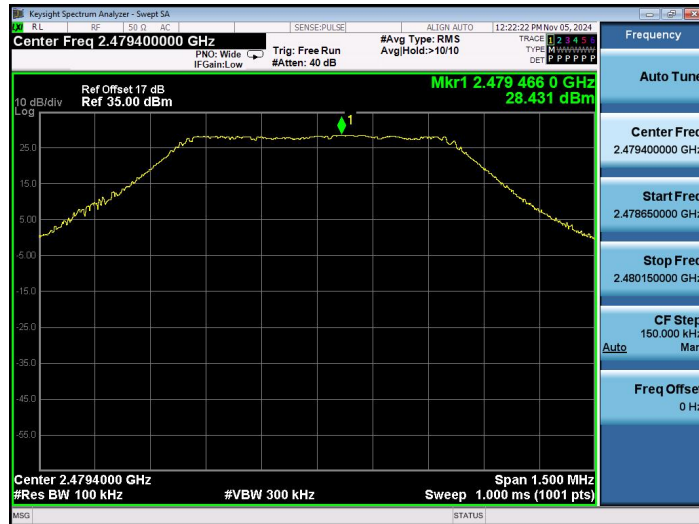
2.4G-Ant1-2479.4-0~Reference-PASS
