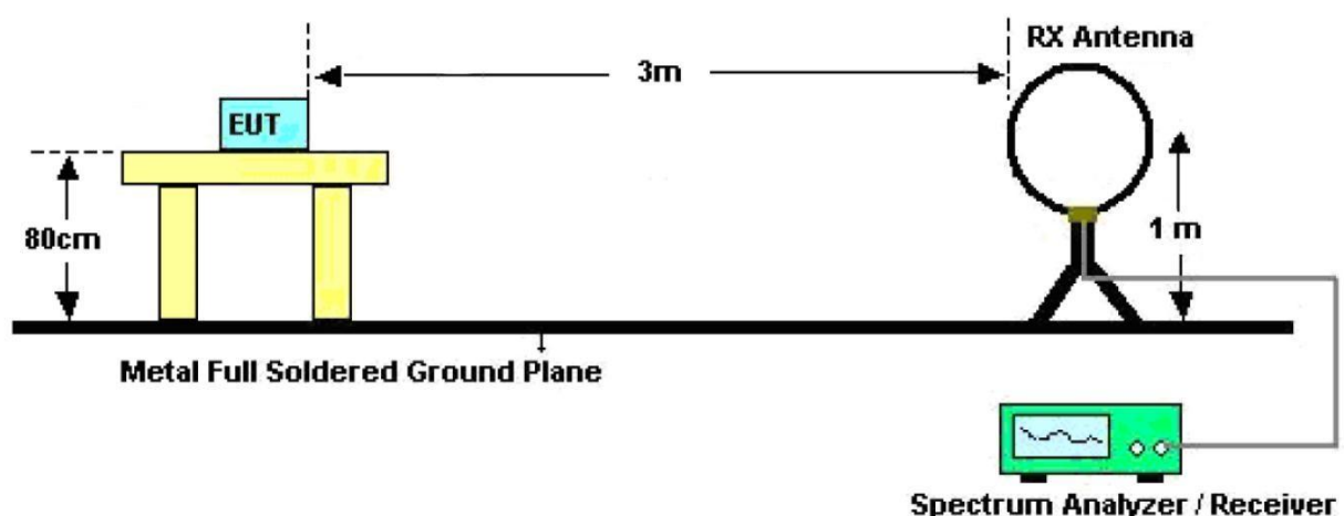
Figure 1. Below 30MHz
