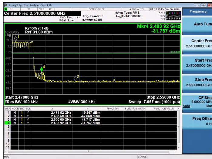
2.4G-Ant1-Hop_2479.4-PASS
