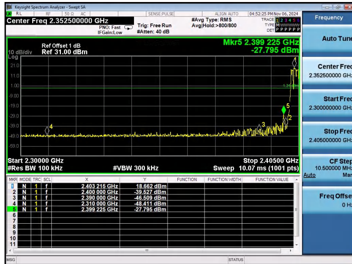
2.4G-Ant1-Hop_2402.4-PASS
