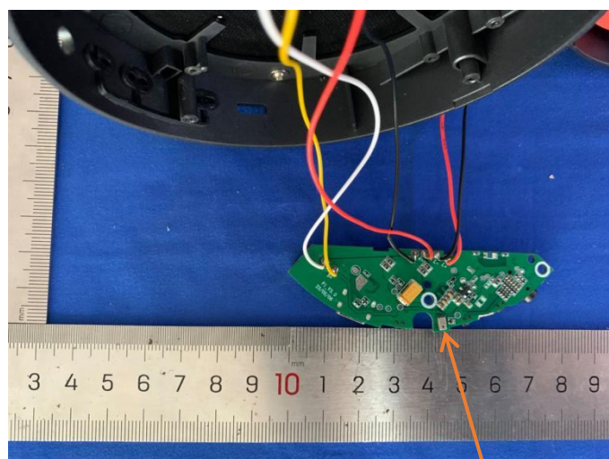
Chip Antenna
