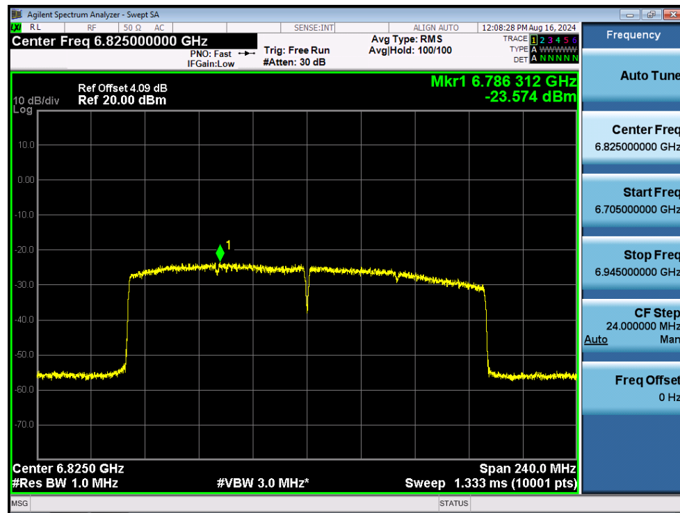
PSD NVNT ax160 6825MHz Ant3
