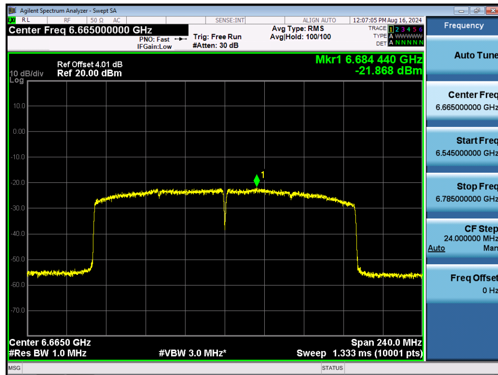
PSD NVNT ax160 6665MHz Ant3
