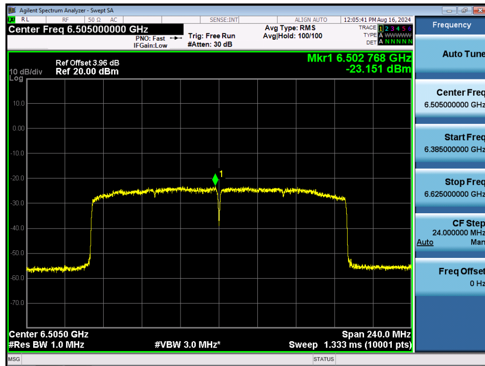
PSD NVNT ax160 6505MHz Ant3
