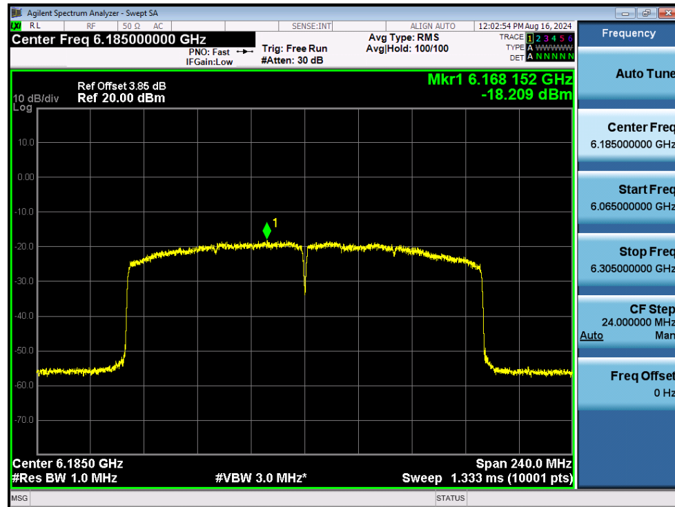
PSD NVNT ax160 6185MHz Ant3
