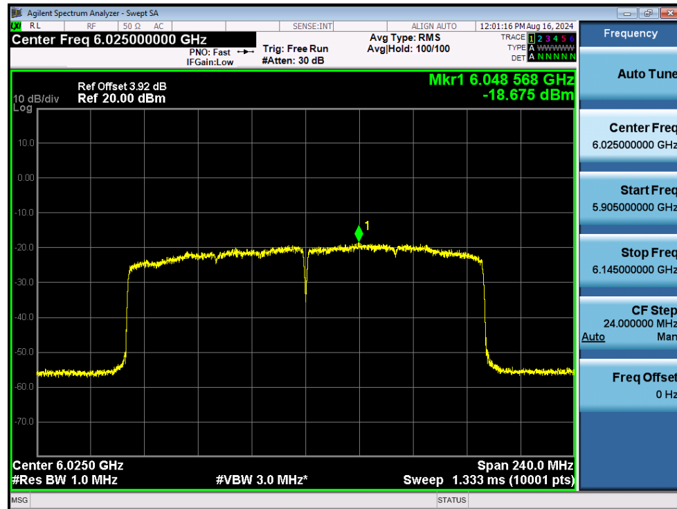
PSD NVNT ax160 6025MHz Ant3
