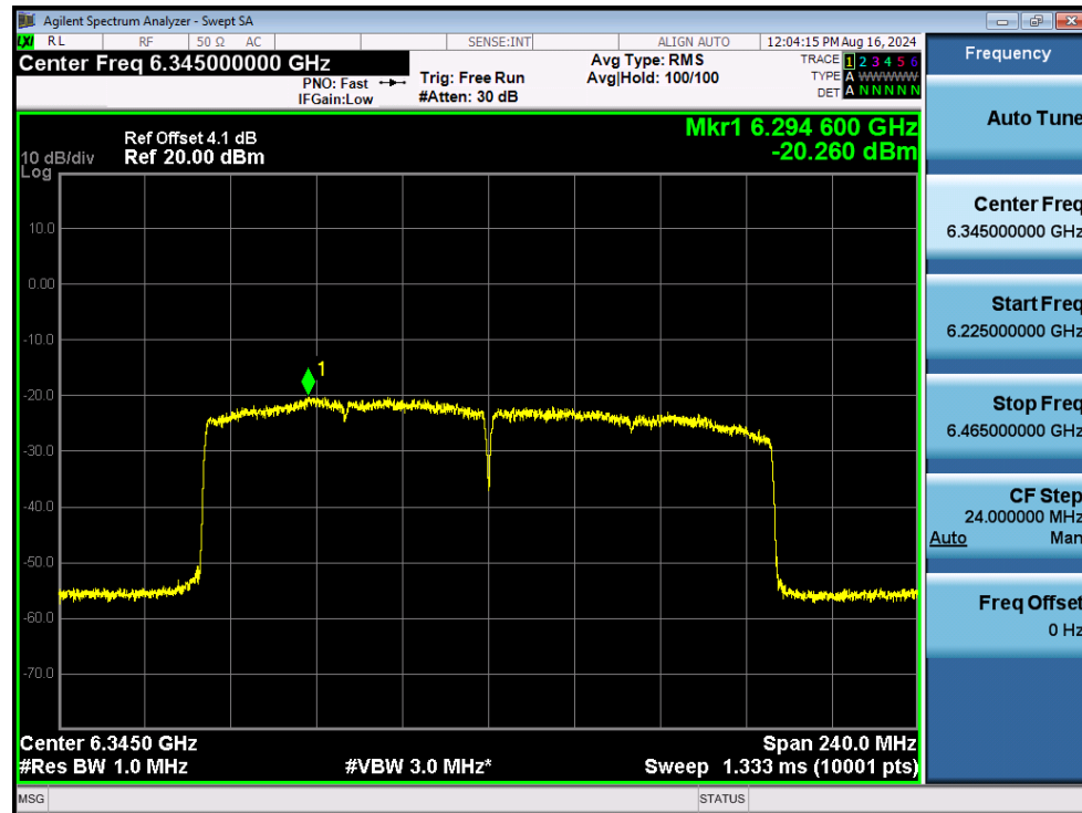
PSD NVNT ax160 6345MHz Ant3
