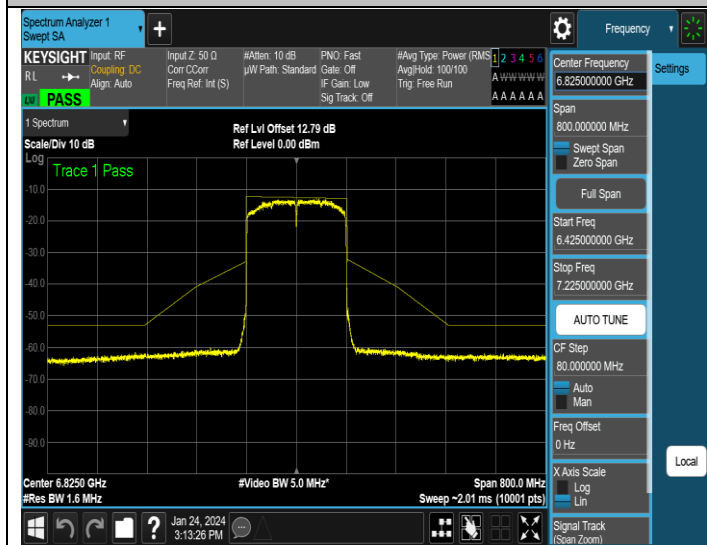
NTNV-11AX160MIMO-Ant1-6825-PASS
