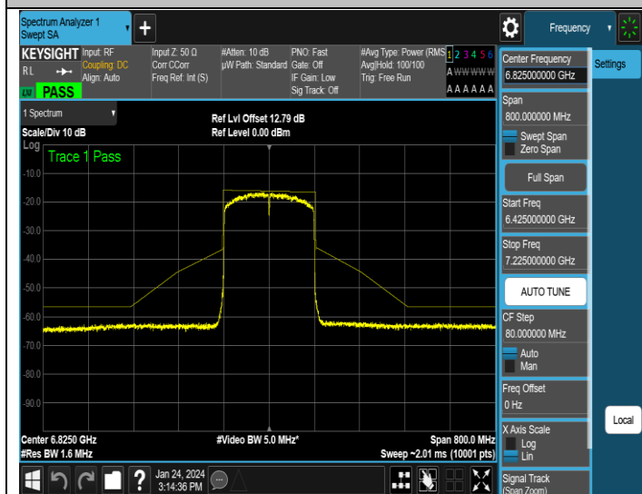
NTNV-11AX160MIMO-Ant3-6825-PASS
