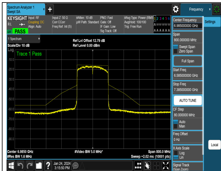
NTNV-11AX160MIMO-Ant1-6985-PASS
