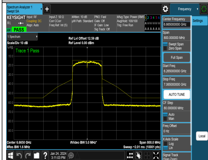
NTNV-11AX160MIMO-Ant1-6665-PASS
