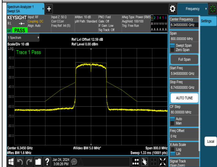
NTNV-11AX160MIMO-Ant1-6345-PASS
