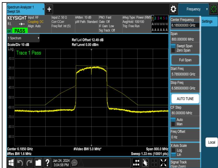
NTNV-11AX160MIMO-Ant3-6185-PASS
