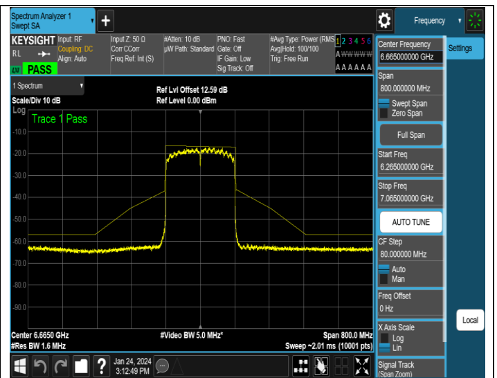
NTNV-11AX160MIMO-Ant4-6665-PASS
