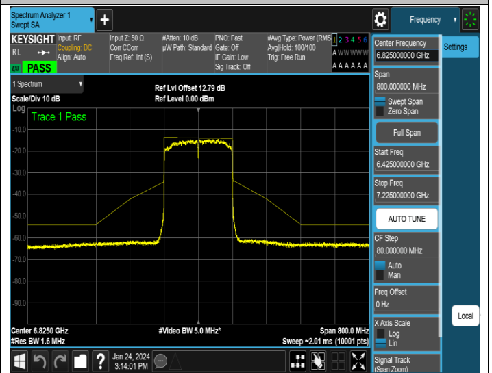
NTNV-11AX160MIMO-Ant2-6825-PASS
