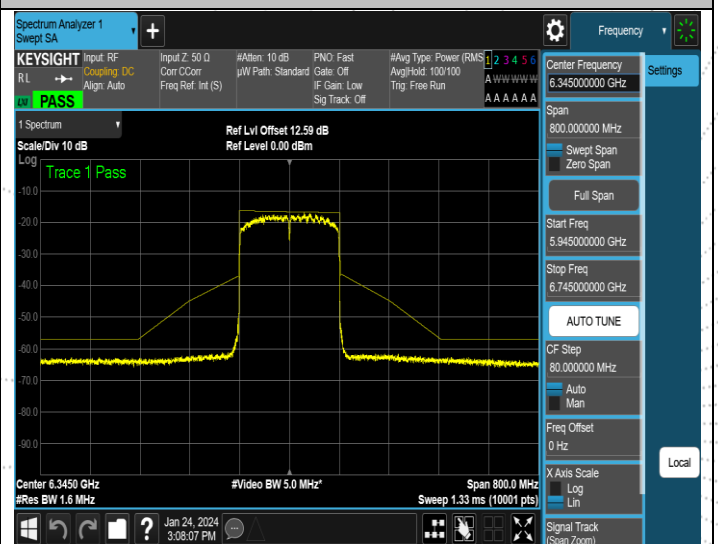
NTNV-11AX160MIMO-Ant4-6345-PASS
