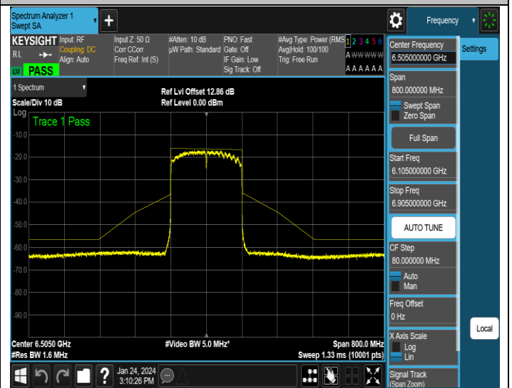
NTNV-11AX160MIMO-Ant4-6505-PASS
