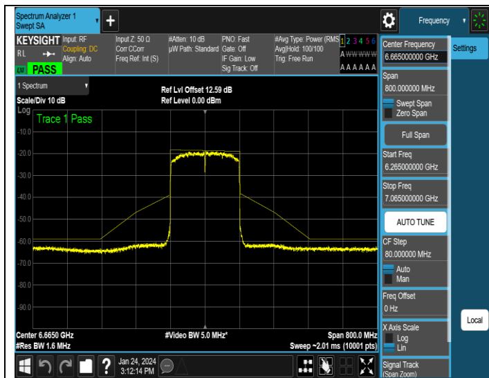
NTNV-11AX160MIMO-Ant3-6665-PASS
