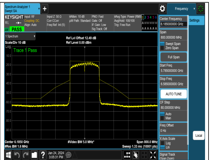
NTNV-11AX160MIMO-Ant4-6185-PASS
