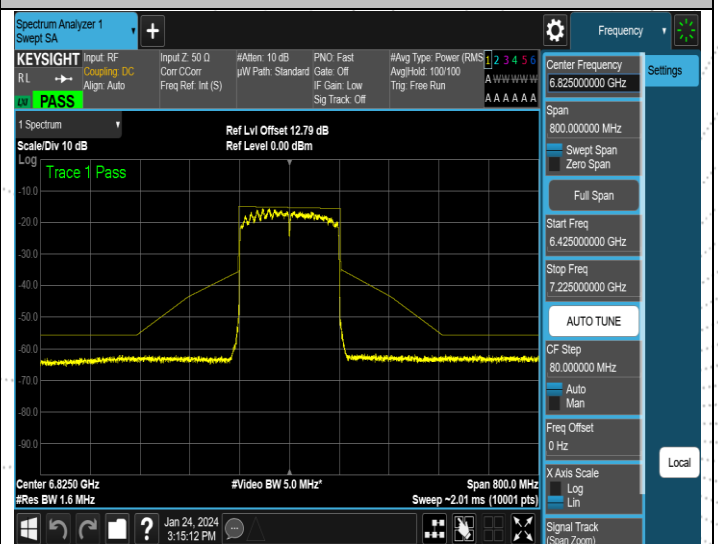
NTNV-11AX160MIMO-Ant4-6825-PASS
