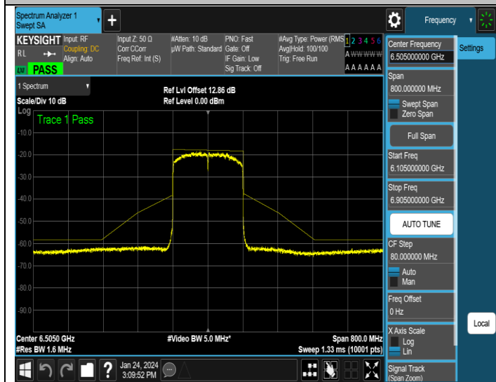
NTNV-11AX160MIMO-Ant3-6505-PASS
