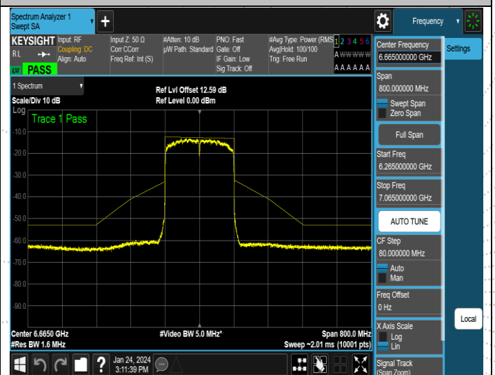
NTNV-11AX160MIMO-Ant2-6665-PASS
