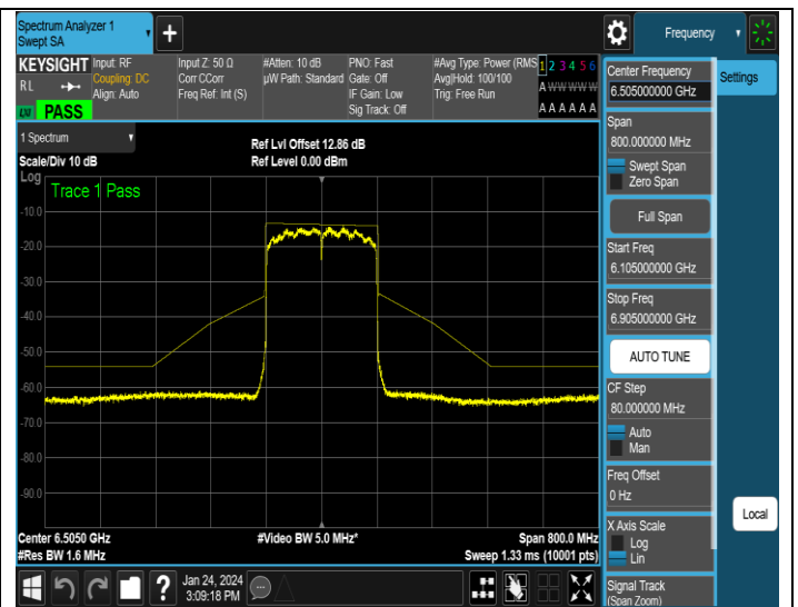
NTNV-11AX160MIMO-Ant2-6505-PASS
