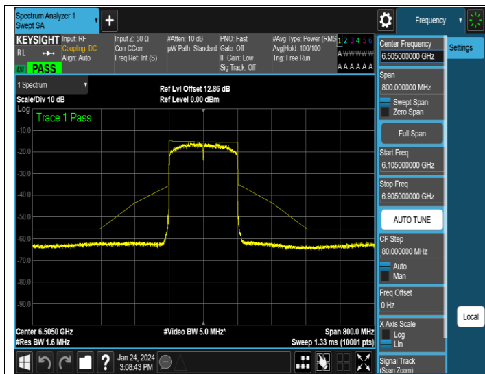
NTNV-11AX160MIMO-Ant1-6505-PASS
