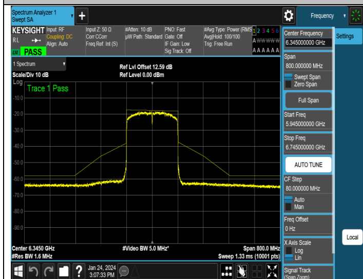
NTNV-11AX160MIMO-Ant3-6345-PASS
