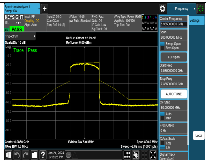
NTNV-11AX160MIMO-Ant2-6985-PASS
