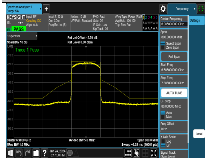
NTNV-11AX160MIMO-Ant3-6985-PASS
