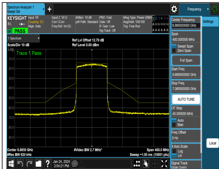
NTNV-11AX80MIMO-Ant1-6865-PASS
