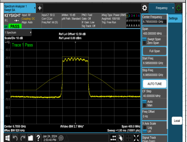
NTNV-11AX80MIMO-Ant4-6785-PASS
