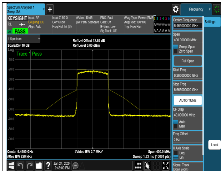
NTVN-11AX80MIMO-Ant3-6465-PASS
