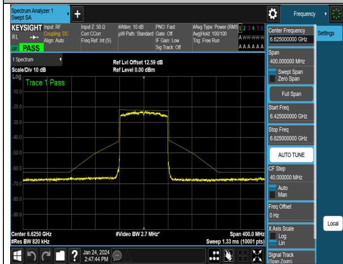
NTNV-11AX80MIMO-Ant3-6625-PASS
