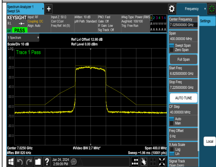
NTNV-11AX80MIMO-Ant1-7025-PASS
