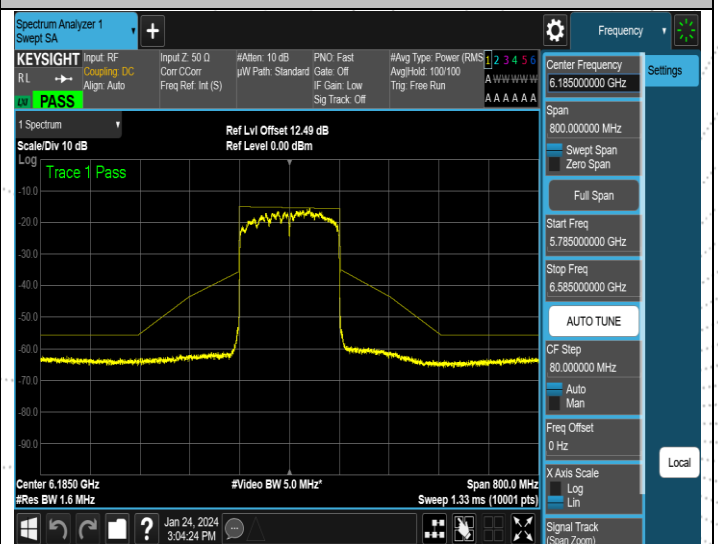
NTNV-11AX160MIMO-Ant2-6185-PASS
