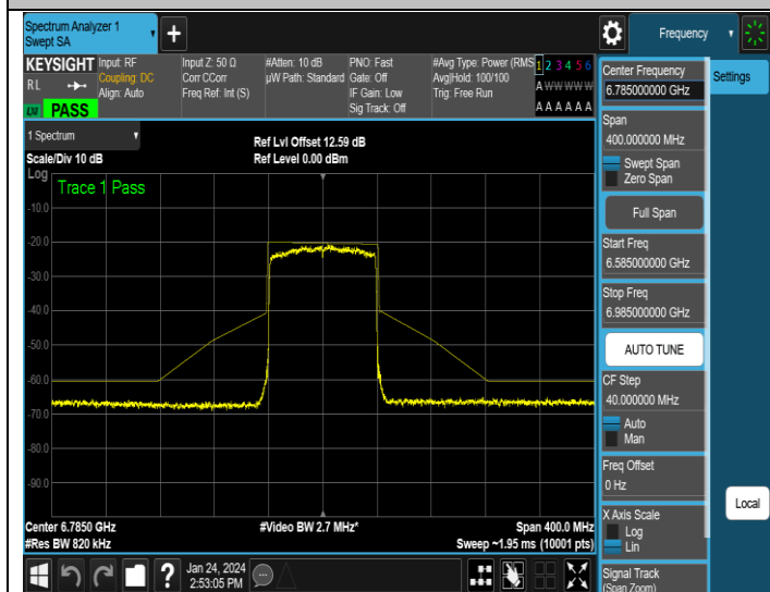
NTNV-11AX80MIMO-Ant3-6785-PASS
