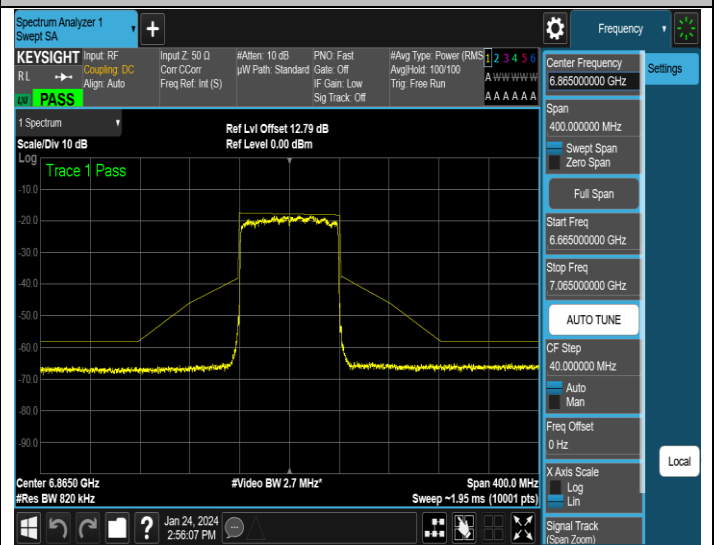
NTNV-11AX80MIMO-Ant4-6865-PASS
