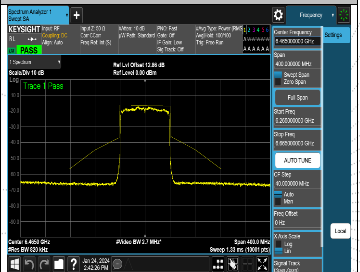
NTNV-11AX80MIMO-Ant2-6465-PASS
