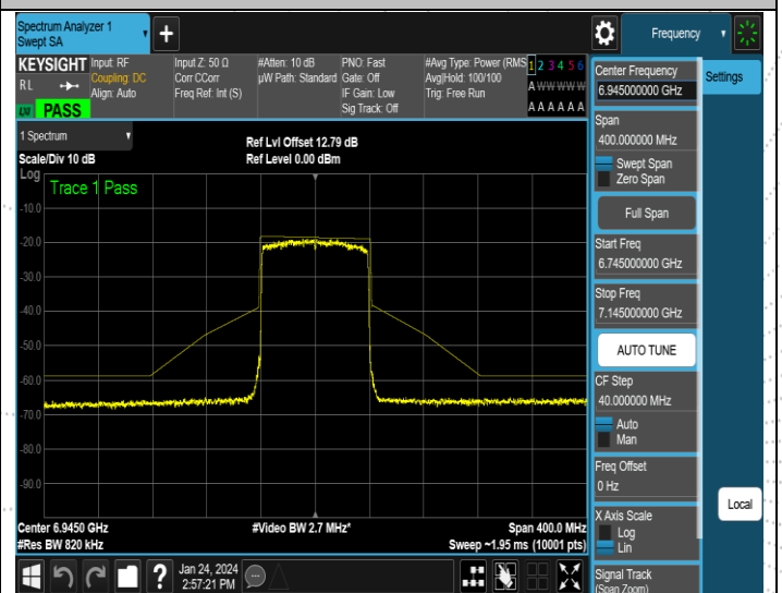
NTNV-11AX80MIMO-Ant2-6945-PASS
