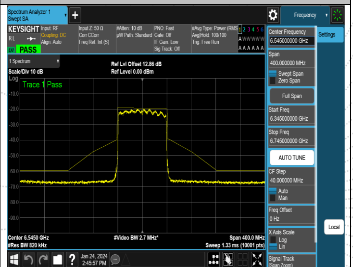
NTVN-11AX80MIMO-Ant4-6545-PASS
