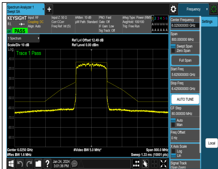
NTNV-11AX160MIMO-Ant1-6025-PASS
