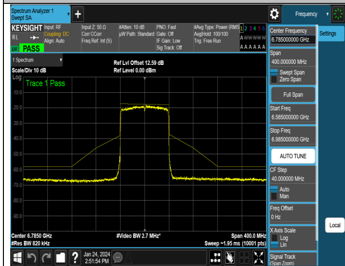
NTNV-11AX80MIMO-Ant1-6785-PASS
