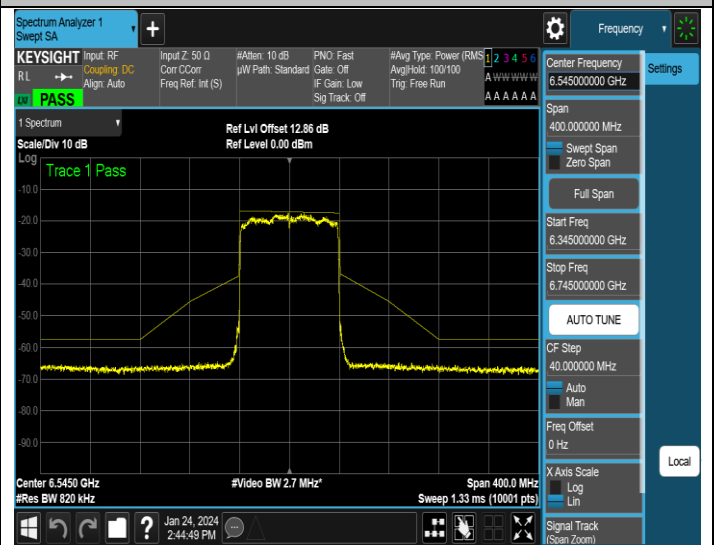
NTVN-11AX80MIMO-Ant2-6545-PASS
