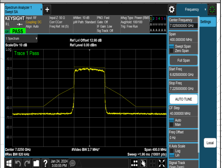
NTNV-11AX80MIMO-Ant4-7025-PASS
