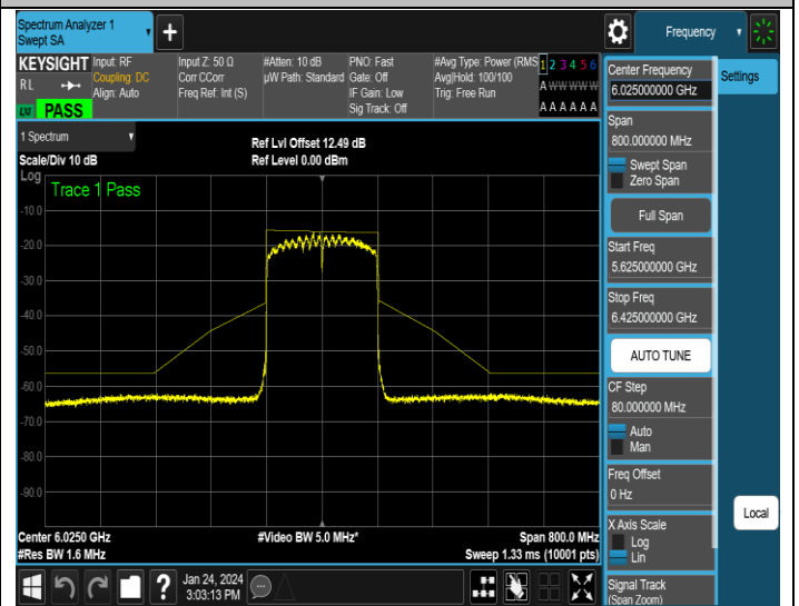
NTNV-11AX160MIMO-Ant4-6025-PASS
