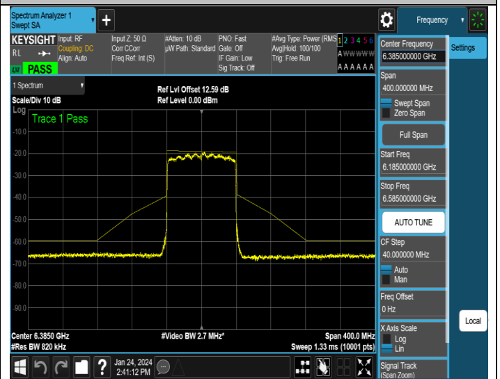
NTNV-11AX80MIMO-Ant4-6385-PASS
