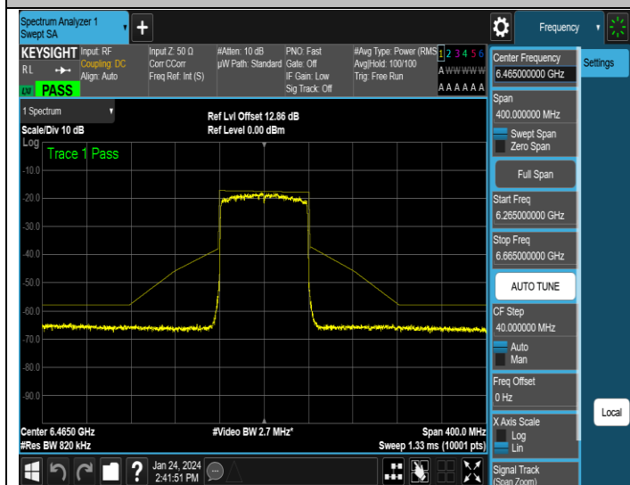
NTNV-11AX80MIMO-Ant1-6465-PASS
