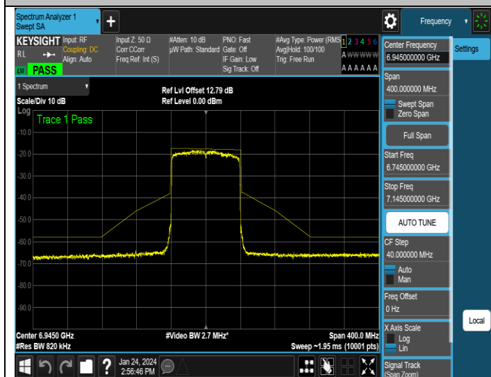
NTNV-11AX80MIMO-Ant1-6945-PASS
