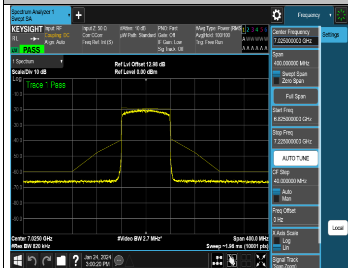
NTNV-11AX80MIMO-Ant3-7025-PASS
