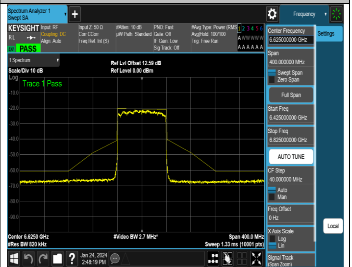
NTNV-11AX80MIMO-Ant4-6625-PASS
