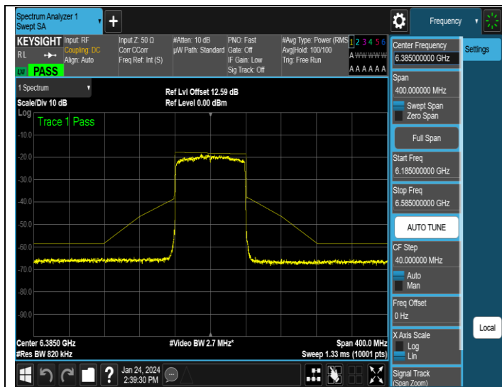
NTNV-11AX80MIMO-Ant1-6385-PASS
