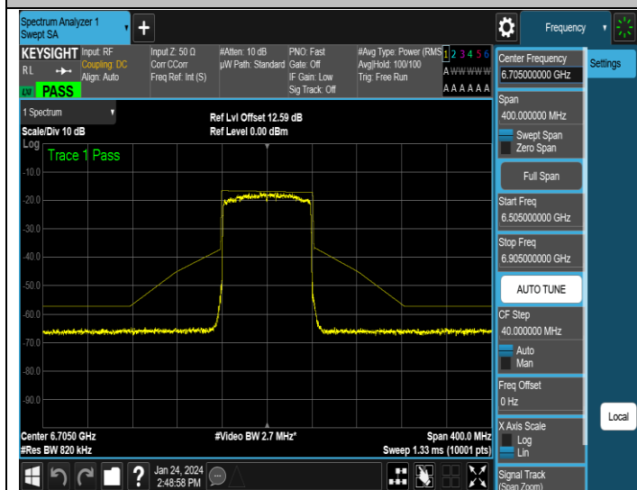
NTNV-11AX80MIMO-Ant1-6705-PASS
