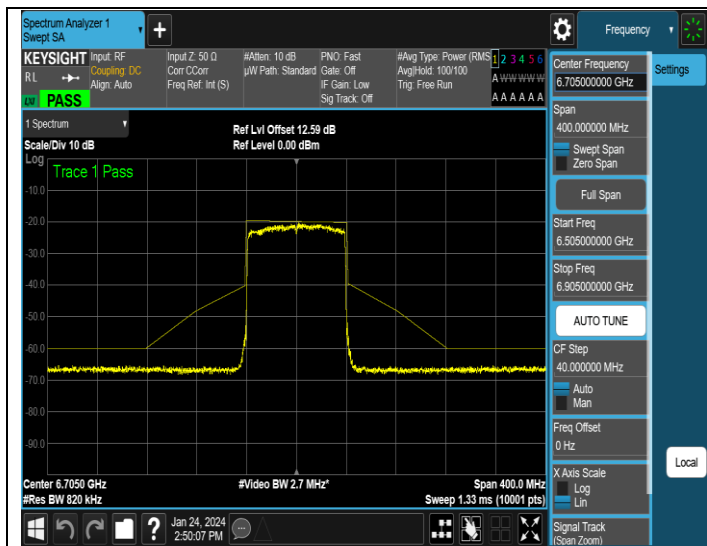
NTNV-11AX80MIMO-Ant3-6705-PASS
