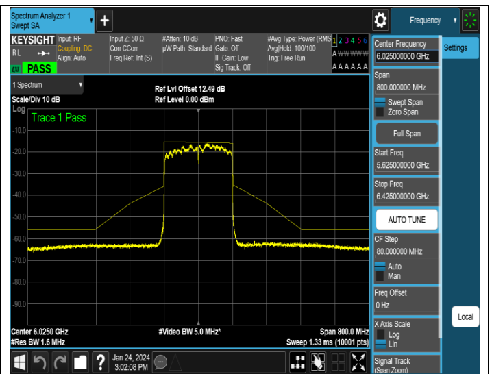
NTNV-11AX160MIMO-Ant2-6025-PASS
