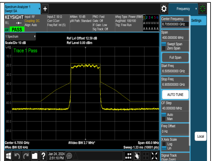
NTNV-11AX80MIMO-Ant4-6705-PASS
