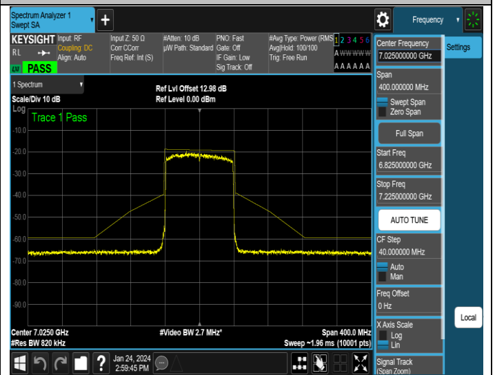
NTNV-11AX80MIMO-Ant2-7025-PASS
