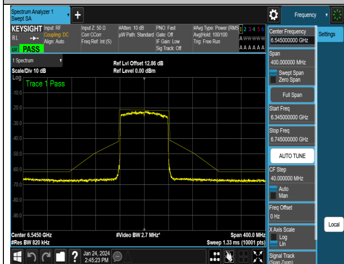
NTVN-11AX80MIMO-Ant3-6545-PASS
