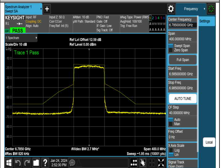
NTNV-11AX80MIMO-Ant2-6785-PASS
