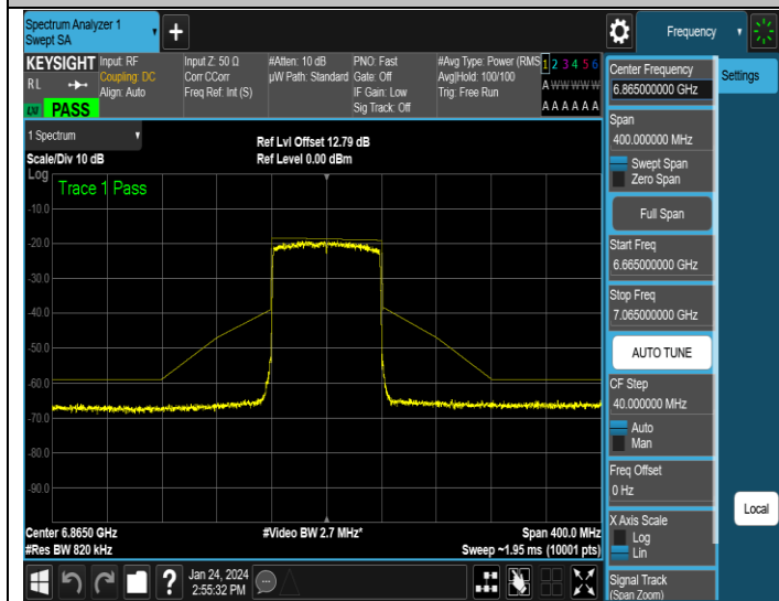
NTNV-11AX80MIMO-Ant3-6865-PASS
