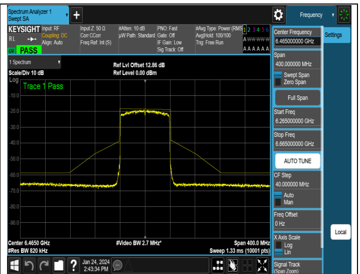
NTVN-11AX80MIMO-Ant4-6465-PASS
