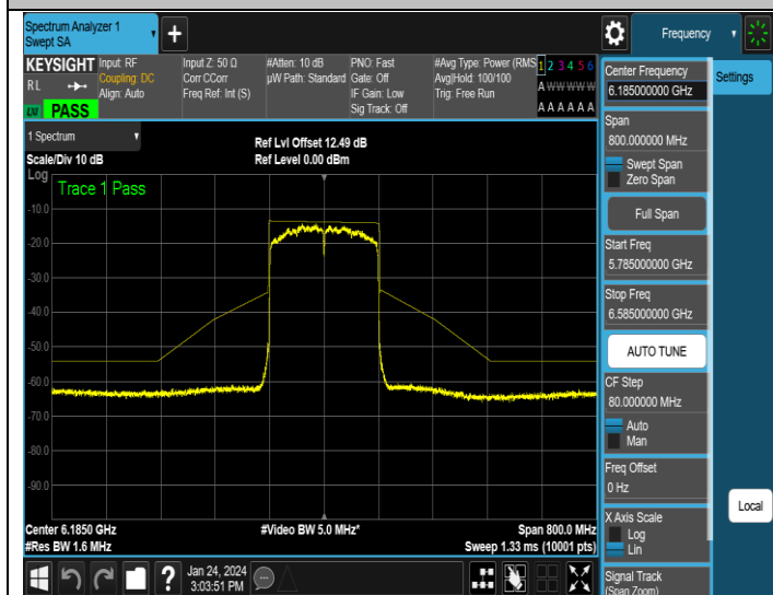
NTNV-11AX160MIMO-Ant1-6185-PASS
