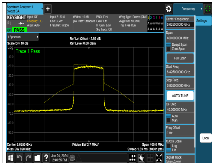
NTNV-11AX80MIMO-Ant1-6625-PASS
