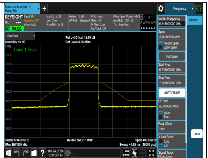
NTNV-11AX80MIMO-Ant4-6945-PASS
