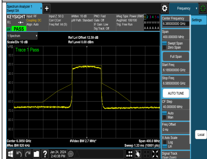
NTNV-11AX80MIMO-Ant3-6385-PASS
