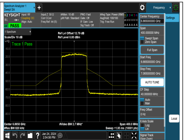
NTNV-11AX80MIMO-Ant2-6865-PASS
