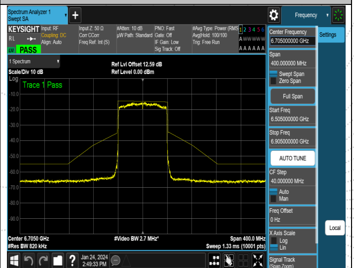
NTNV-11AX80MIMO-Ant2-6705-PASS
