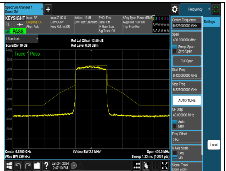
NTNV-11AX80MIMO-Ant2-6625-PASS
