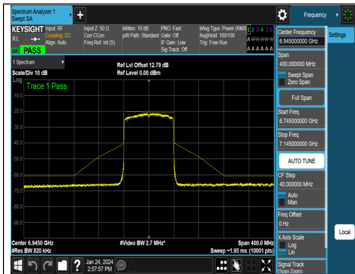
NTNV-11AX80MIMO-Ant3-6945-PASS
