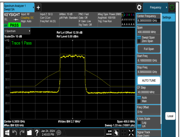
NTNV-11AX80MIMO-Ant2-6385-PASS
