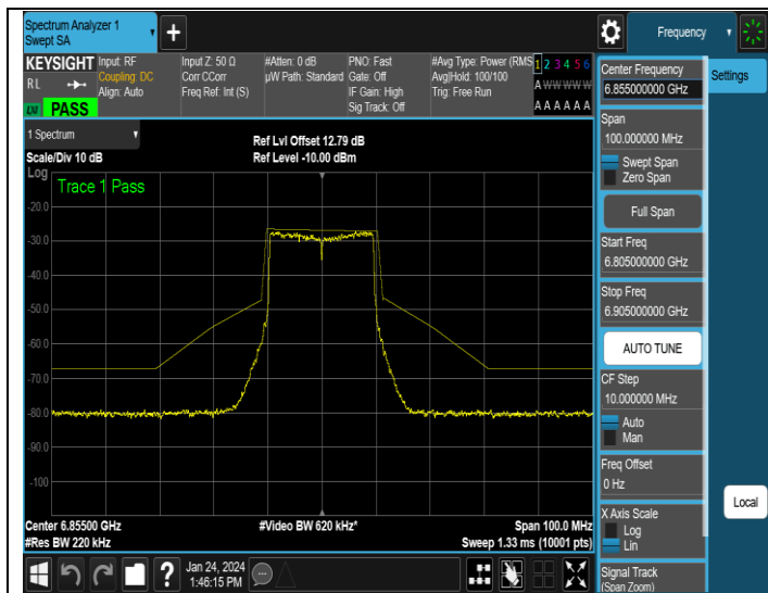
NTNV-11AX20MIMO-Ant3-6855-PASS
