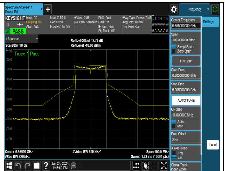
NTNV-11AX20MIMO-Ant4-6855-PASS
