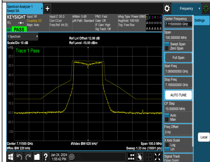
NTNV-11AX20MIMO-Ant1-7115-PASS
