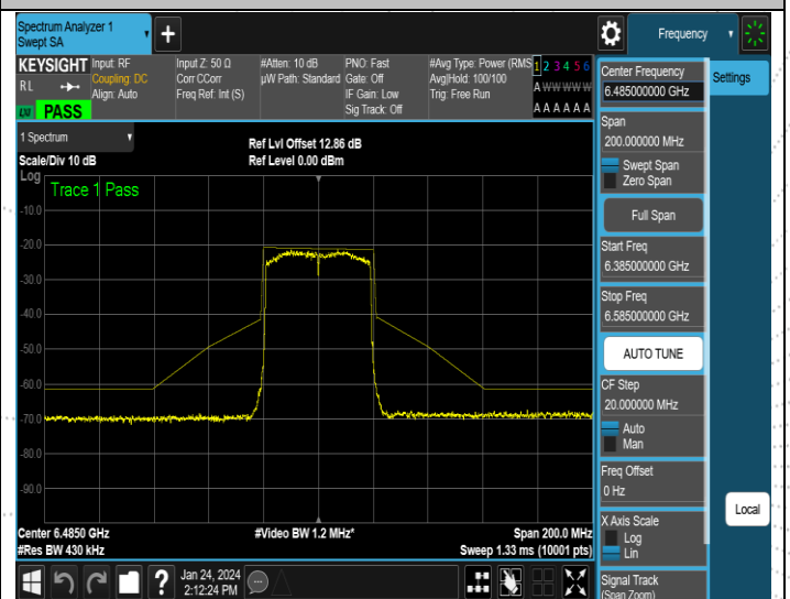
NTNV-11AX40MIMO-Ant2-6485-PASS
