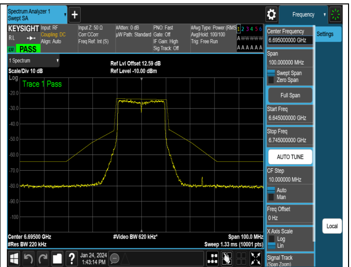
NTNV-11AX20MIMO-Ant2-6695-PASS
