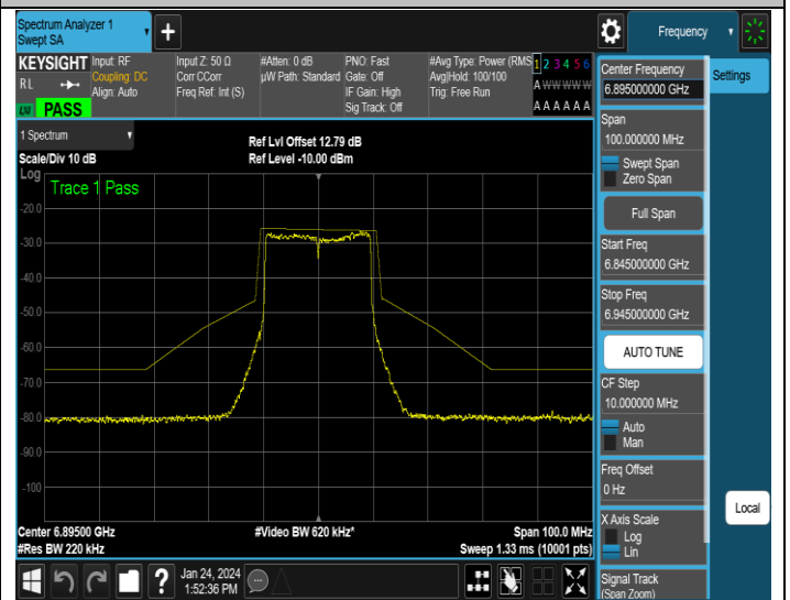
NTNV-11AX20MIMO-Ant4-6895-PASS
