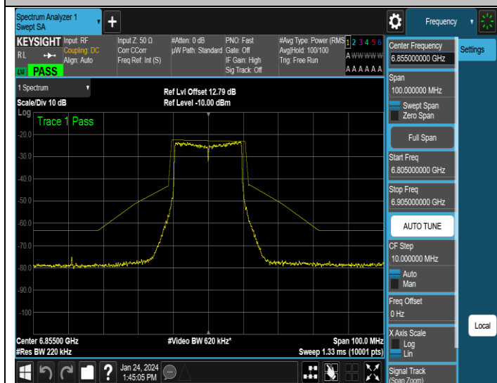
NTNV-11AX20MIMO-Ant1-6855-PASS
