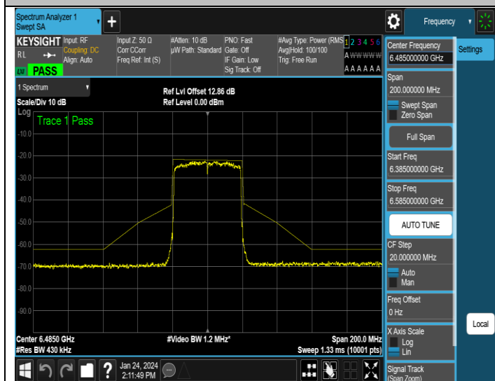
NTNV-11AX40MIMO-Ant1-6485-PASS
