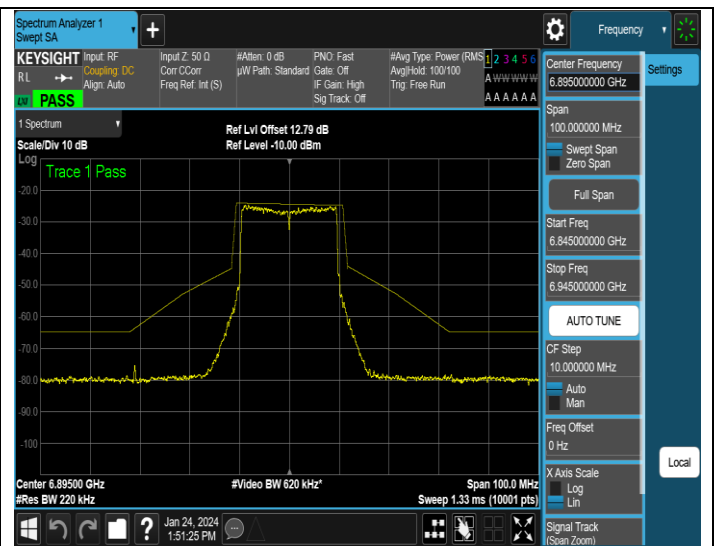
NTNV-11AX20MIMO-Ant2-6895-PASS
