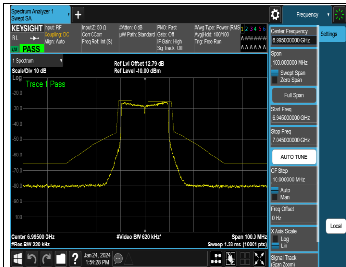
NTNV-11AX20MIMO-Ant3-6995-PASS
