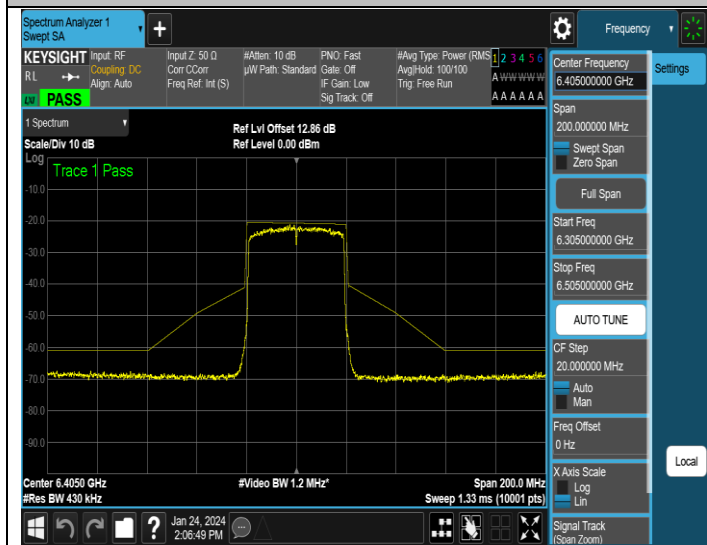
NTNV-11AX40MIMO-Ant1-6405-PASS
