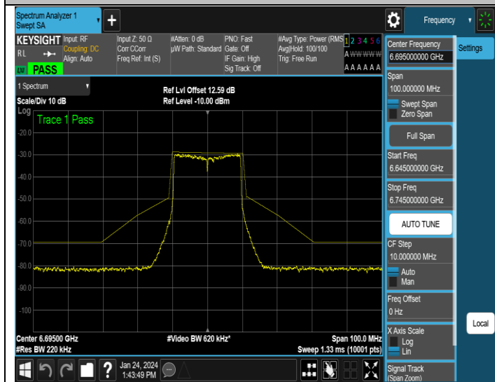
NTNV-11AX20MIMO-Ant3-6695-PASS
