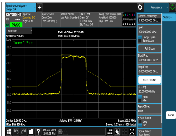
NTNV-11AX40MIMO-Ant1-5965-PASS
