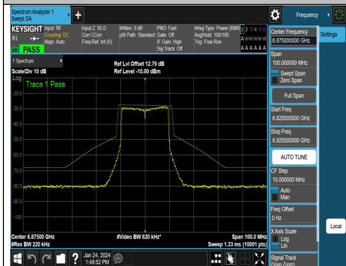
NTNV-11AX20MIMO-Ant3-6875-PASS
