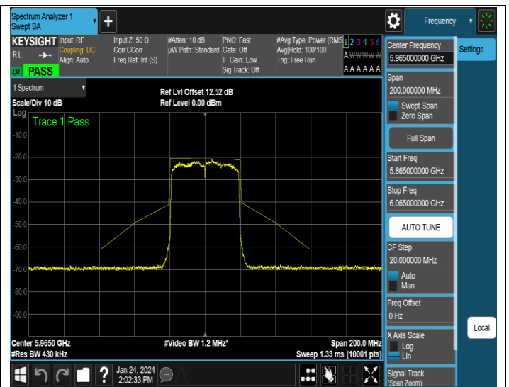
NTNV-11AX40MIMO-Ant2-5965-PASS
