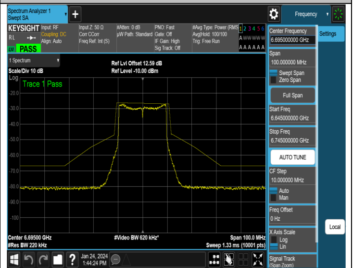
NTNV-11AX20MIMO-Ant4-6695-PASS
