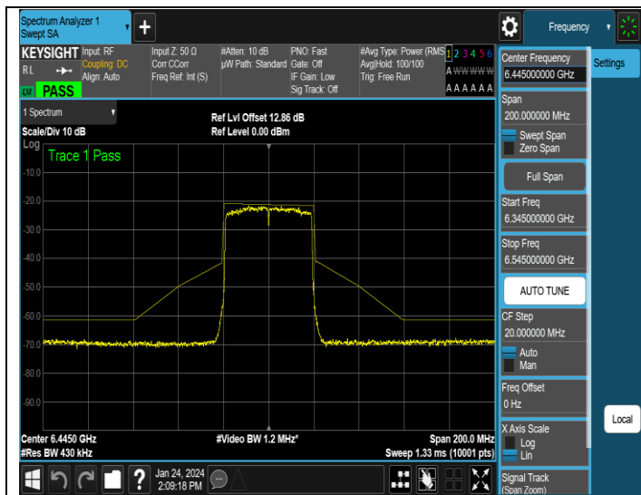
NTNV-11AX40MIMO-Ant1-6445-PASS
