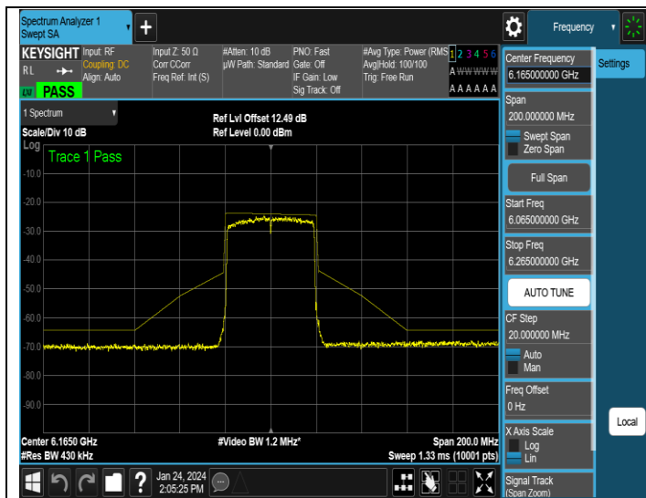
NTNV-11AX40MIMO-Ant3-6165-PASS
