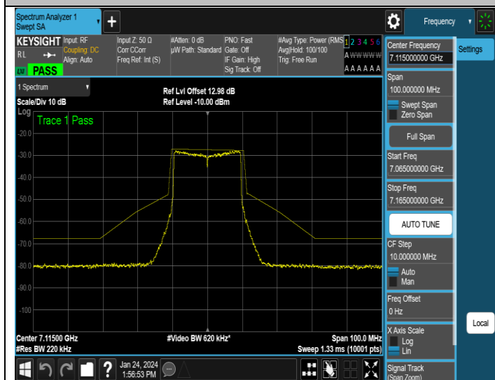
NTNV-11AX20MIMO-Ant3-7115-PASS
