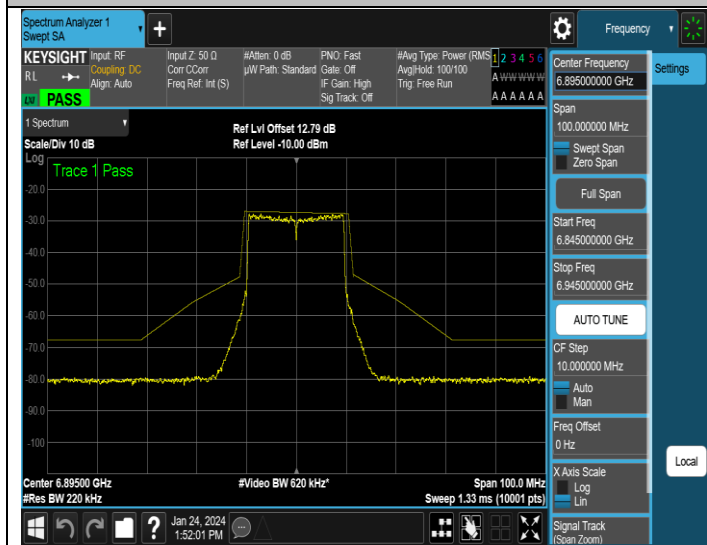
NTNV-11AX20MIMO-Ant3-6895-PASS
