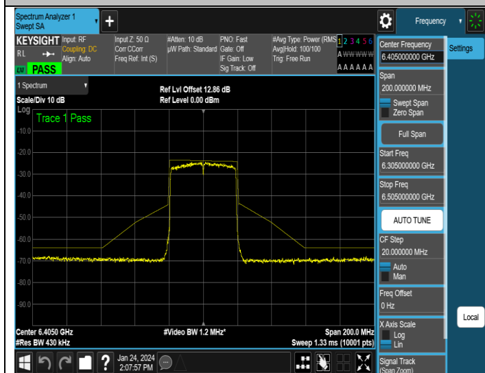
NTNV-11AX40MIMO-Ant3-6405-PASS
