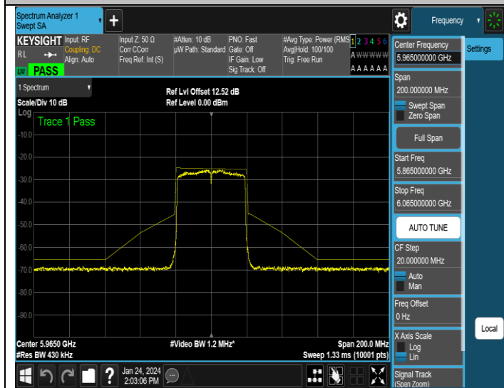
NTNV-11AX40MIMO-Ant3-5965-PASS
