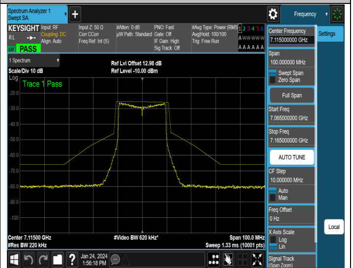
NTNV-11AX20MIMO-Ant2-7115-PASS
