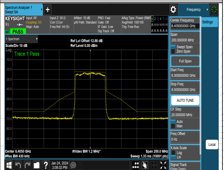
NTNV-11AX40MIMO-Ant4-6405-PASS
