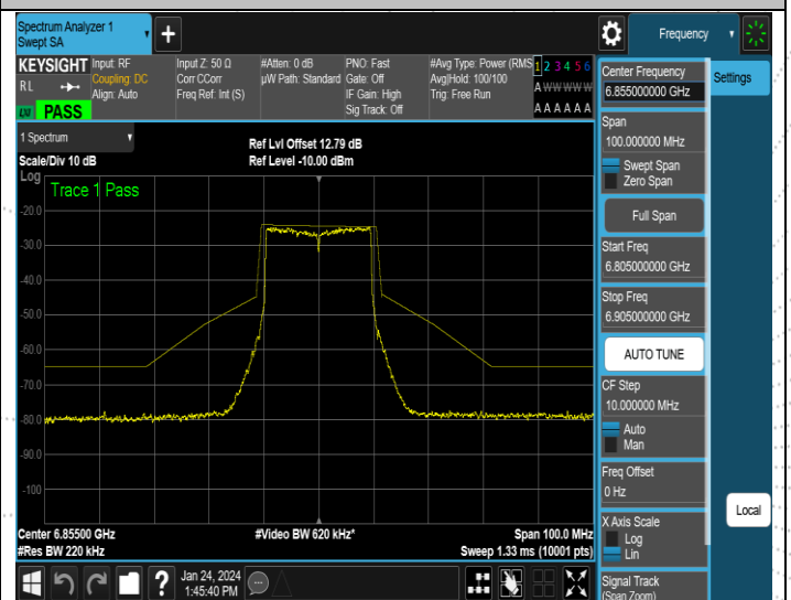
NTNV-11AX20MIMO-Ant2-6855-PASS
