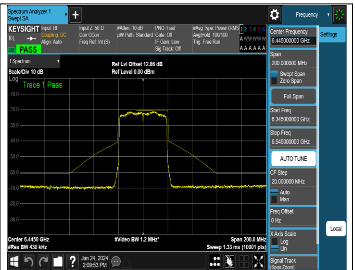
NTNV-11AX40MIMO-Ant2-6445-PASS
