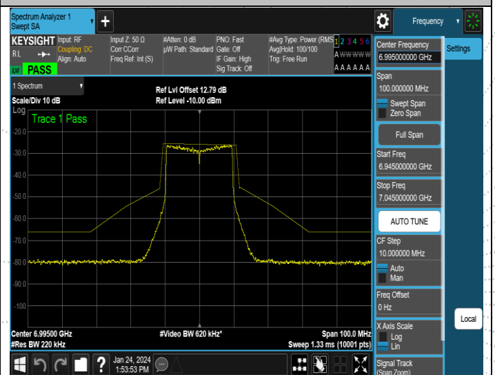
NTNV-11AX20MIMO-Ant2-6995-PASS
