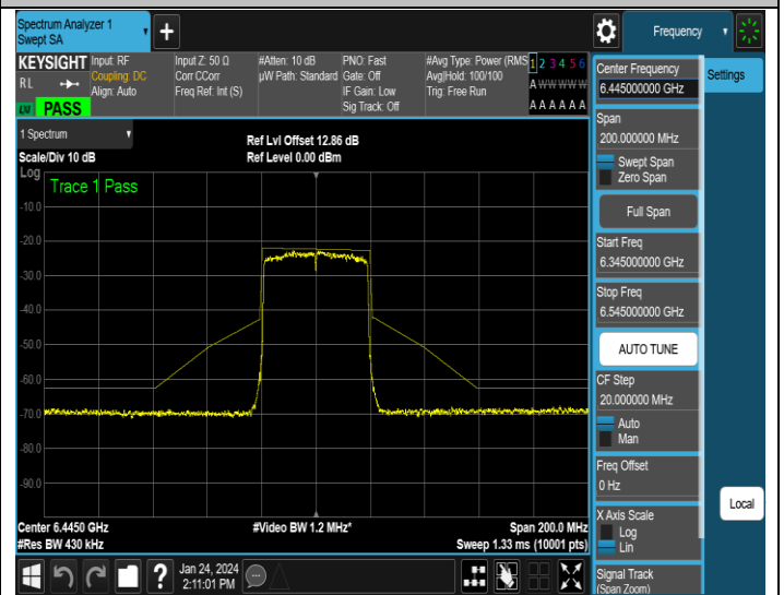
NTNV-11AX40MIMO-Ant4-6445-PASS
