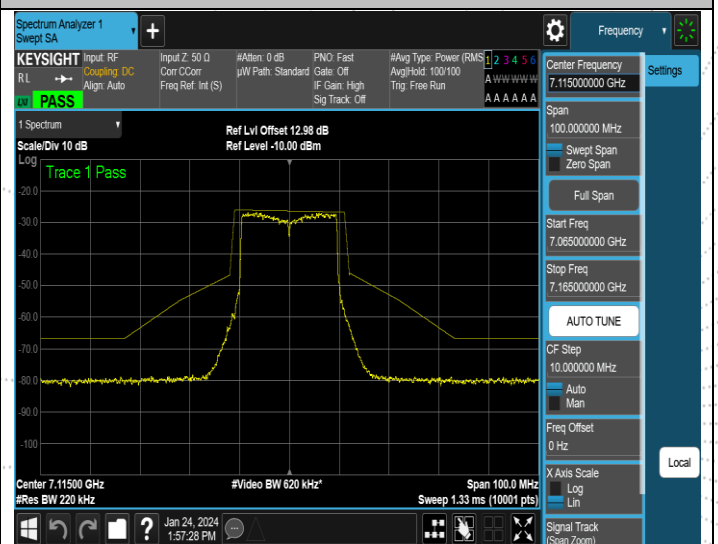
NTNV-11AX20MIMO-Ant4-7115-PASS
