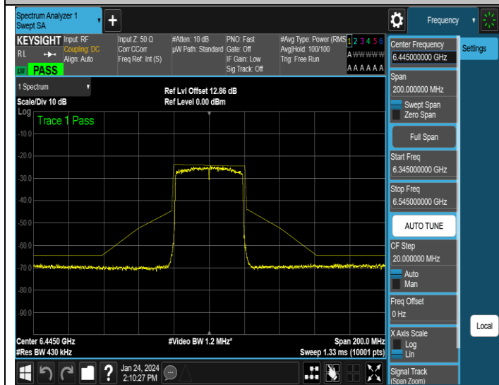
NTNV-11AX40MIMO-Ant3-6445-PASS
