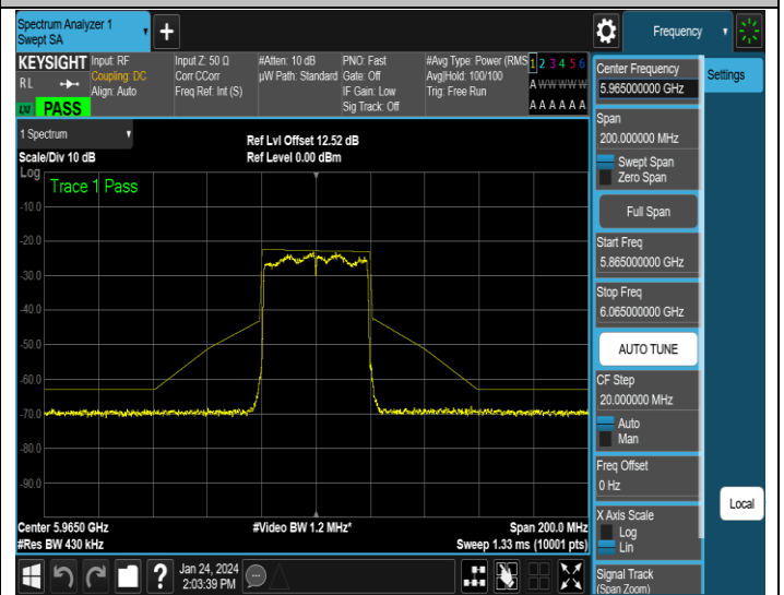
NTNV-11AX40MIMO-Ant4-5965-PASS
