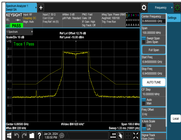
NTNV-11AX20MIMO-Ant1-6895-PASS
