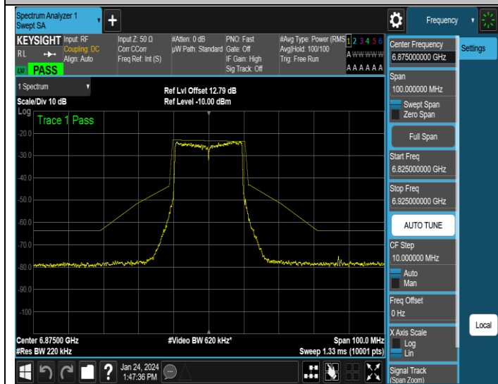
NTNV-11AX20MIMO-Ant1-6875-PASS
