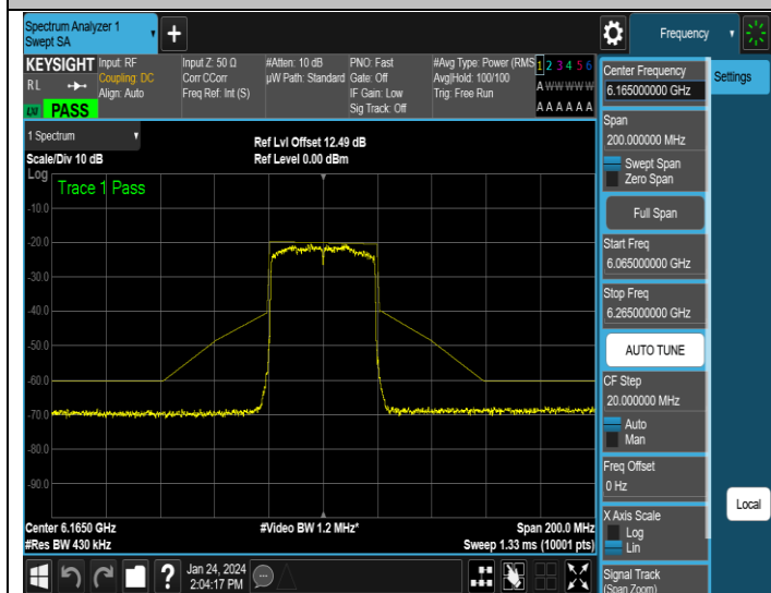
NTNV-11AX40MIMO-Ant1-6165-PASS
