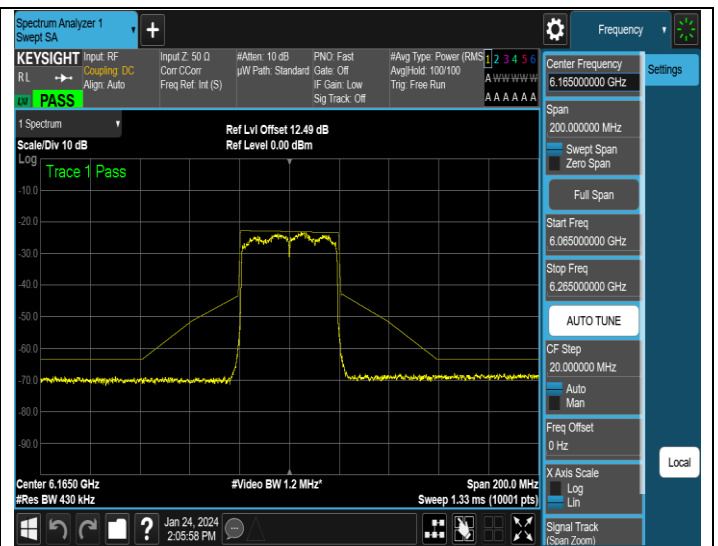
NTNV-11AX40MIMO-Ant4-6165-PASS
