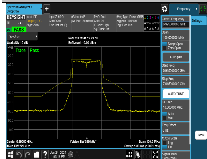
NTNV-11AX20MIMO-Ant1-6995-PASS
