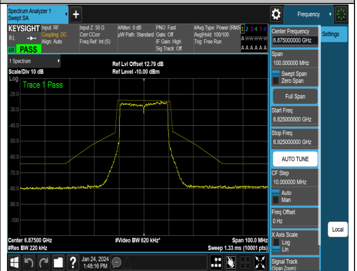
NTNV-11AX20MIMO-Ant2-6875-PASS
