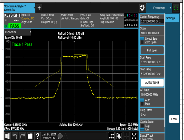
NTNV-11AX20MIMO-Ant4-6875-PASS
