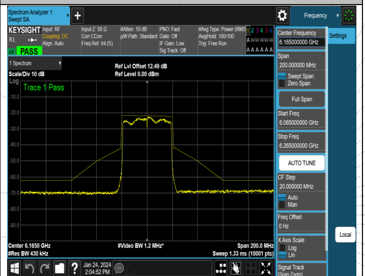
NTNV-11AX40MIMO-Ant2-6165-PASS
