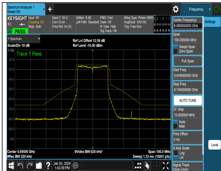
NTNV-11AX20MIMO-Ant1-6695-PASS
