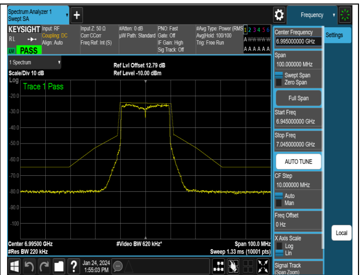
NTNV-11AX20MIMO-Ant4-6995-PASS
