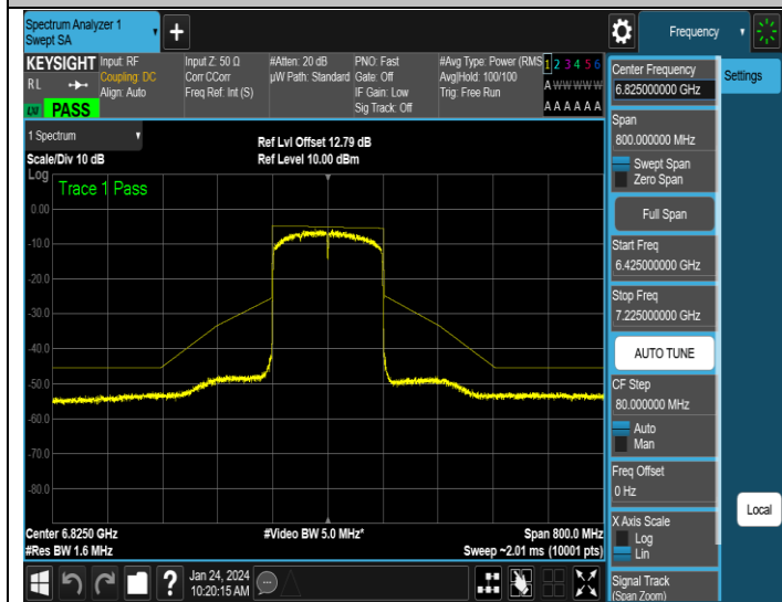
NTNV-11AX160SISO-Ant3-6825-PASS
