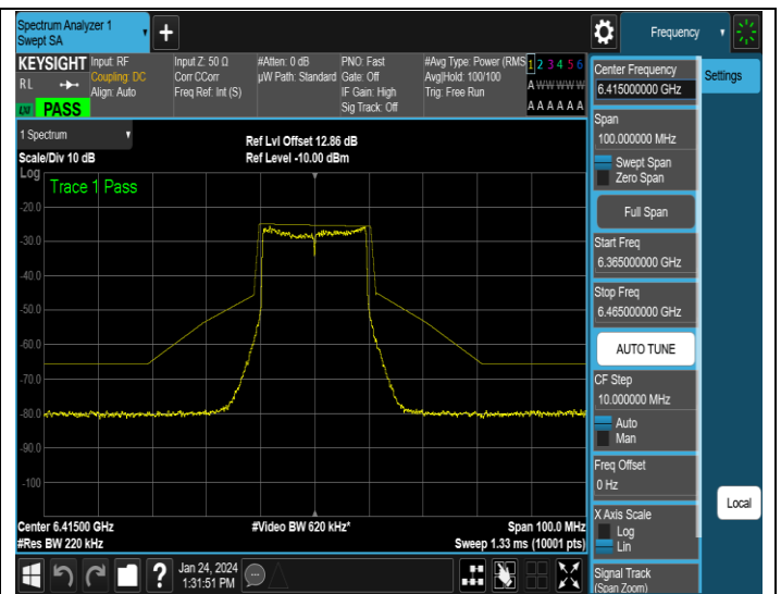
NTNV-11AX20MIMO-Ant4-6415-PASS
