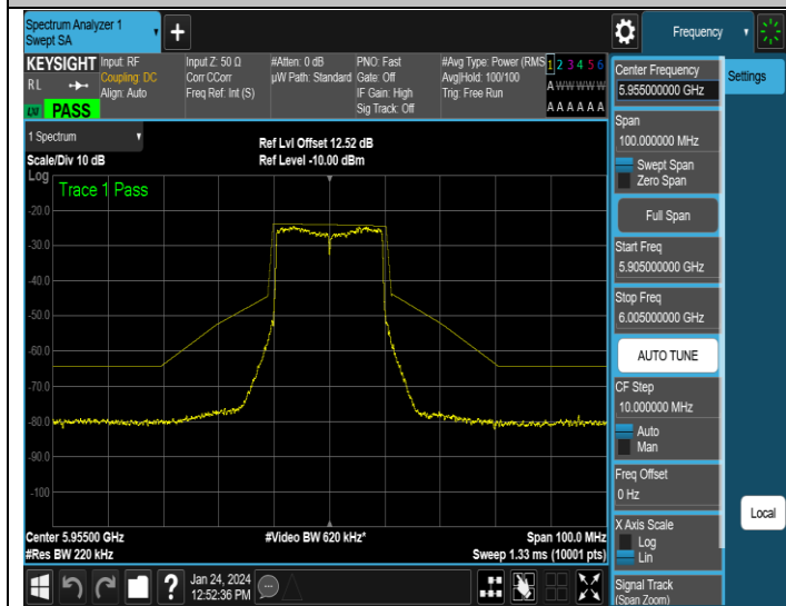
NTNV-11AX20MIMO-Ant1-5955-PASS
