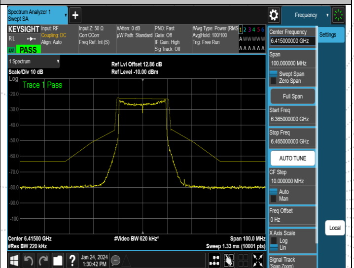
NTNV-11AX20MIMO-Ant2-6415-PASS
