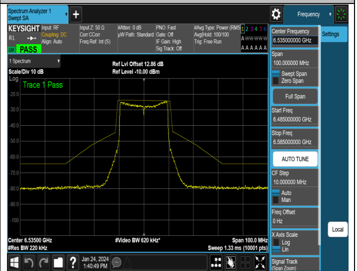
NTNV-11AX20MIMO-Ant2-6535-PASS
