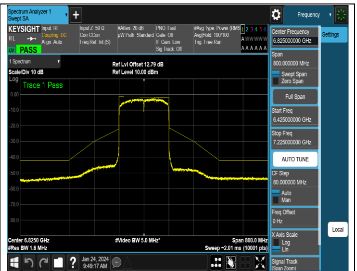
NTNV-11AX160SISO-Ant2-6825-PASS
