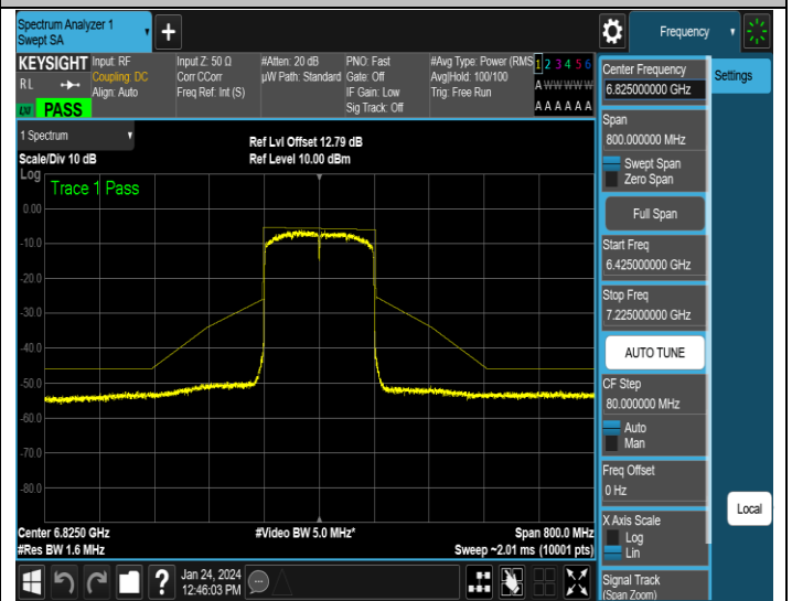
NTNV-11AX160SISO-Ant4-6825-PASS
