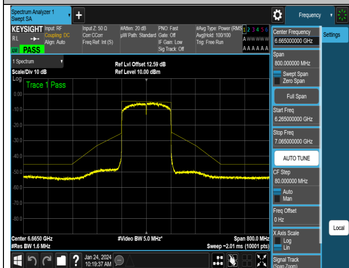
NTNV-11AX160SISO-Ant3-6665-PASS
