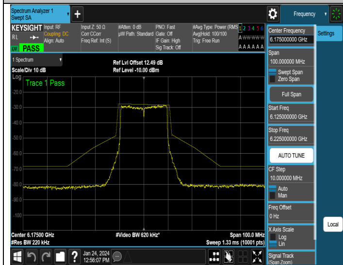
NTNV-11AX20MIMO-Ant3-6175-PASS
