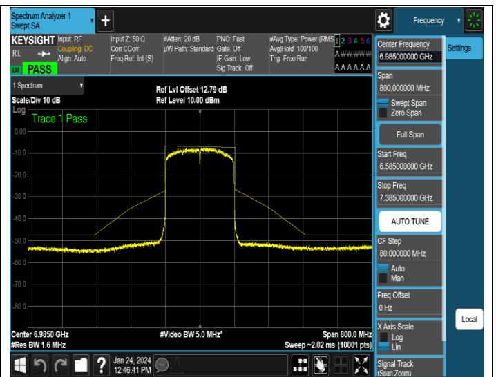
NTNV-11AX160SISO-Ant4-6985-PASS
