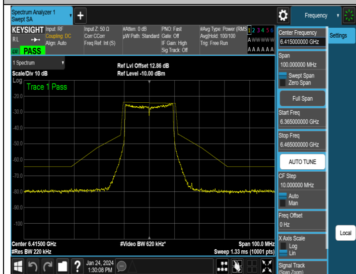
NTNV-11AX20MIMO-Ant1-6415-PASS
