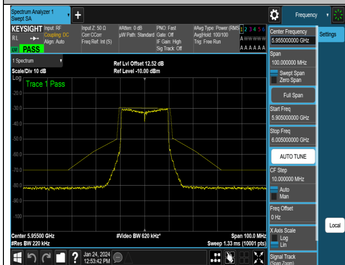
NTNV-11AX20MIMO-Ant3-5955-PASS
