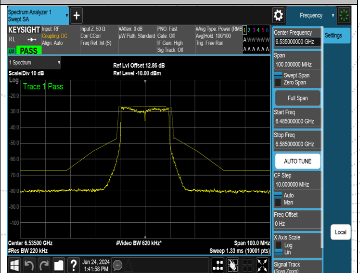
NTNV-11AX20MIMO-Ant4-6535-PASS
