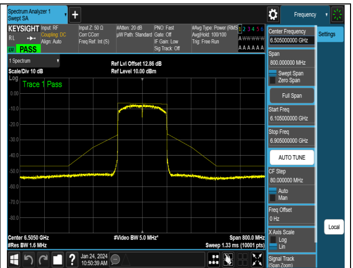
NTNV-11AX160SISO-Ant4-6505-PASS
