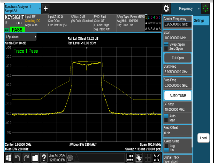
NTNV-11AX20MIMO-Ant2-5955-PASS
