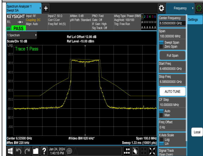
NTNV-11AX20MIMO-Ant1-6535-PASS
