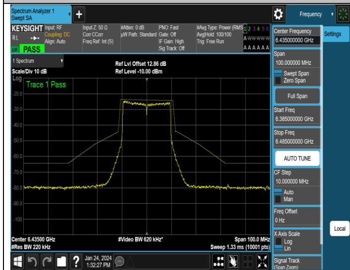
NTNV-11AX20MIMO-Ant1-6435-PASS
