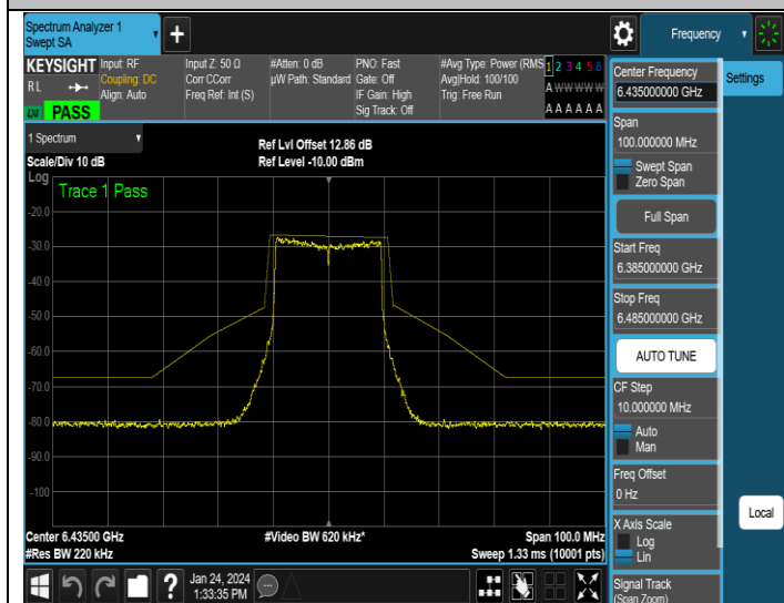
NTNV-11AX20MIMO-Ant3-6435-PASS
