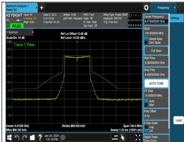
NTNV-11AX20MIMO-Ant3-6415-PASS
