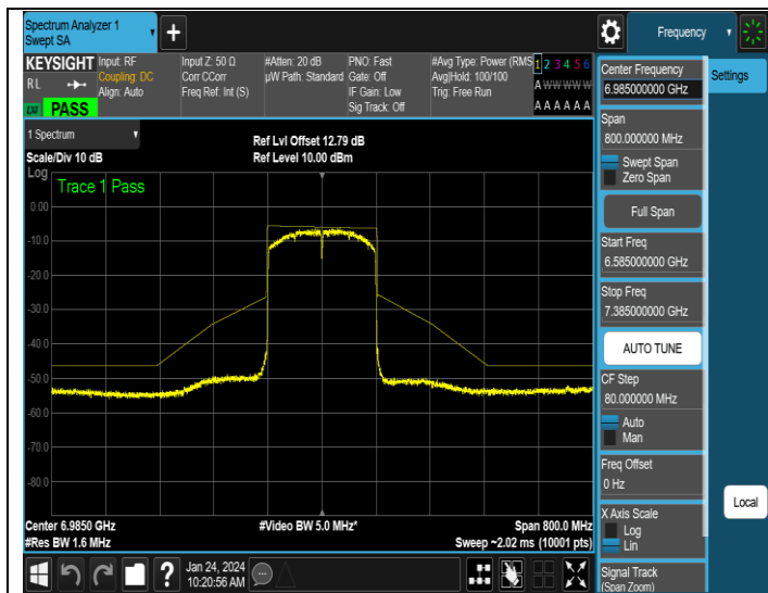
NTNV-11AX160SISO-Ant3-6985-PASS
