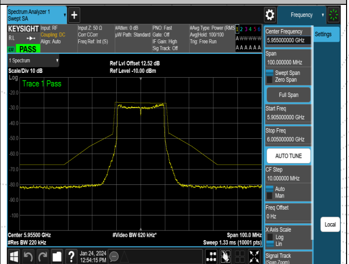
NTNV-11AX20MIMO-Ant4-5955-PASS
