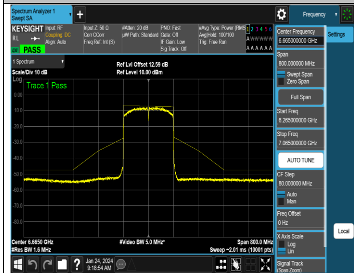
NTNV-11AX160SISO-Ant1-6665-PASS
