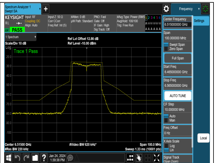
NTNV-11AX20MIMO-Ant4-6515-PASS
