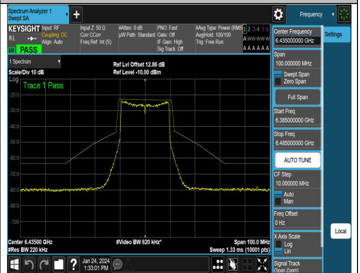
NTNV-11AX20MIMO-Ant2-6435-PASS
