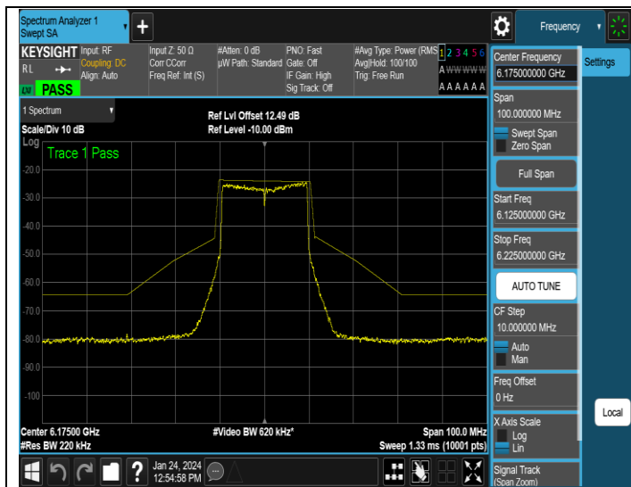
NTNV-11AX20MIMO-Ant1-6175-PASS
