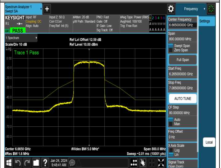
NTNV-11AX160SISO-Ant2-6665-PASS
