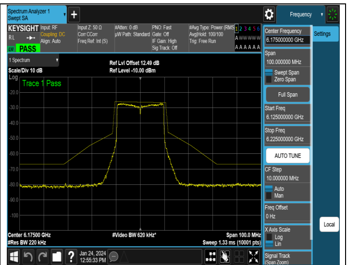
NTNV-11AX20MIMO-Ant2-6175-PASS
