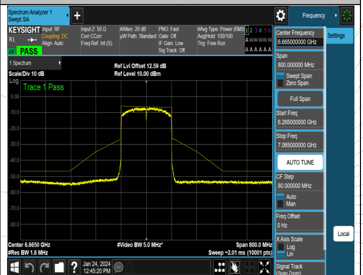
NTNV-11AX160SISO-Ant4-6665-PASS
