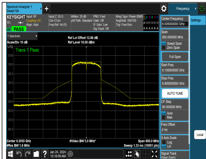
NTNV-11AX160SISO-Ant3-6505-PASS
