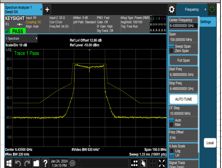
NTNV-11AX20MIMO-Ant4-6435-PASS
