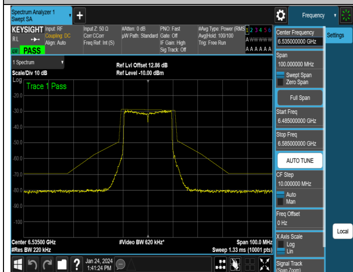
NTNV-11AX20MIMO-Ant3-6535-PASS
