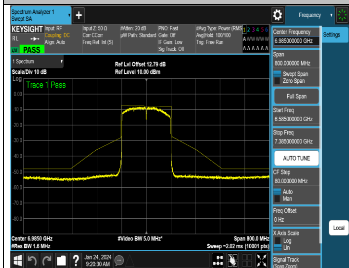
NTNV-11AX160SISO-Ant1-6985-PASS
