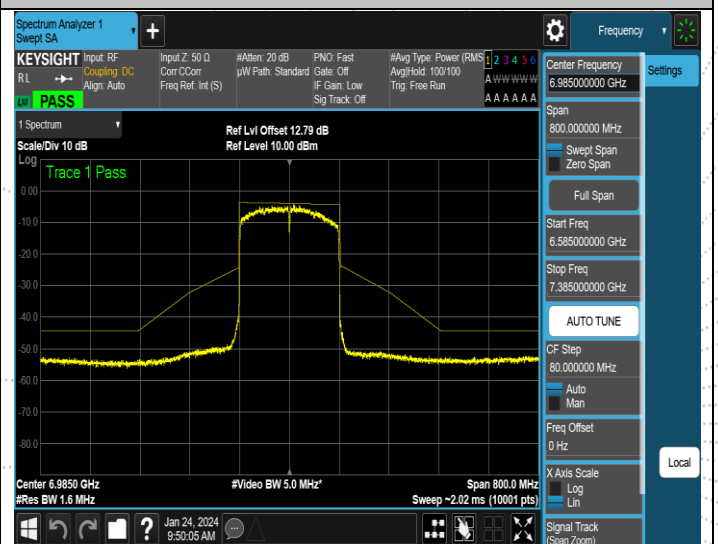
NTNV-11AX160SISO-Ant2-6985-PASS
