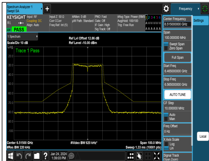
NTNV-11AX20MIMO-Ant3-6515-PASS
