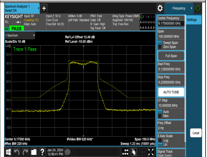
NTNV-11AX20MIMO-Ant4-6175-PASS
