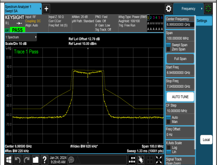
NTNV-11AX20SISO-Ant2-6995-PASS
