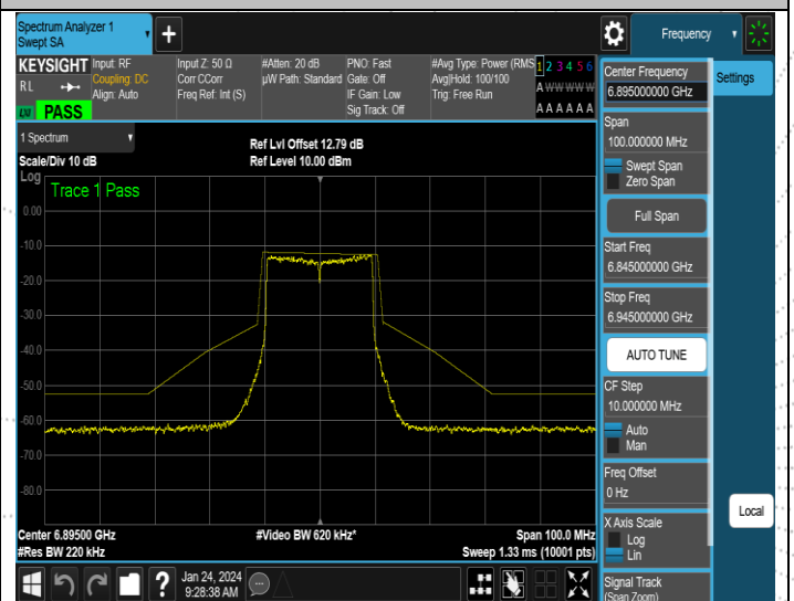
NTNV-11AX20SISO-Ant2-6895-PASS
