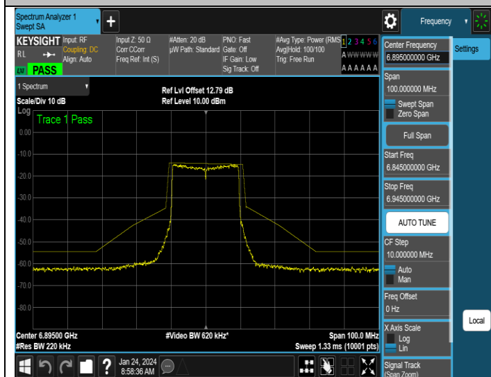
NTNV-11AX20SISO-Ant1-6895-PASS
