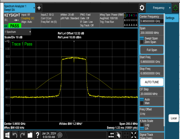
NTNV-11AX40SISO-Ant2-5965-PASS
