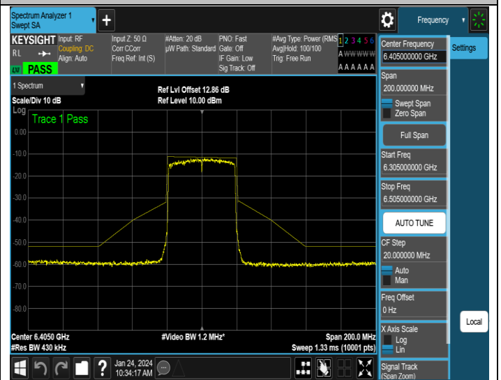
NTNV-11AX40SISO-Ant4-6405-PASS
