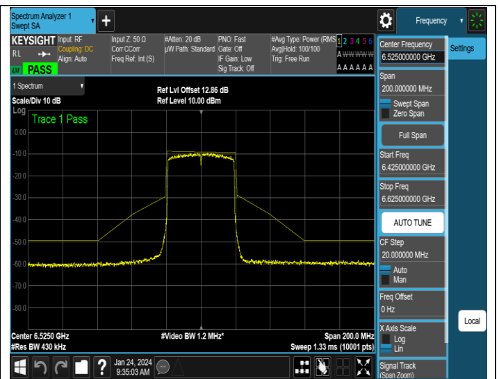
NTNV-11AX40SISO-Ant2-6525-PASS
