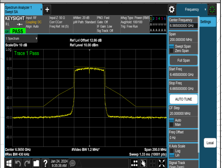
NTNV-11AX40SISO-Ant2-6565-PASS
