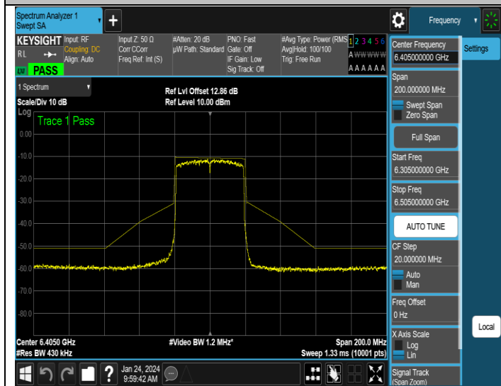
NTNV-11AX40SISO-Ant3-6405-PASS
