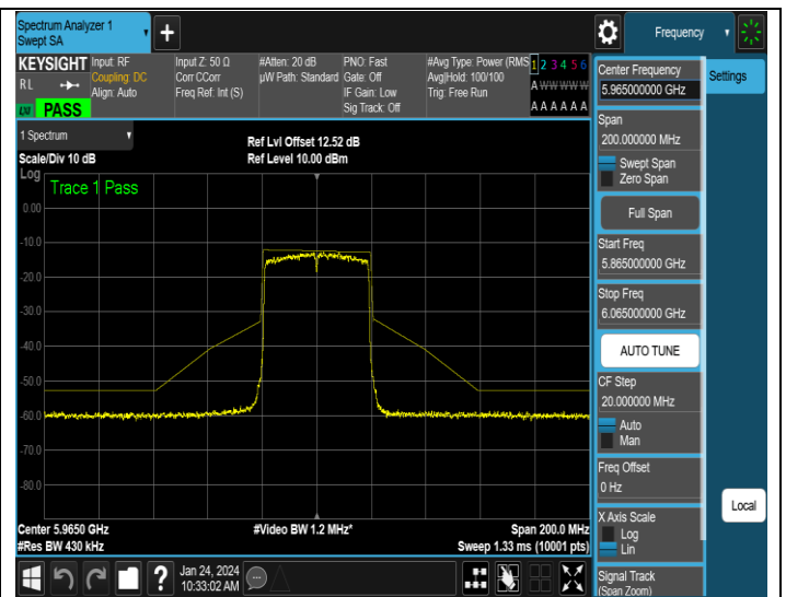
NTNV-11AX40ISO-Ant4-5965-PASS
