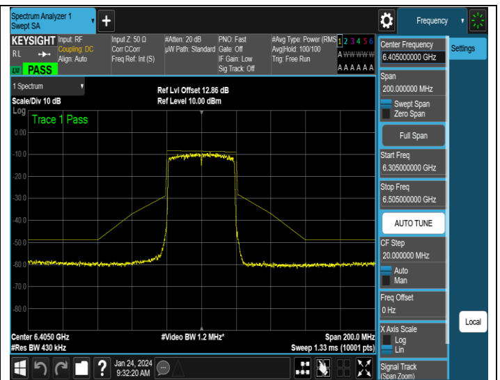
NTNV-11AX40SISO-Ant2-6405-PASS
