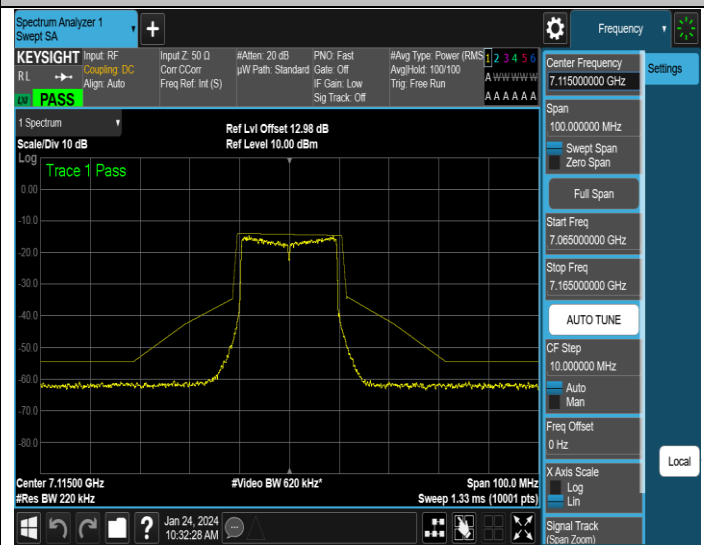
NTNV-11AX20SISO-Ant4-7115-PASS
