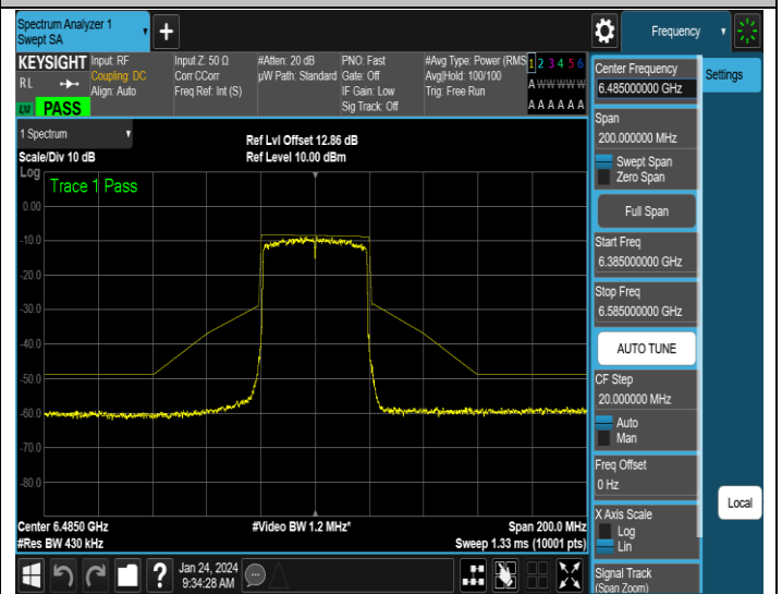
NTNV-11AX40ISO-Ant2-6485-PASS
