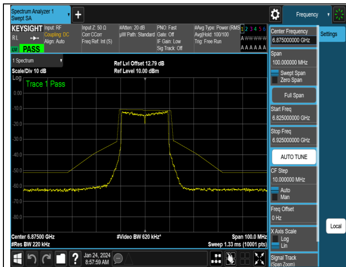
NTNV-11AX20SISO-Ant1-6875-PASS
