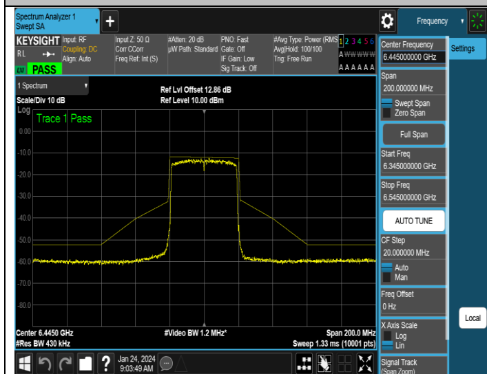
NTNV-11AX40SISO-Ant1-6445-PASS
