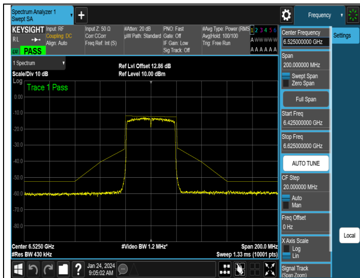
NTNV-11AX40SISO-Ant1-6525-PASS
