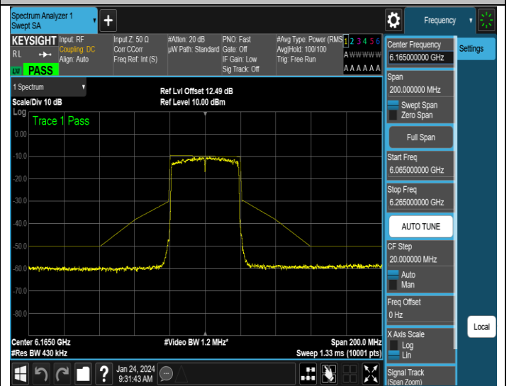
NTNV-11AX40ISO-Ant2-6165-PASS
