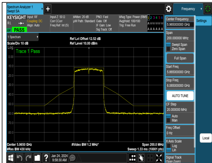
NTNV-11AX40ISO-Ant3-5965-PASS
