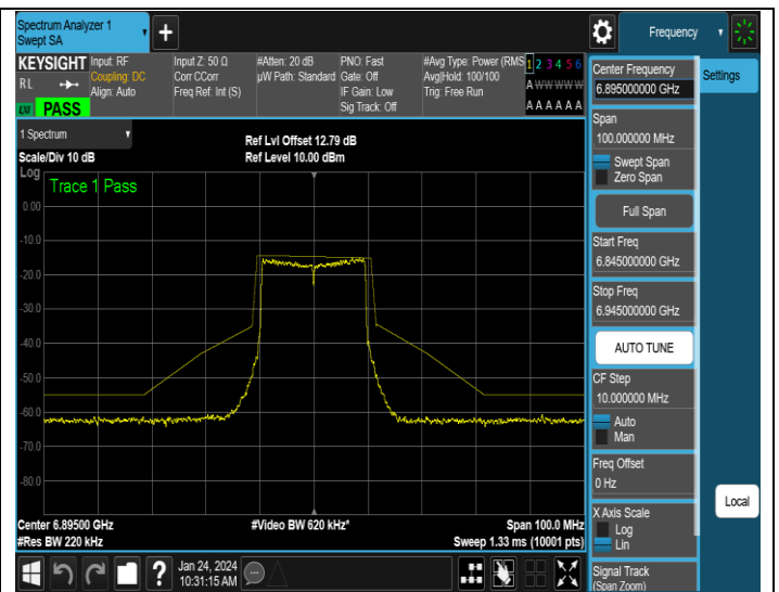
NTNV-11AX20SISO-Ant4-6895-PASS
