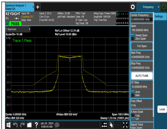
NTNV-11AX20SISO-Ant3-6895-PASS
