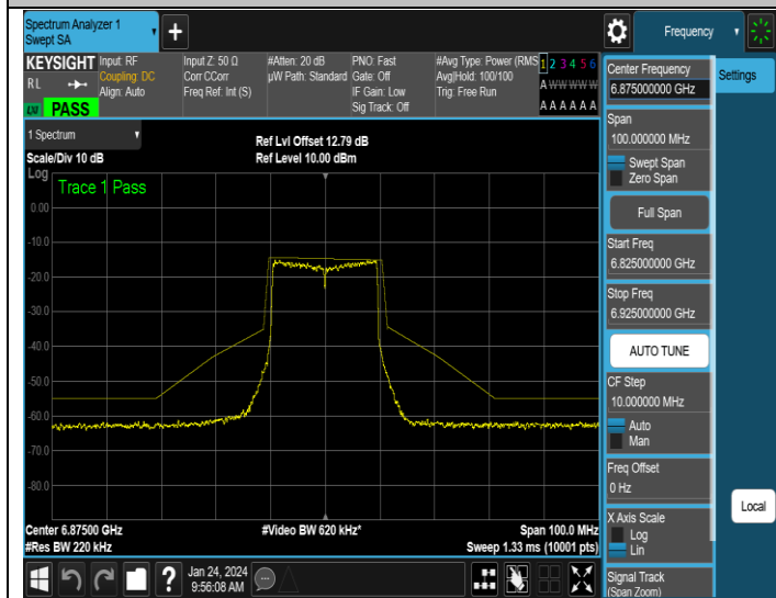
NTNV-11AX20SISO-Ant3-6875-PASS
