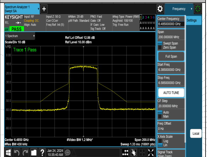
NTNV-11AX40ISO-Ant4-6485-PASS
