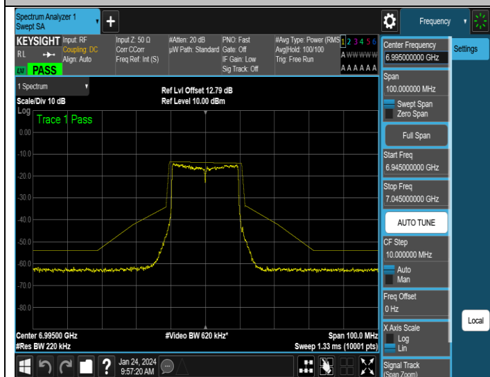
NTNV-11AX20SISO-Ant3-6995-PASS
