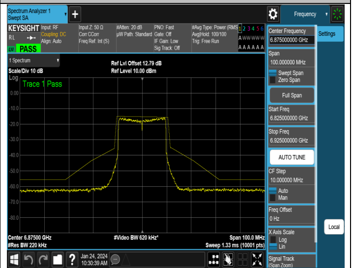
NTNV-11AX20SISO-Ant4-6875-PASS
