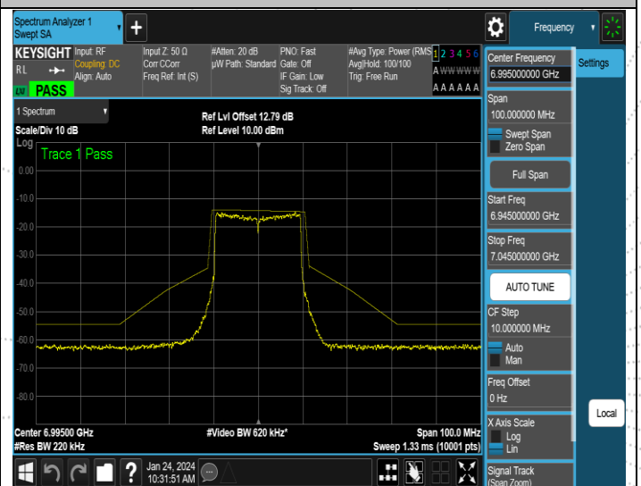
NTNV-11AX20SISO-Ant4-6995-PASS
