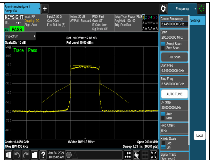
NTNV-11AX40ISO-Ant4-6445-PASS
