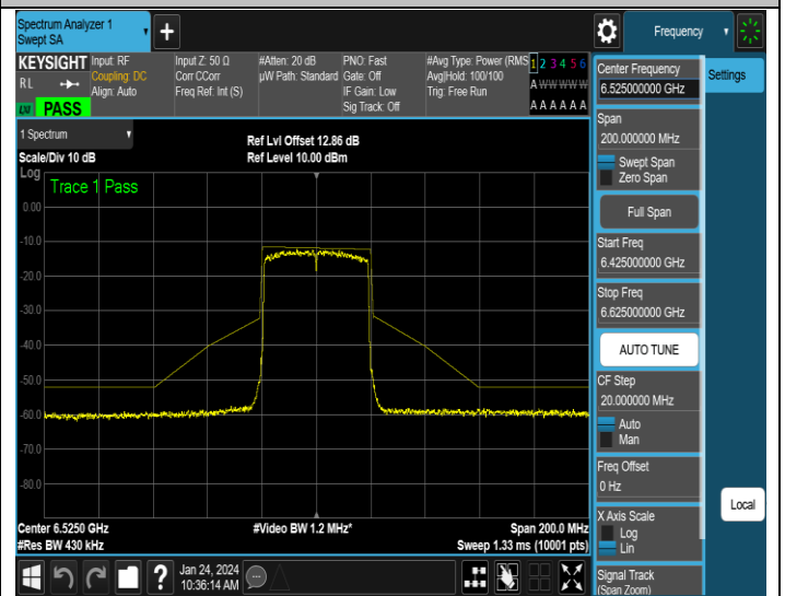
NTNV-11AX40SISO-Ant4-6525-PASS
