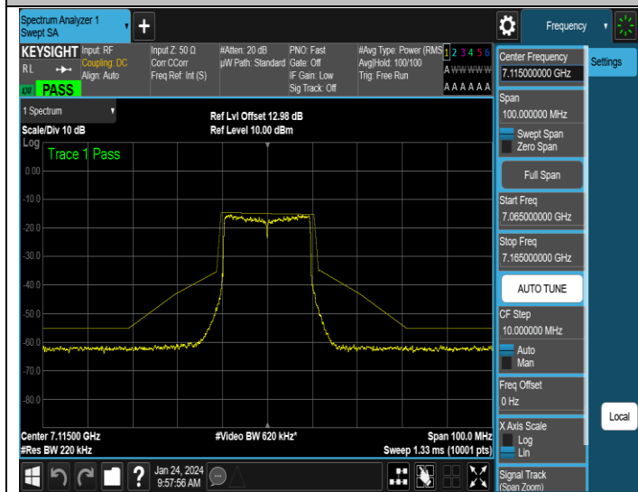
NTNV-11AX20SISO-Ant3-7115-PASS
