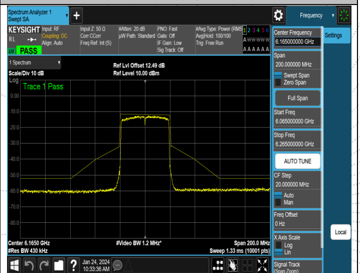
NTNV-11AX40ISO-Ant4-6165-PASS
