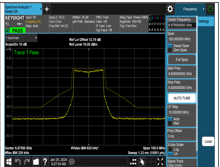
NTNV-11AX20SISO-Ant2-6875-PASS
