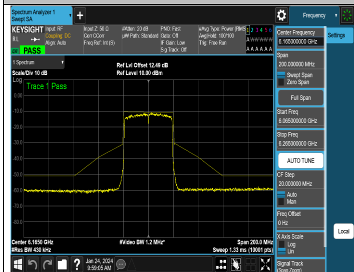
NTNV-11AX40ISO-Ant3-6165-PASS
