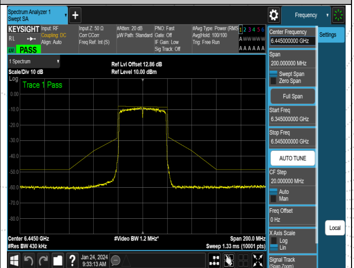
NTNV-11AX40SISO-Ant2-6445-PASS
