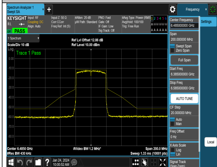
NTNV-11AX40ISO-Ant3-6485-PASS
