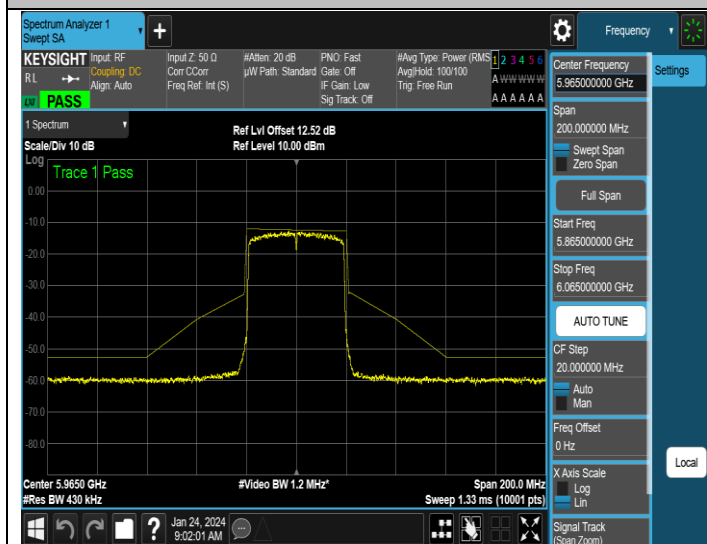
NTNV-11AX40SISO-Ant1-5965-PASS
