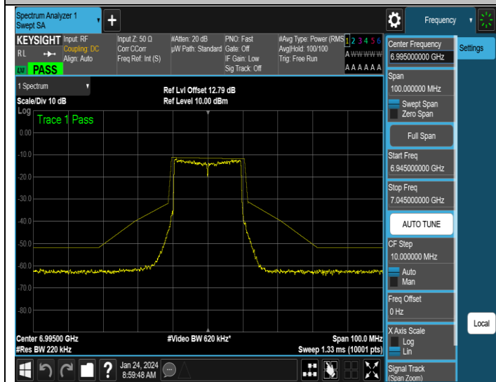
NTNV-11AX20SISO-Ant1-6995-PASS
