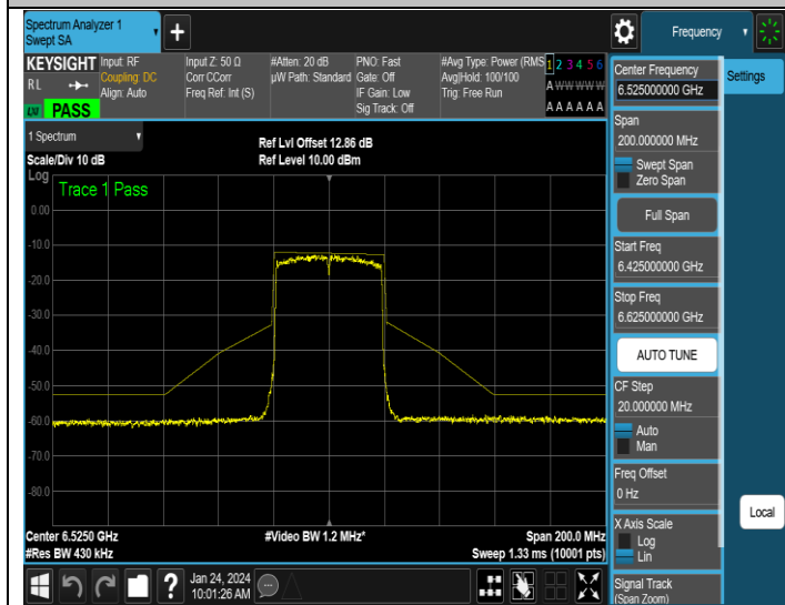
NTNV-11AX40SISO-Ant3-6525-PASS
