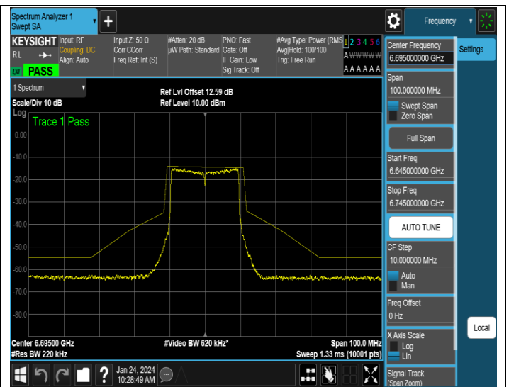
NTNV-11AX20SISO-Ant4-6695-PASS
