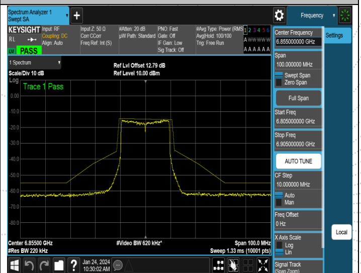
NTNV-11AX20SISO-Ant4-6855-PASS
