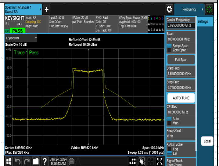
NTNV-11AX20SISO-Ant2-6695-PASS
