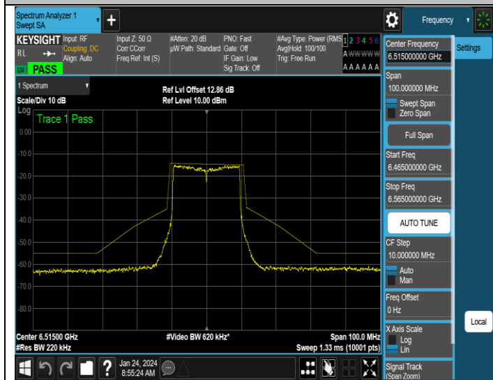
NTNV-11AX20SISO-Ant1-6515-PASS
