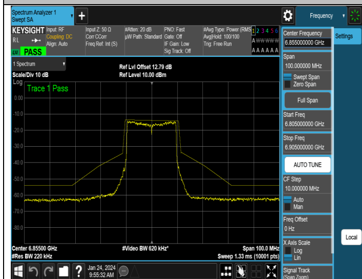
NTNV-11AX20SISO-Ant3-6855-PASS
