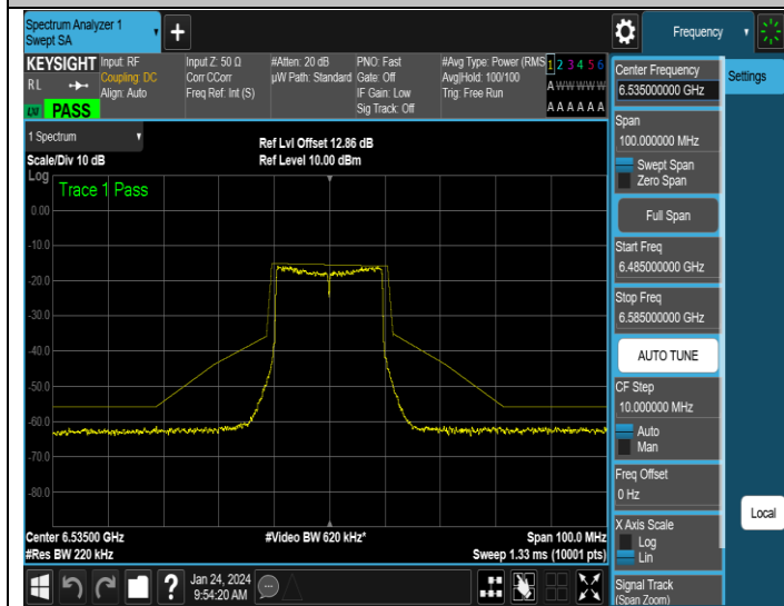
NTNV-11AX20SISO-Ant3-6535-PASS
