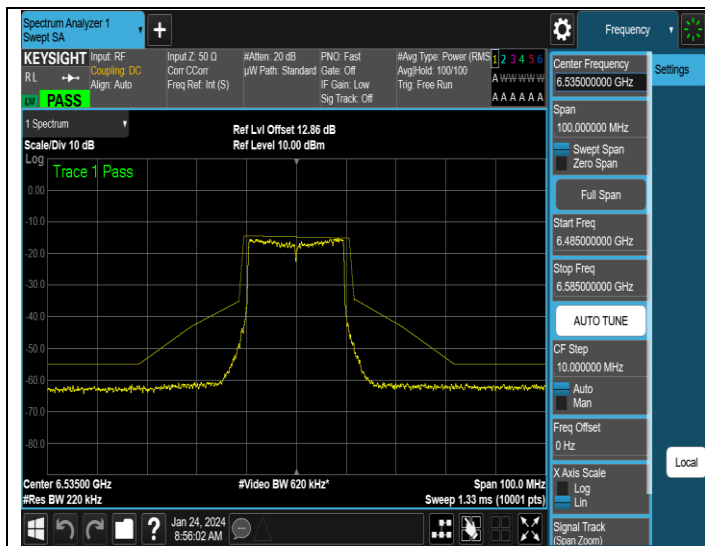
NTNV-11AX20SISO-Ant1-6535-PASS
