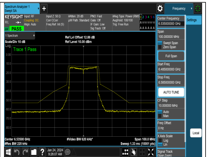
NTNV-11AX20SISO-Ant2-6535-PASS
