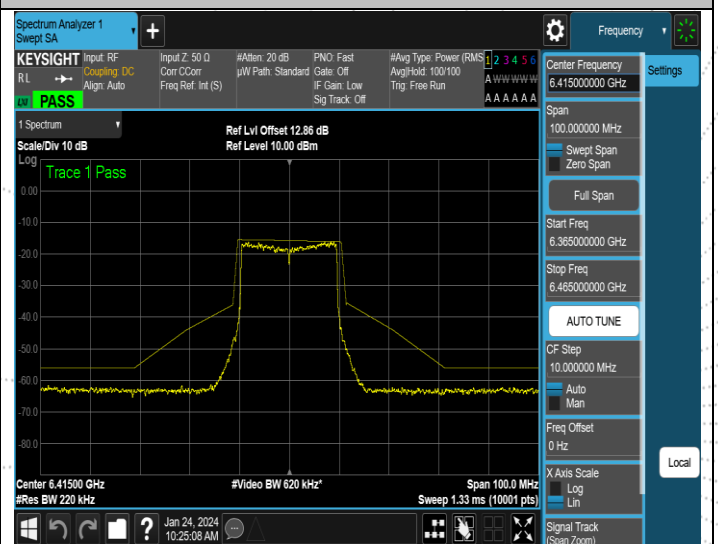
NTNV-11AX20SISO-Ant4-6415-PASS
