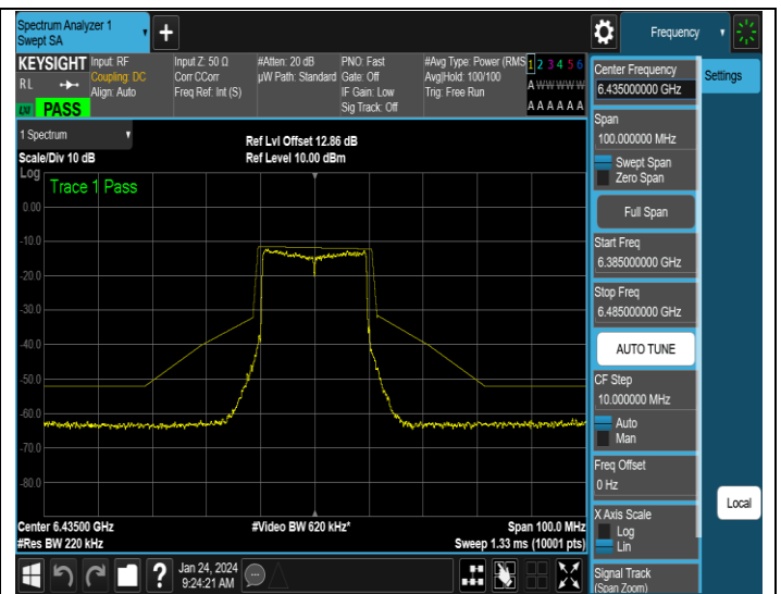
NTNV-11AX20SISO-Ant2-6435-PASS
