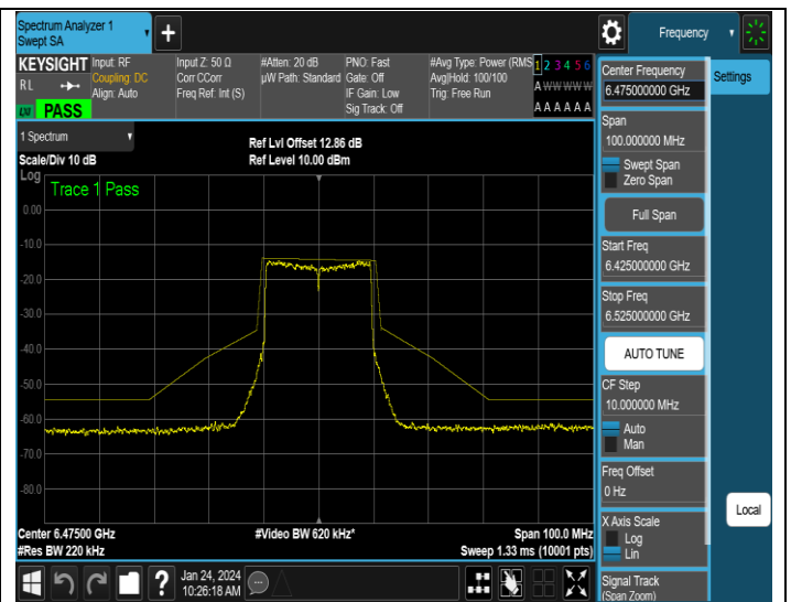
NTNV-11AX20SISO-Ant4-6475-PASS
