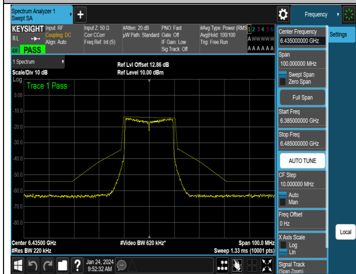
NTNV-11AX20SISO-Ant3-6435-PASS
