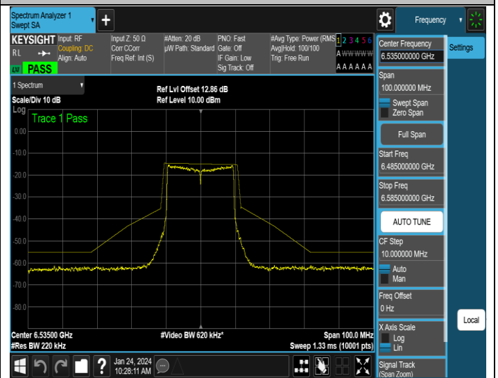
NTNV-11AX20SISO-Ant4-6535-PASS
