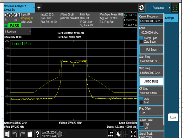
NTNV-11AX20SISO-Ant4-6515-PASS
