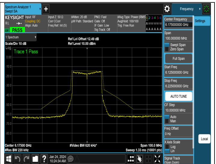
NTNV-11AX20SISO-Ant4-6175-PASS
