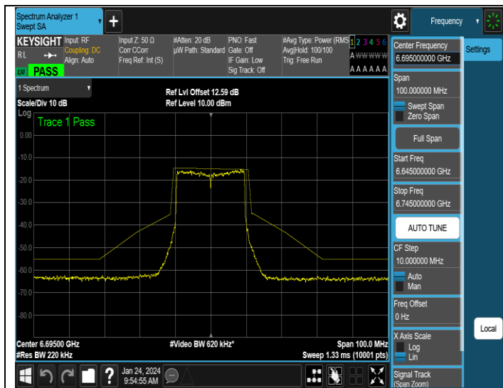
NTNV-11AX20SISO-Ant3-6695-PASS
