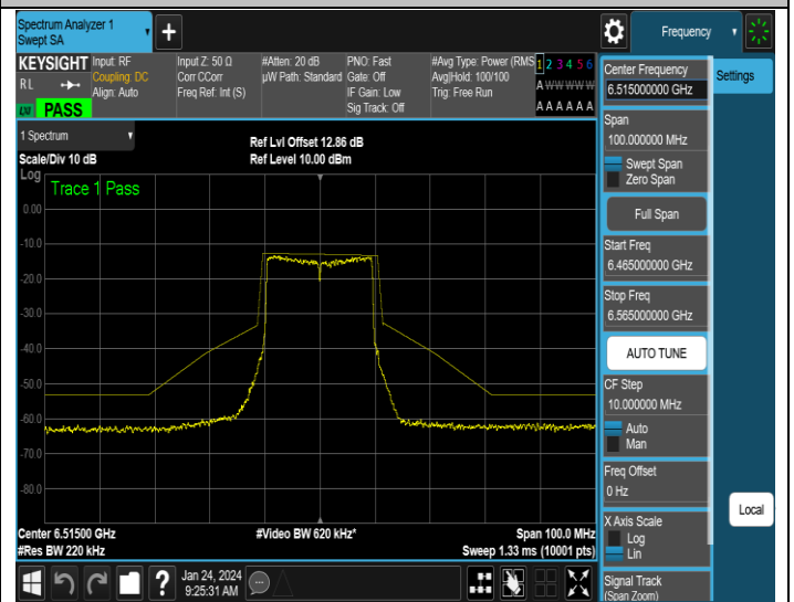
NTNV-11AX20SISO-Ant2-6515-PASS
