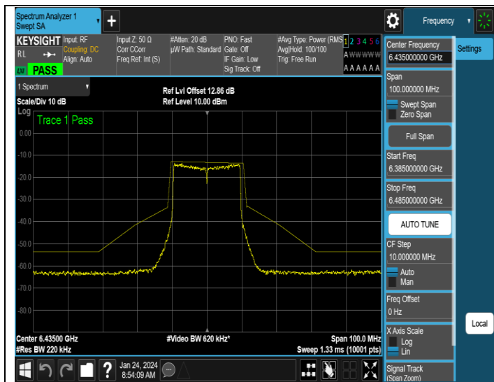
NTNV-11AX20SISO-Ant1-6435-PASS
