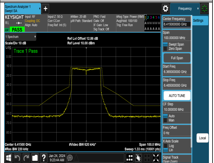
NTNV-11AX20SISO-Ant2-6415-PASS
