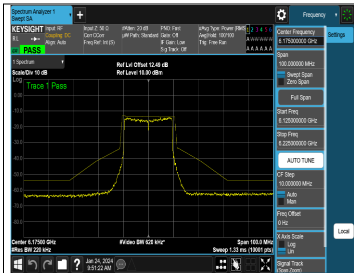
NTNV-11AX20SISO-Ant3-6175-PASS
