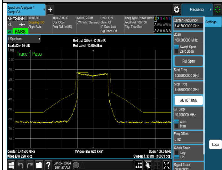
NTNV-11AX20SISO-Ant3-6415-PASS
