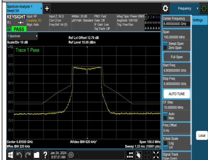
NTNV-11AX20SISO-Ant1-6855-PASS
