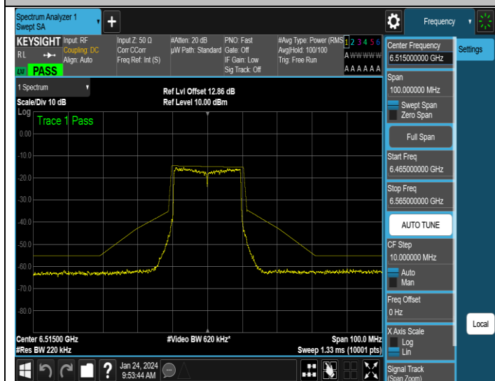
NTNV-11AX20SISO-Ant3-6515-PASS
