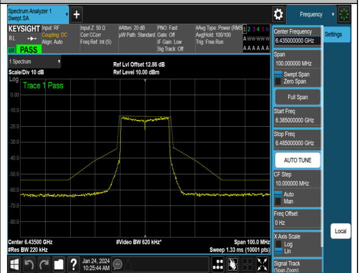
NTNV-11AX20SISO-Ant4-6435-PASS
