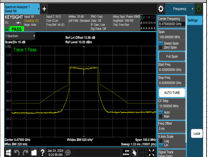
NTNV-11AX20SISO-Ant2-6475-PASS
