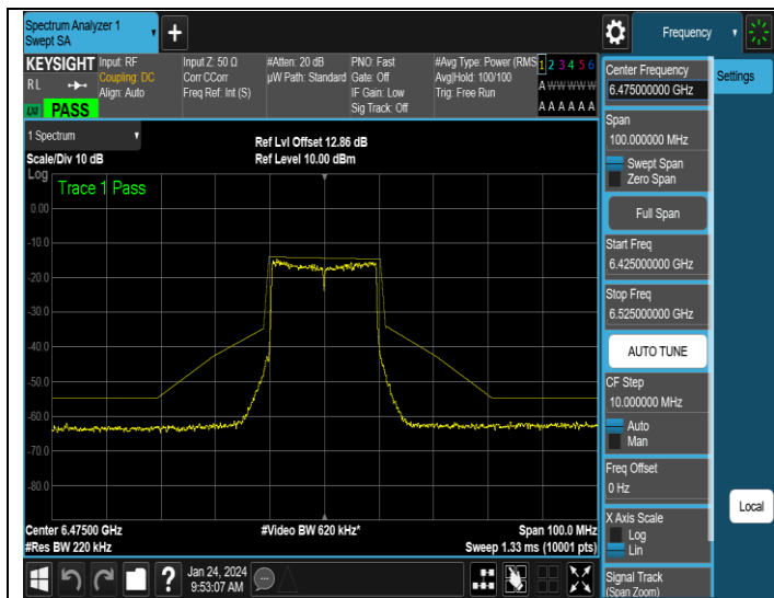
NTNV-11AX20SISO-Ant3-6475-PASS
