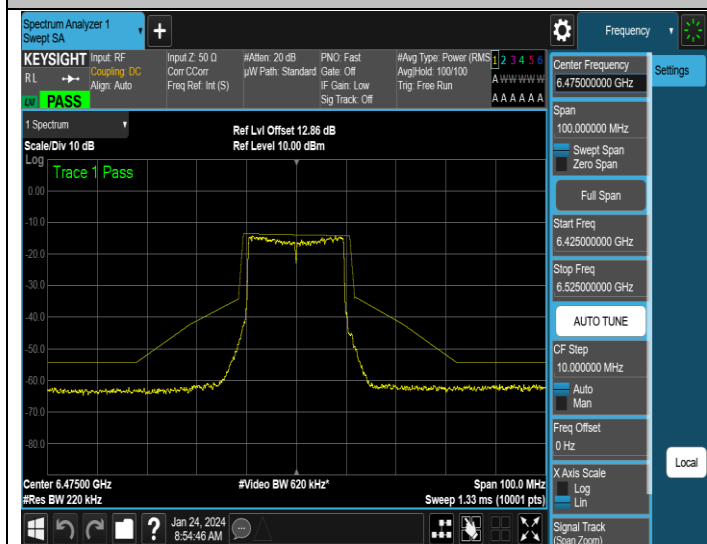
NTNV-11AX20SISO-Ant1-6475-PASS
