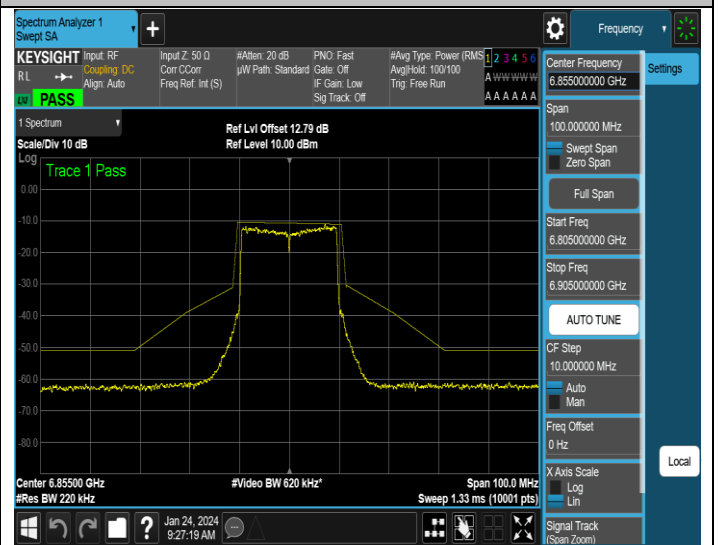
NTNV-11AX20SISO-Ant2-6855-PASS
