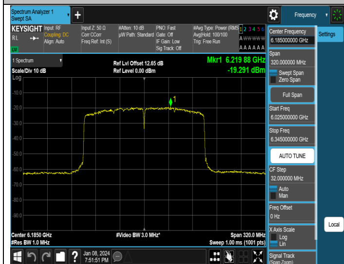
11AX160MIMO-Ant1-6185-PASS
