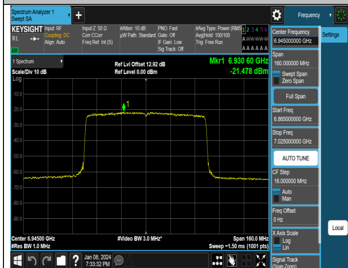
11AX80MIMO-Ant1-6945-PASS
