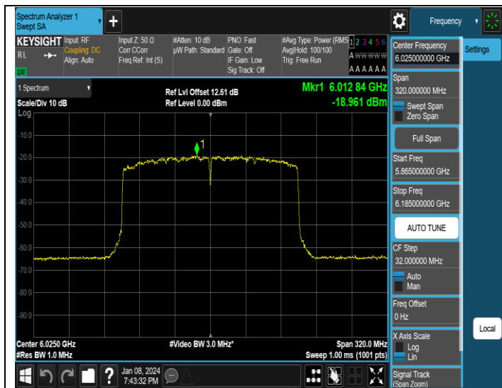
11AX160MIMO-Ant1-6025-PASS
