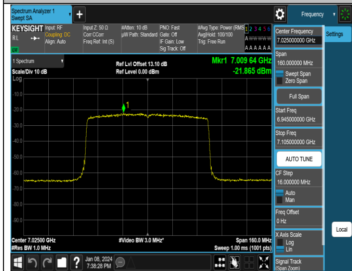
11AX80MIMO-Ant1-7025-PASS
