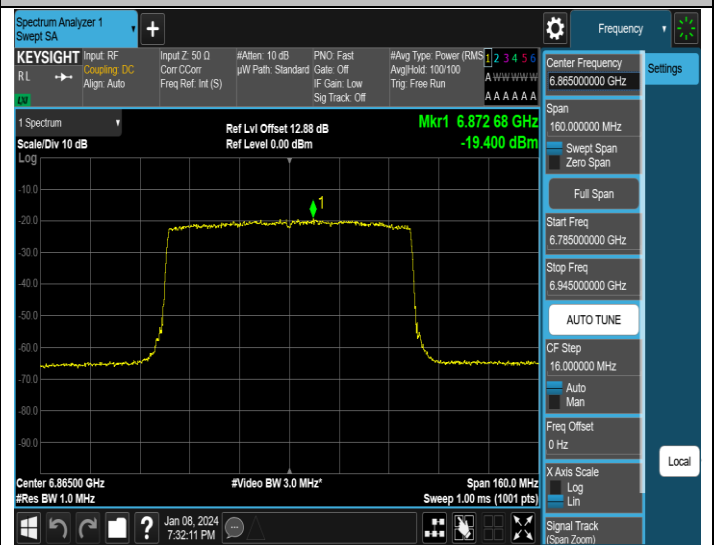
11AX80MIMO-Ant4-6865-PASS
