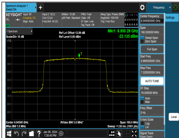
11AX80MIMO-Ant3-6945-PASS
