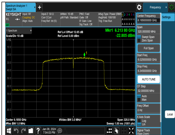
11AX160MIMO-Ant3-6185-PASS
