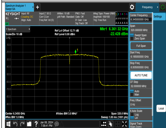
11AX160MIMO-Ant3-6345-PASS
