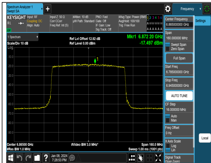
11AX80MIMO-Ant1-6865-PASS
