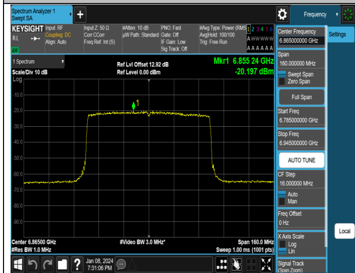
11AX80MIMO-Ant3-6865-PASS
