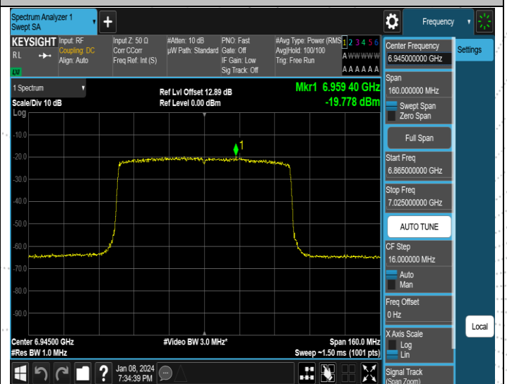
11AX80MIMO-Ant2-6945-PASS
