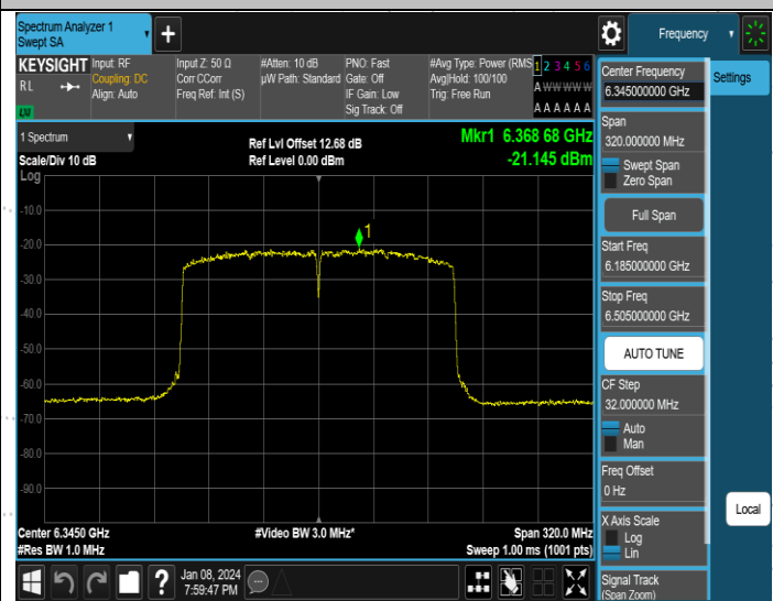
11AX160MIMO-Ant4-6345-PASS
