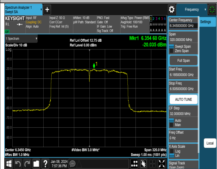
11AX160MIMO-Ant2-6345-PASS
