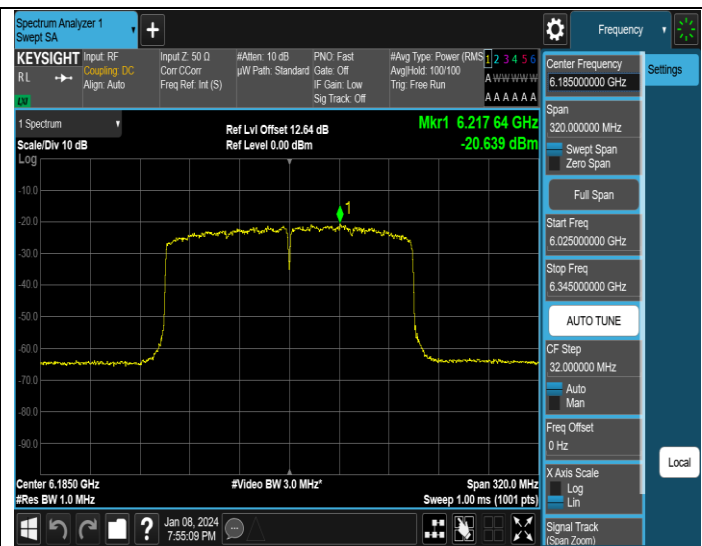
11AX160MIMO-Ant4-6185-PASS
