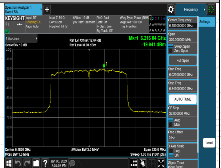
11AX160MIMO-Ant2-6185-PASS
