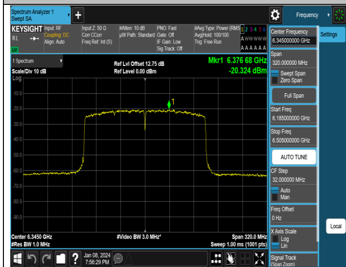
11AX160MIMO-Ant1-6345-PASS
