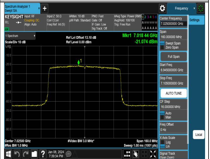
11AX80MIMO-Ant2-7025-PASS
