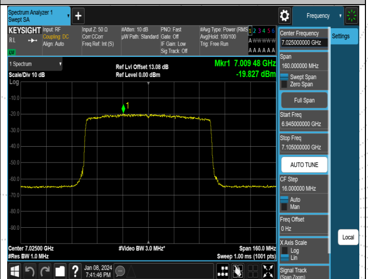
11AX80MIMO-Ant4-7025-PASS
