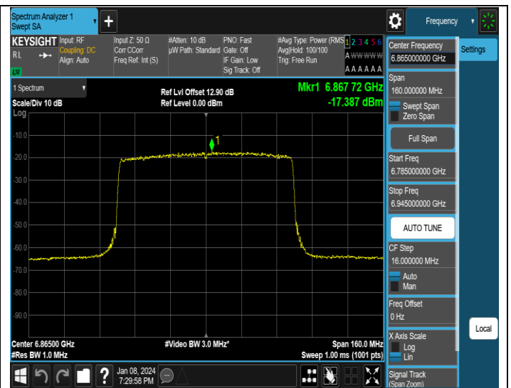
11AX80MIMO-Ant2-6865-PASS
