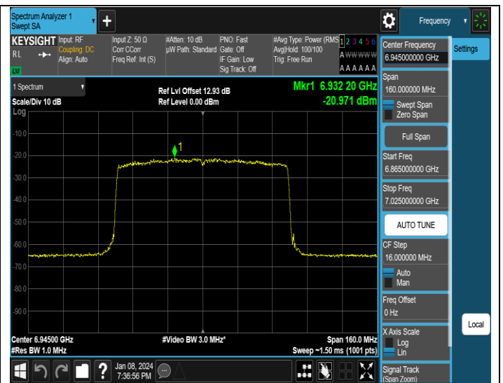
11AX80MIMO-Ant4-6945-PASS
