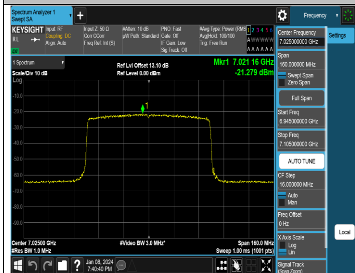
11AX80MIMO-Ant3-7025-PASS
