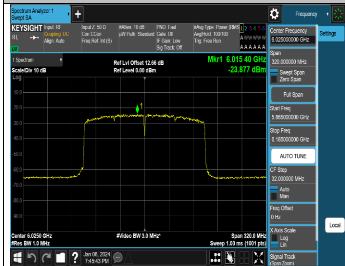
11AX160MIMO-Ant3-6025-PASS
