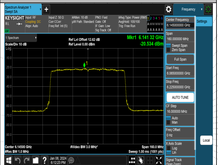
11AX80MIMO-Ant4-6145-PASS
