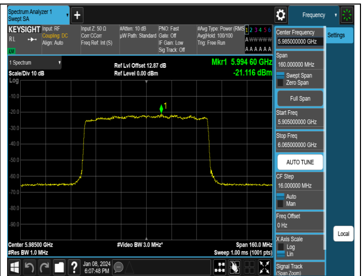
11AX80MIMO-Ant4-5985-PASS
