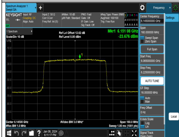
11AX80MIMO-Ant3-6145-PASS
