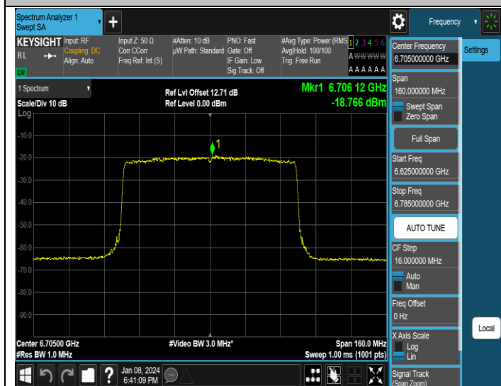
11AX80MIMO-Ant1-6705-PASS
