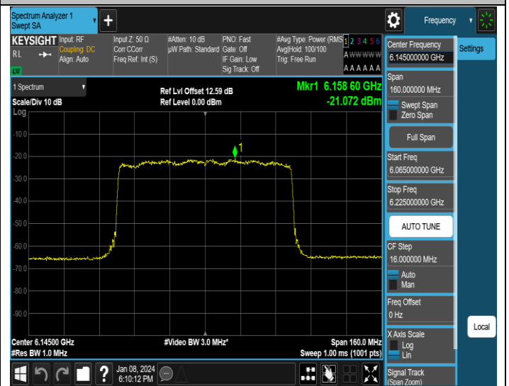
11AX80MIMO-Ant2-6145-PASS
