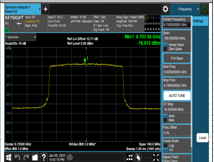
11AX80MIMO-Ant2-6705-PASS
