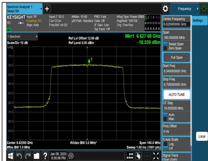
11AX80MIMO-Ant1-6625-PASS
