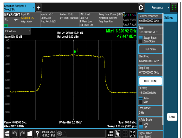
11AX80MIMO-Ant2-6625-PASS
