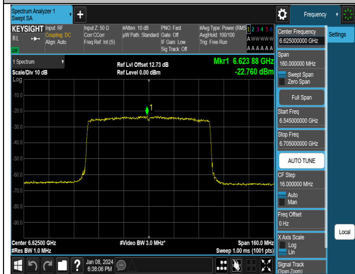
11AX80MIMO-Ant3-6625-PASS
