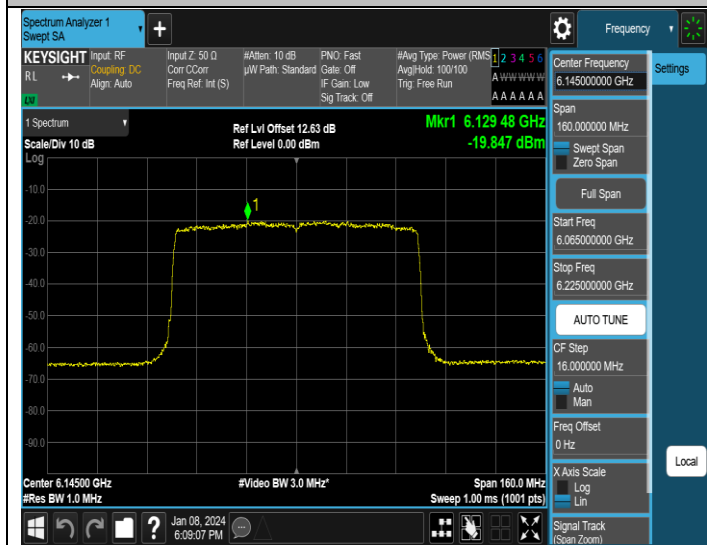
11AX80MIMO-Ant1-6145-PASS
