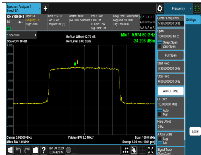
11AX80MIMO-Ant3-5985-PASS
