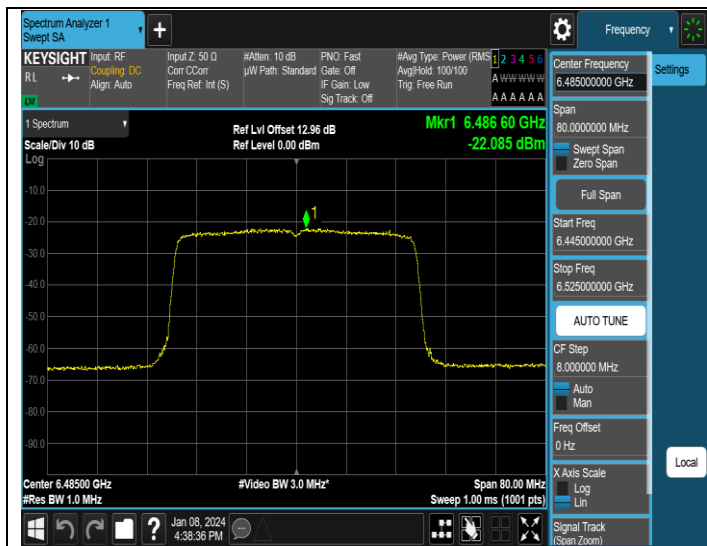
11AX40MIMO-Ant3-6485-PASS
