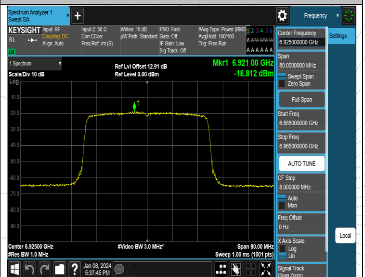
11AX40MIMO-Ant2-6925-PASS
