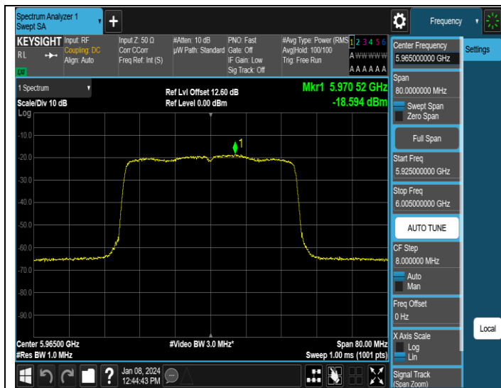
11AX40MIMO-Ant1-5965-PASS
