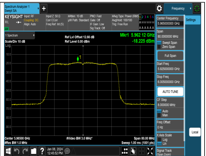
11AX40MIMO-Ant2-5965-PASS
