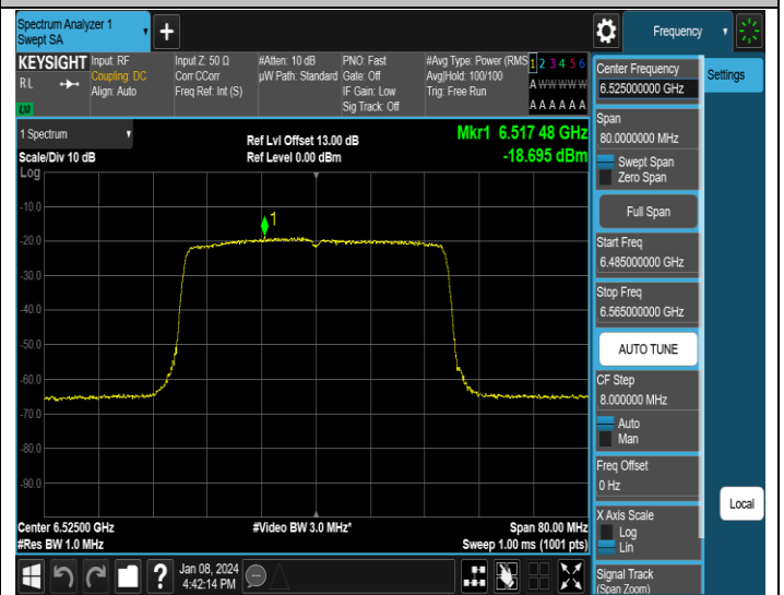
11AX40MIMO-Ant2-6525-PASS
