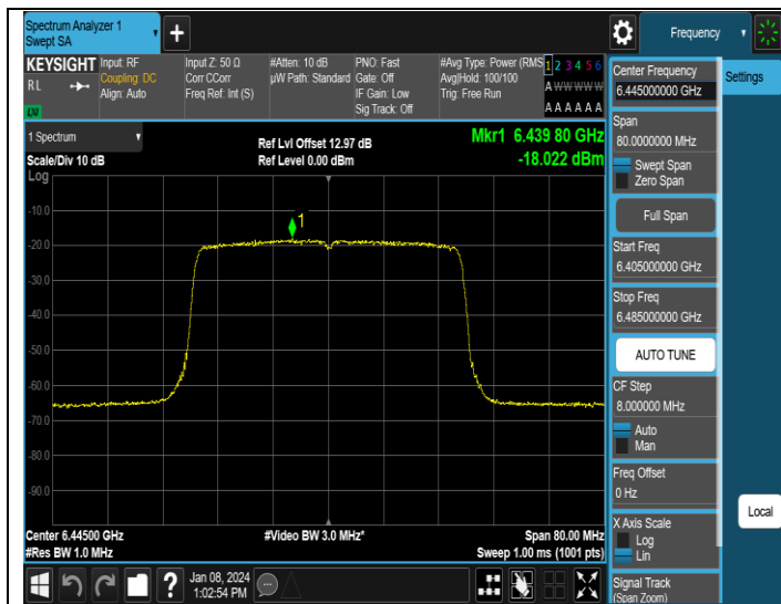
11AX40MIMO-Ant1-6445-PASS
