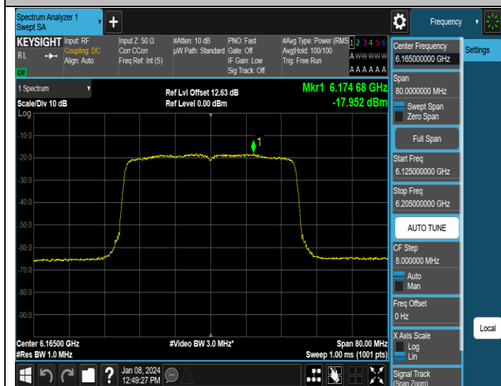
11AX40MIMO-Ant1-6165-PASS
