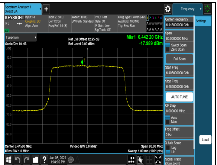
11AX40MIMO-Ant2-6445-PASS
