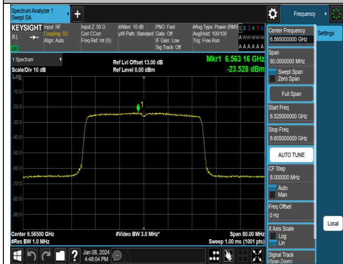
11AX40MIMO-Ant3-6565-PASS
