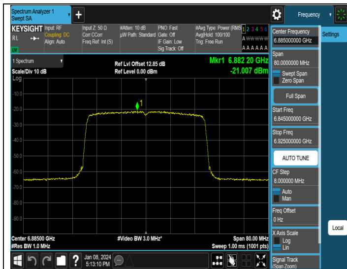
11AX40MIMO-Ant1-6885-PASS
