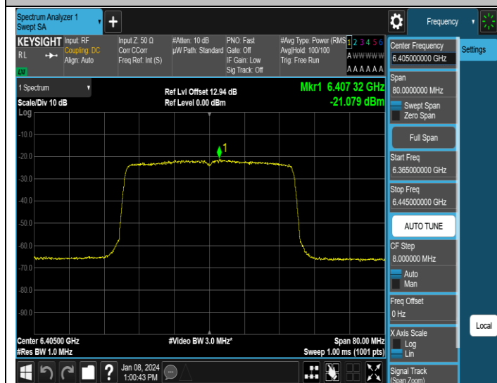
11AX40MIMO-Ant3-6405-PASS
