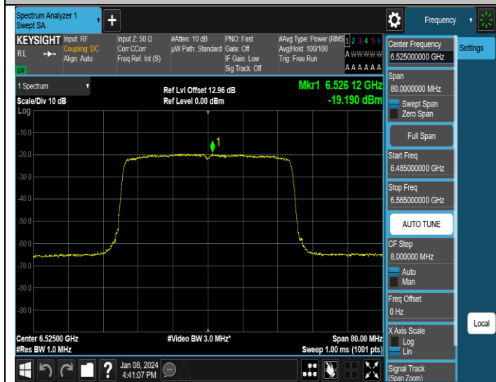
11AX40MIMO-Ant1-6525-PASS
