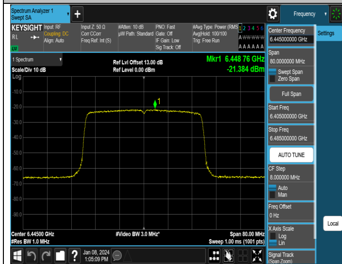
11AX40MIMO-Ant3-6445-PASS
