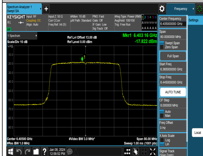
11AX40MIMO-Ant1-6405-PASS
