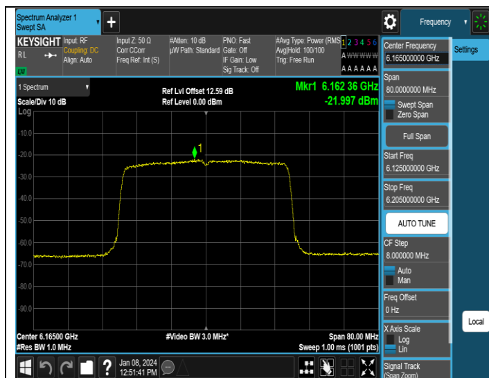
11AX40MIMO-Ant3-6165-PASS
