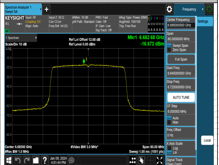
11AX40MIMO-Ant2-6685-PASS
