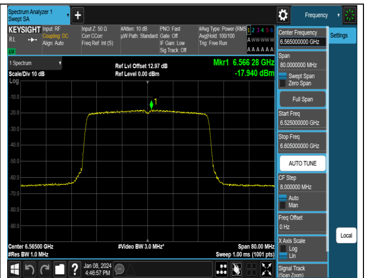
11AX40MIMO-Ant2-6565-PASS
