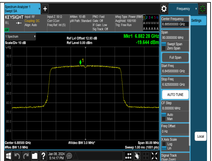
11AX40MIMO-Ant2-6885-PASS
