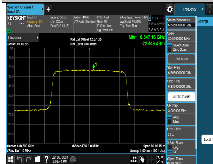
11AX40MIMO-Ant3-6845-PASS
