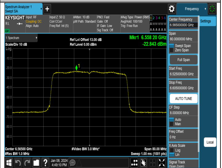
11AX40MIMO-Ant4-6565-PASS
