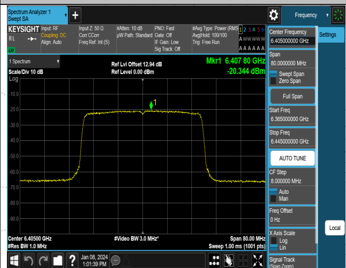
11AX40MIMO-Ant4-6405-PASS
