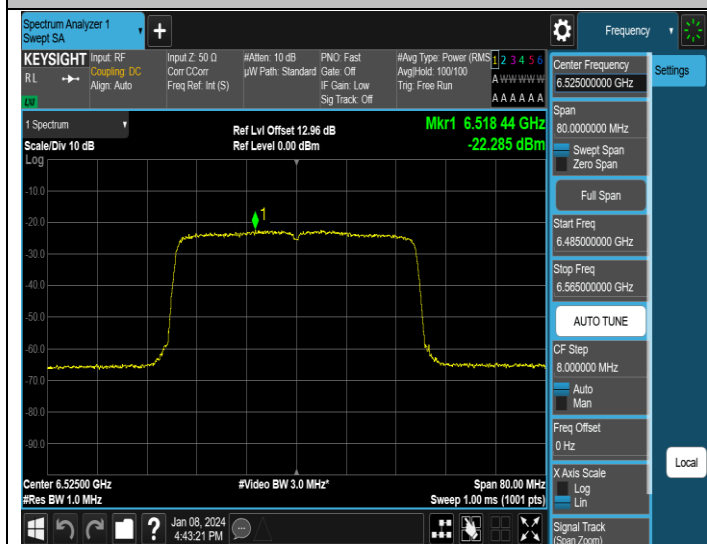
11AX40MIMO-Ant3-6525-PASS
