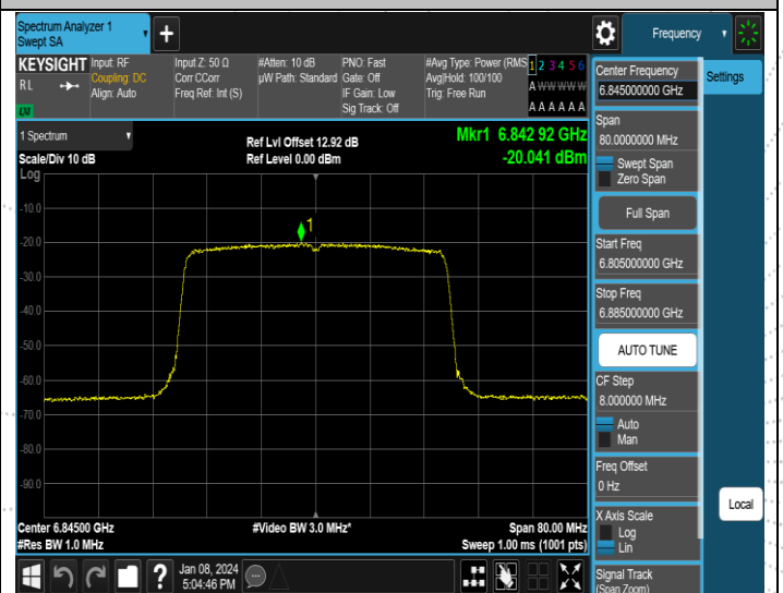
11AX40MIMO-Ant4-6845-PASS
