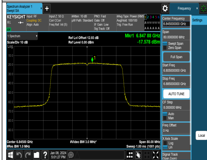
11AX40MIMO-Ant1-6845-PASS
