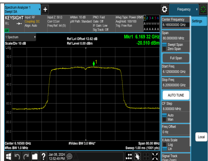
11AX40MIMO-Ant4-6165-PASS
