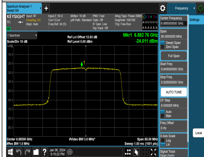
11AX40MIMO-Ant3-6885-PASS
