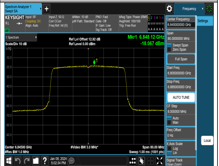
11AX40MIMO-Ant2-6845-PASS
