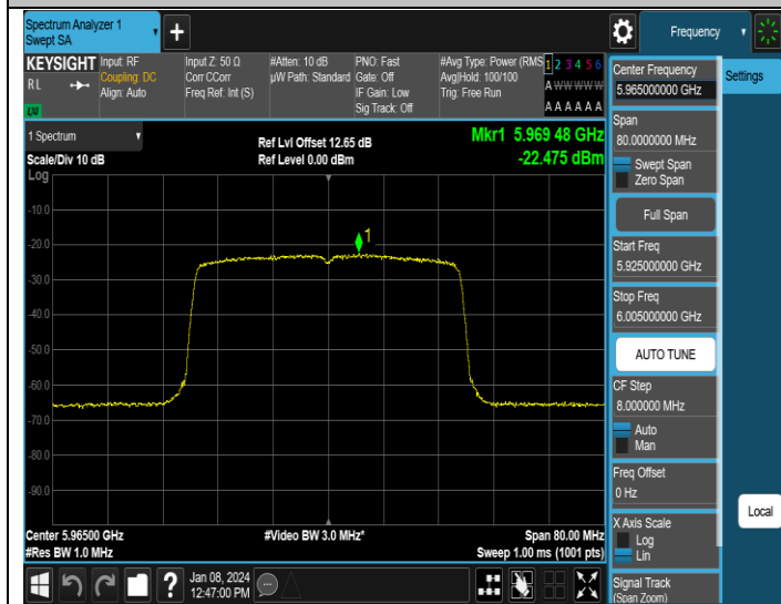
11AX40MIMO-Ant3-5965-PASS
