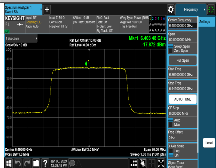
11AX40MIMO-Ant2-6405-PASS
