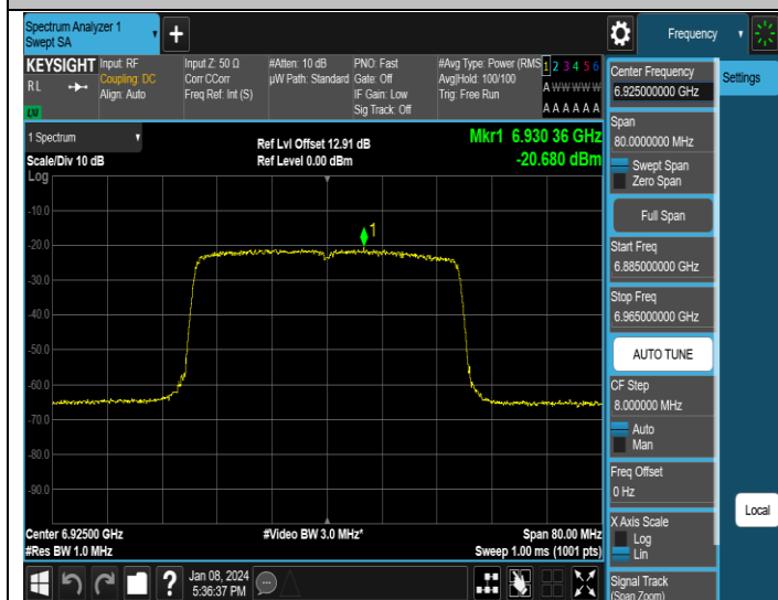
11AX40MIMO-Ant1-6925-PASS
