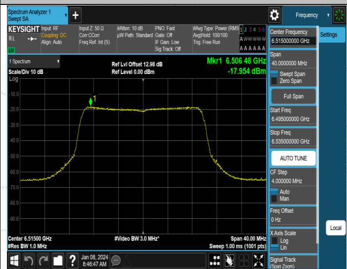
11AX20MIMO-Ant2-6515-PASS
