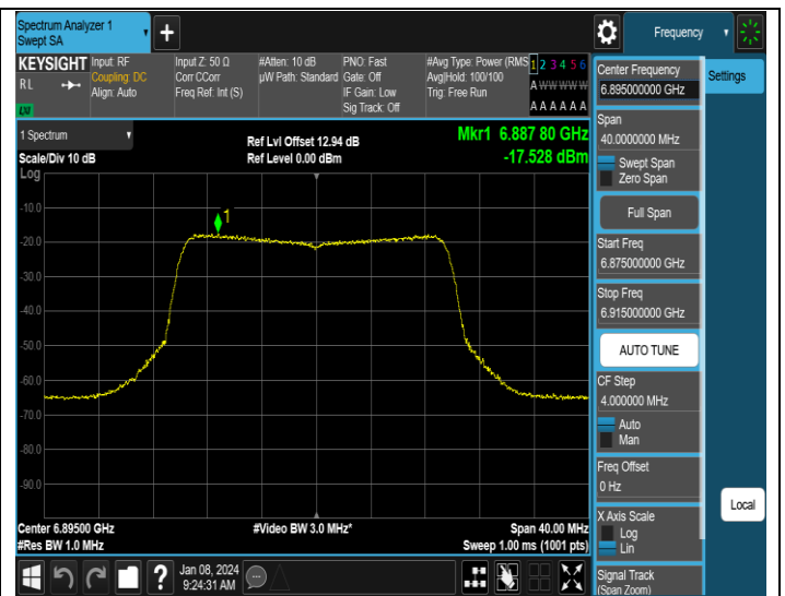
11AX20MIMO-Ant2-6895-PASS
