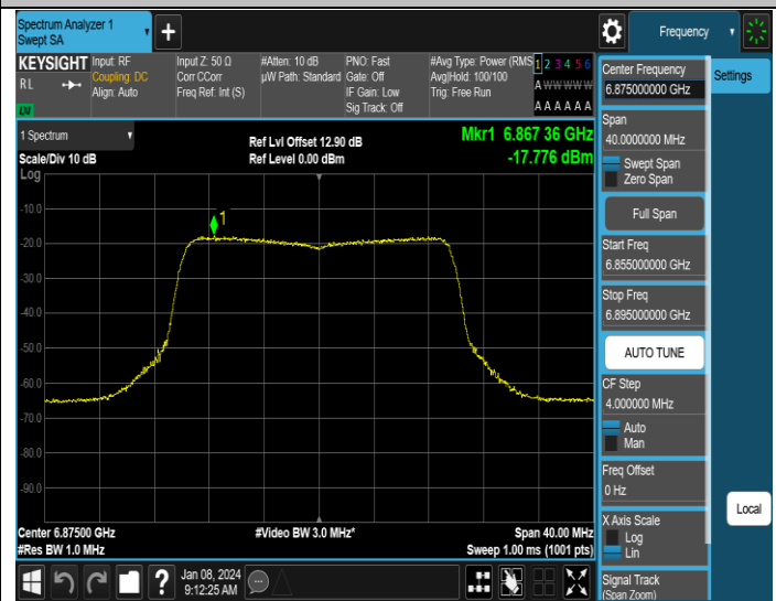
11AX20MIMO-Ant2-6875-PASS
