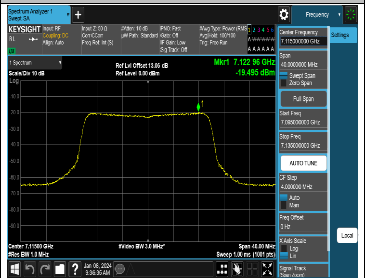
11AX20MIMO-Ant2-7115-PASS
