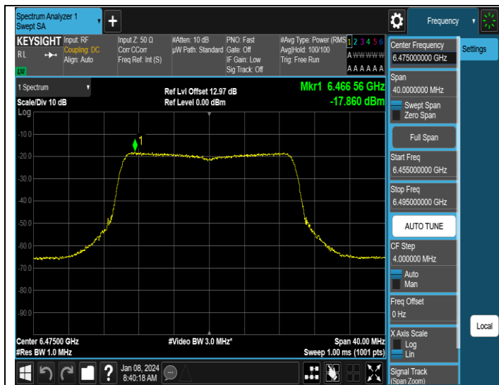
11AX20MIMO-Ant1-6475-PASS
