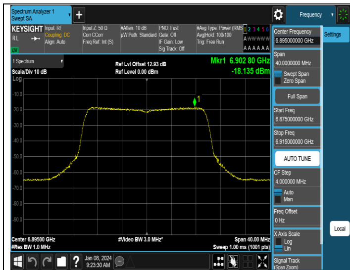
11AX20MIMO-Ant1-6895-PASS
