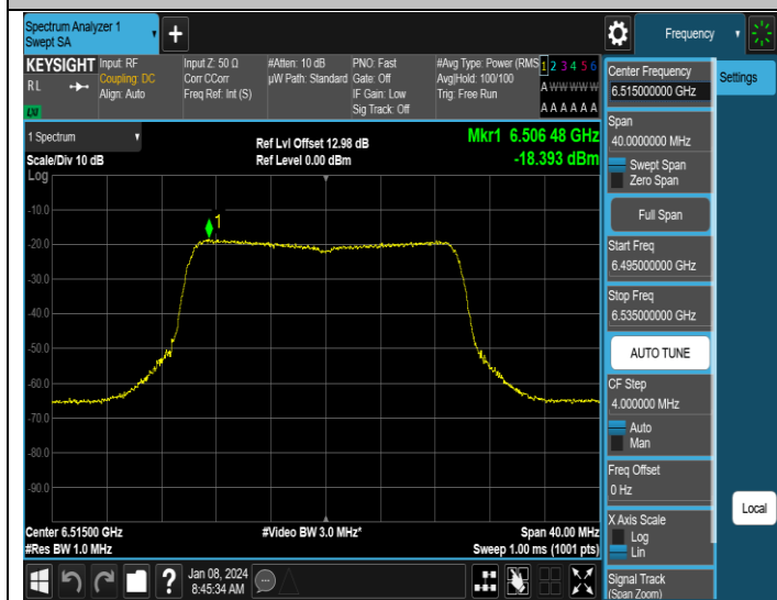
11AX20MIMO-Ant1-6515-PASS
