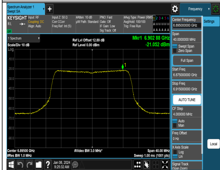
11AX20MIMO-Ant3-6895-PASS
