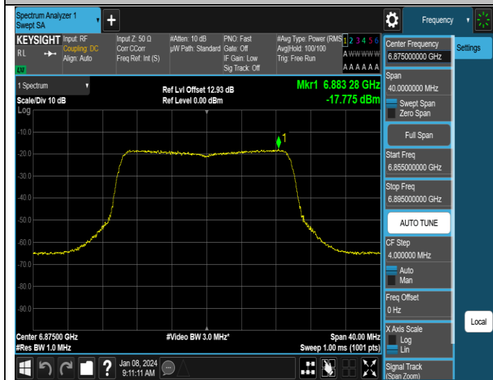
11AX20MIMO-Ant1-6875-PASS
