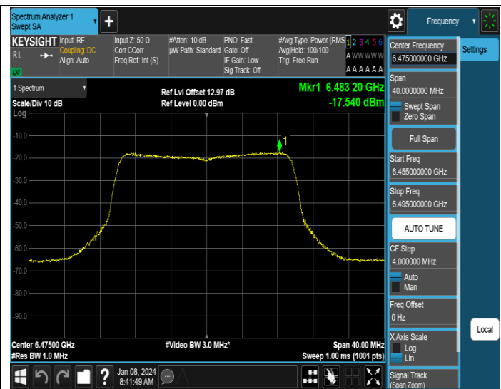
11AX20MIMO-Ant2-6475-PASS
