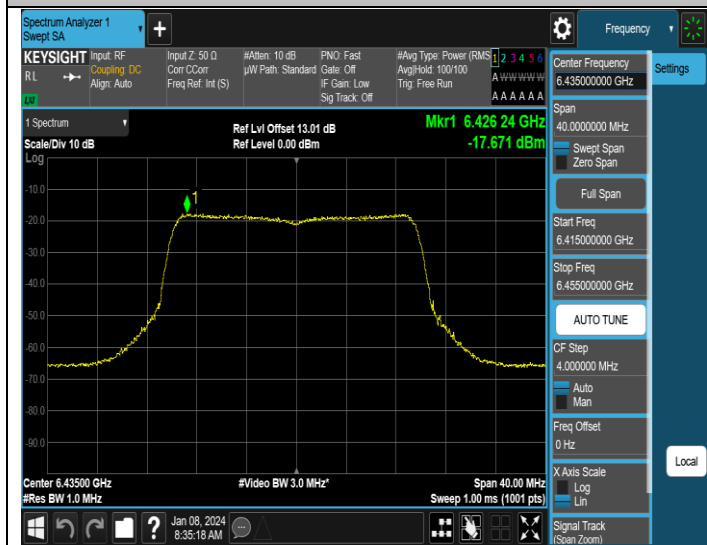
11AX20MIMO-Ant1-6435-PASS
