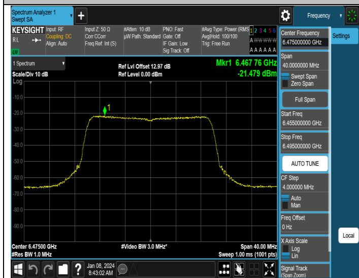
11AX20MIMO-Ant3-6475-PASS
