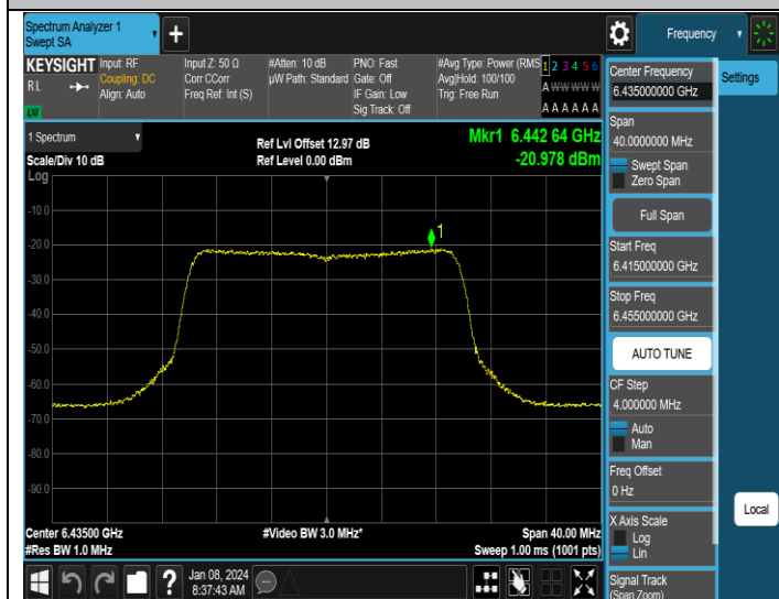
11AX20MIMO-Ant3-6435-PASS
