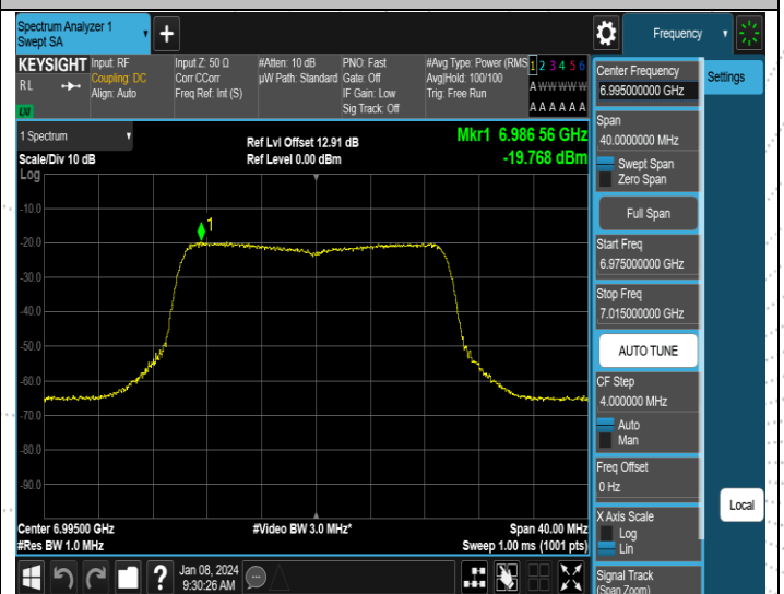
11AX20MIMO-Ant2-6995-PASS
