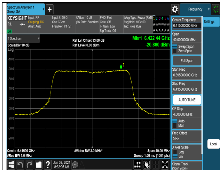
11AX20MIMO-Ant3-6415-PASS
