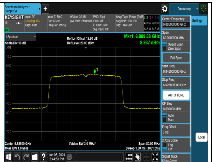
11AX40SISO-Ant4-6885-PASS
