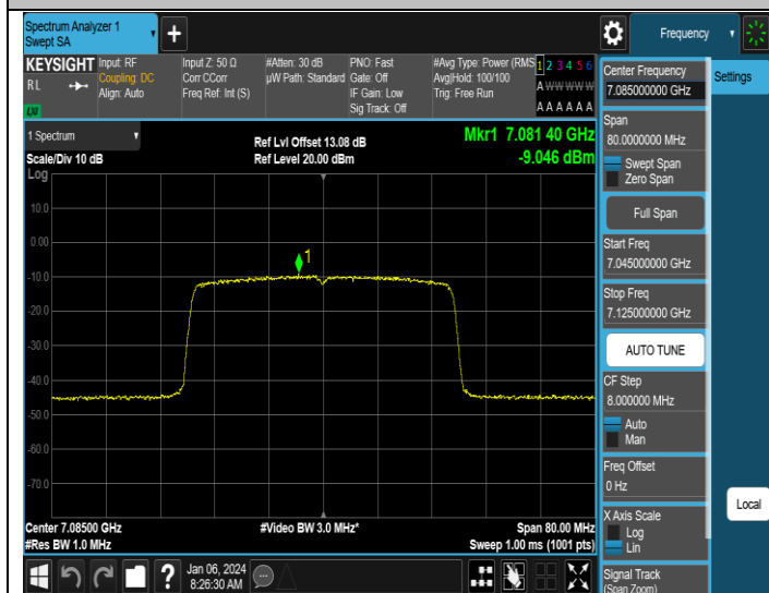
11AX40SISO-Ant1-7085-PASS
