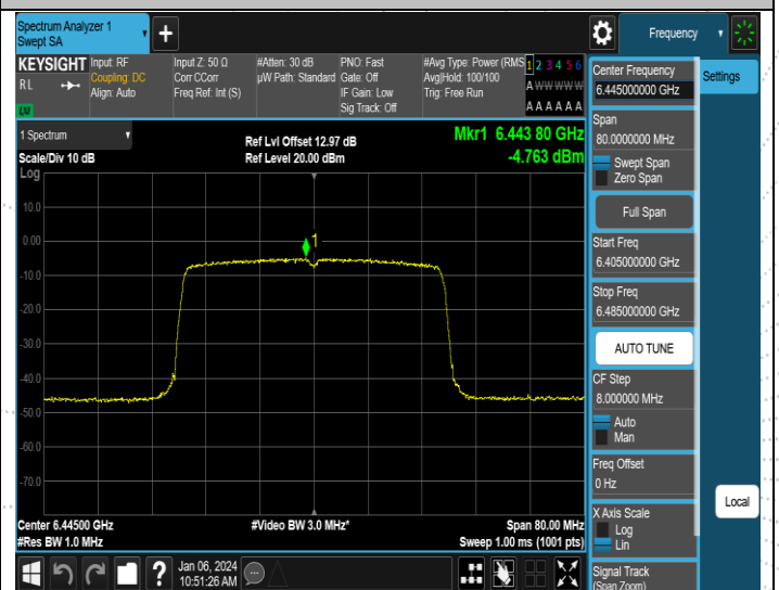
11AX40SISO-Ant2-6445-PASS
