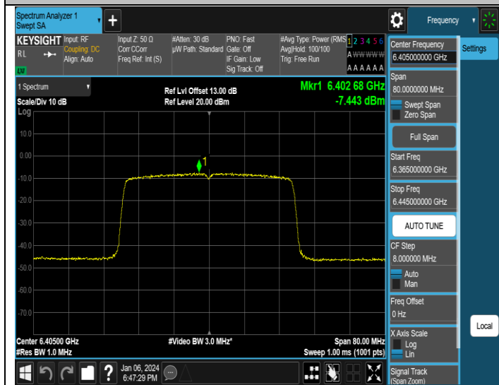
11AX40SISO-Ant3-6405-PASS
