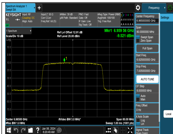
11AX40SISO-Ant1-6965-PASS
