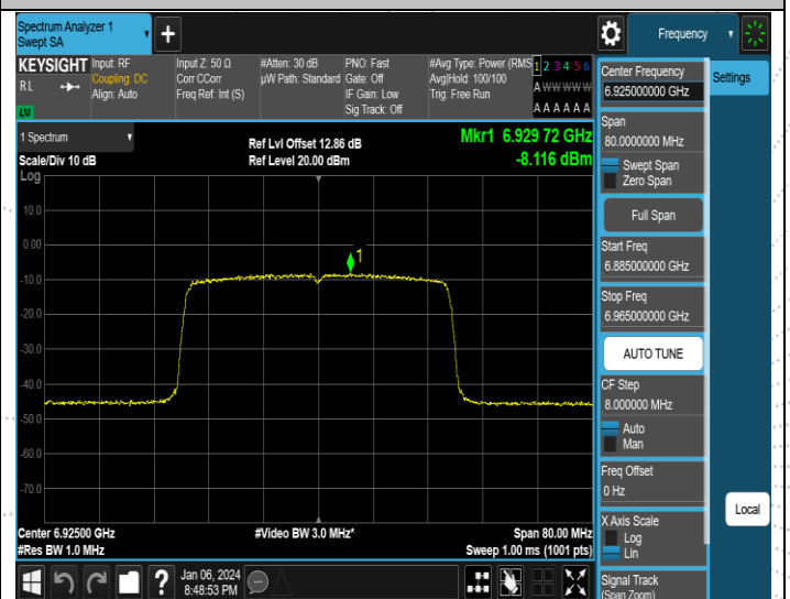
11AX40SISO-Ant4-6925-PASS
