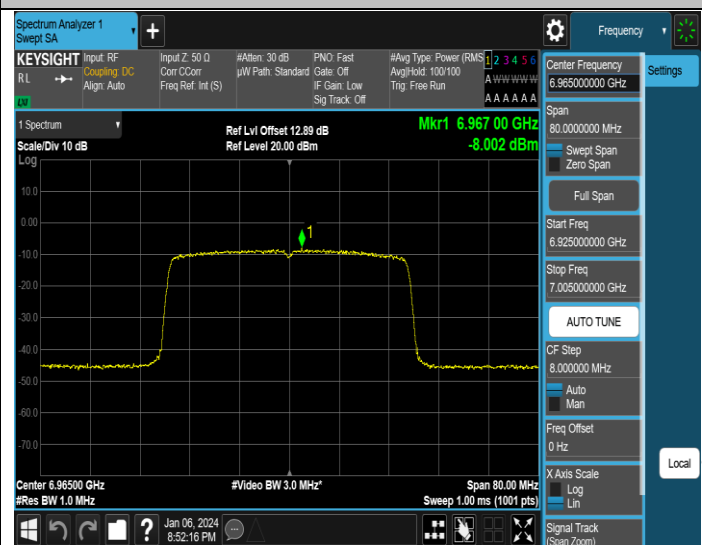
11AX40SISO-Ant4-6965-PASS
