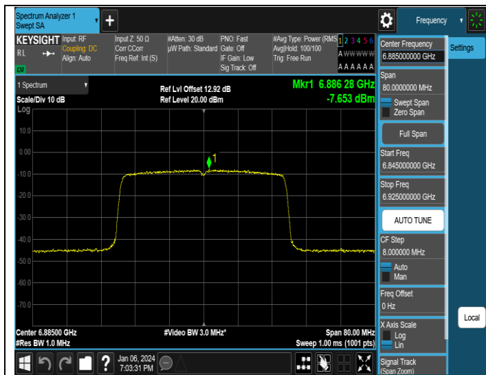
11AX40SISO-Ant3-6885-PASS
