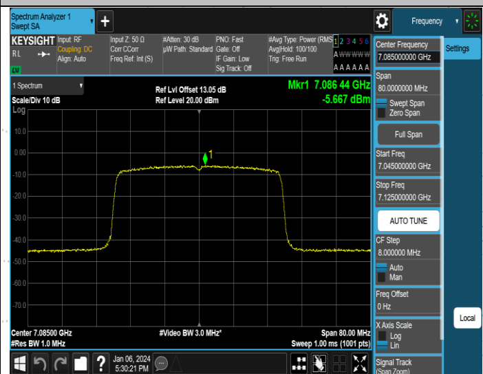
11AX40SISO-Ant2-7085-PASS
