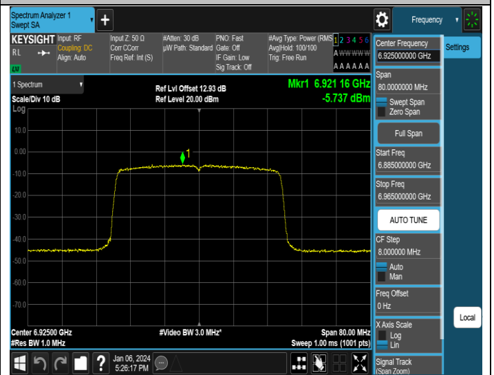
11AX40SISO-Ant2-6925-PASS
