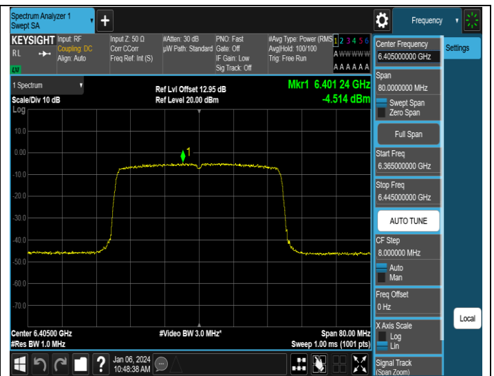
11AX40SISO-Ant2-6405-PASS
