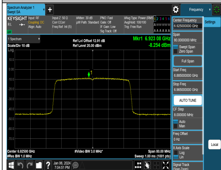
11AX40SISO-Ant3-6925-PASS
