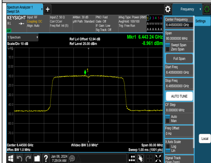
11AX40SISO-Ant1-6445-PASS
