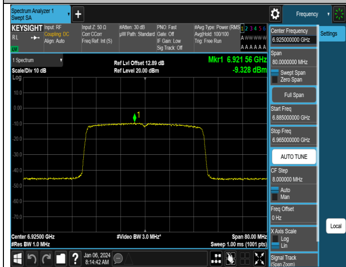
11AX40SISO-Ant1-6925-PASS
