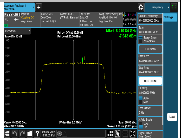
11AX40SISO-Ant4-6405-PASS
