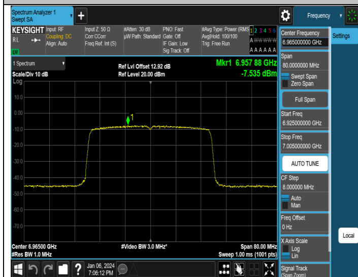
11AX40SISO-Ant3-6965-PASS
