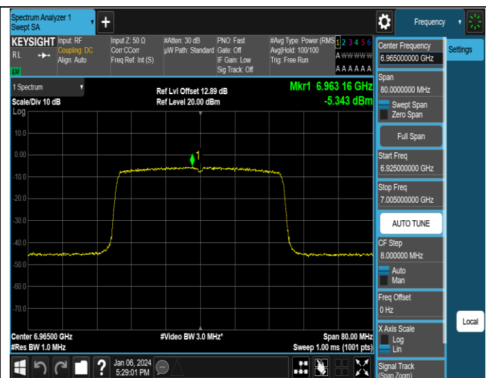
11AX40SISO-Ant2-6965-PASS
