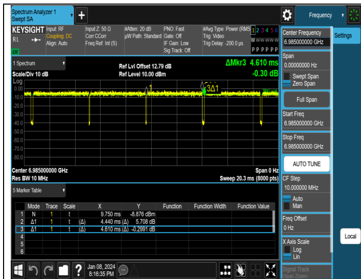
NTNV-11AX160MIMO-Ant1-6985
