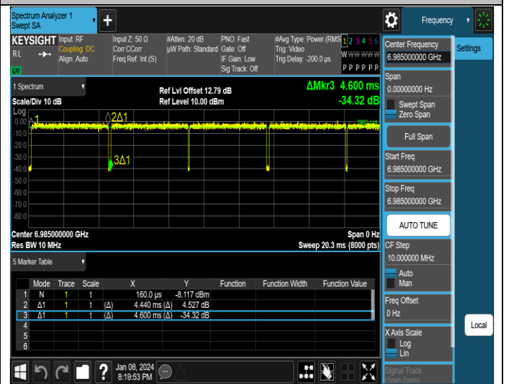
NTNV-11AX160MIMO-Ant4-6985
