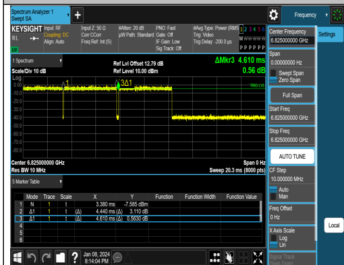
NTNV-11AX160MIMO-Ant3-6825
