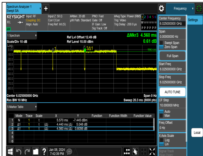
NTNV-11AX160MIMO-Ant1-6025
