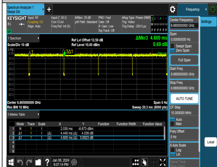
NTNV-11AX160MIMO-Ant1-6665
