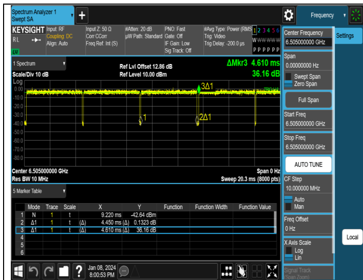
NTNV-11AX160MIMO-Ant1-6505
