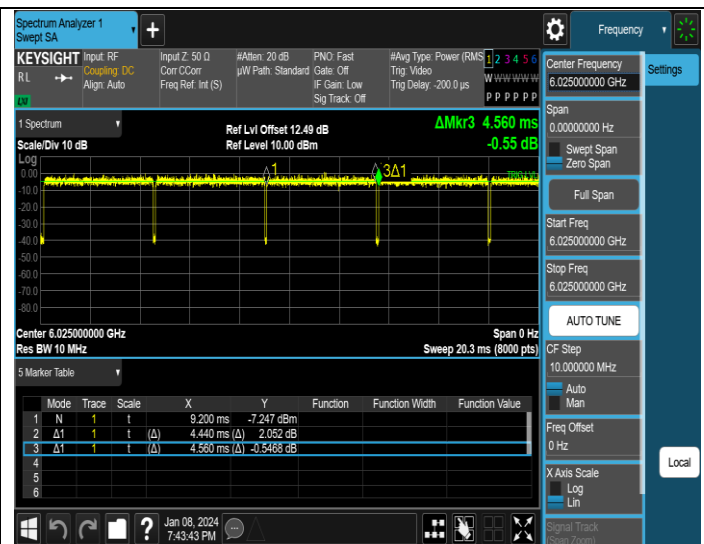
NTNV-11AX160MIMO-Ant2-6025
