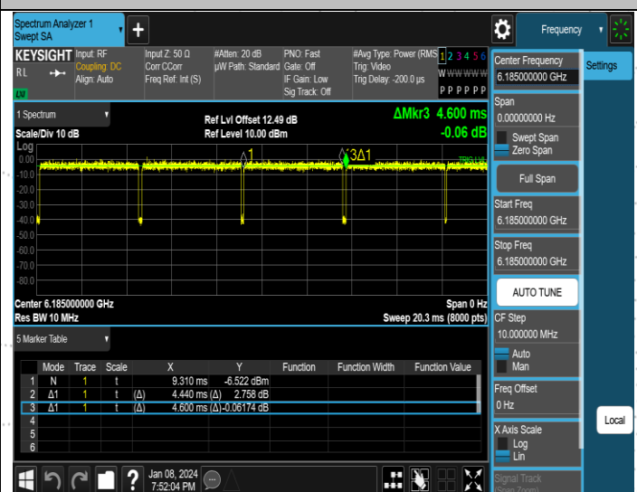
NTNV-11AX160MIMO-Ant2-6185
