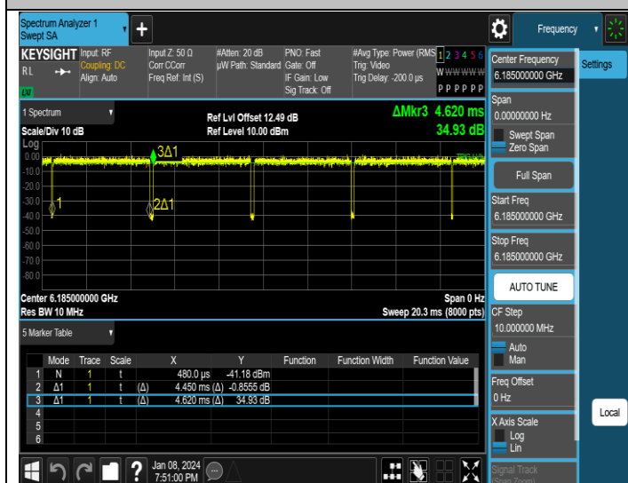
NTNV-11AX160MIMO-Ant1-6185
