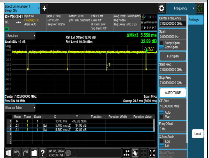
NTNV-11AX80MIMO-Ant2-7025
