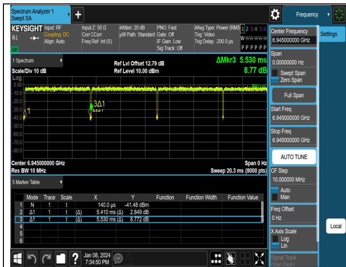
NTNV-11AX80MIMO-Ant3-6945
