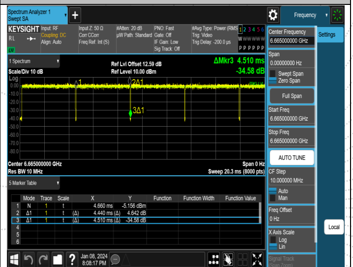
NTNV-11AX160MIMO-Ant2-6665
