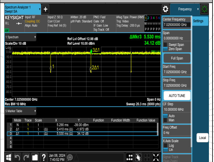
NTNV-11AX80MIMO-Ant4-7025
