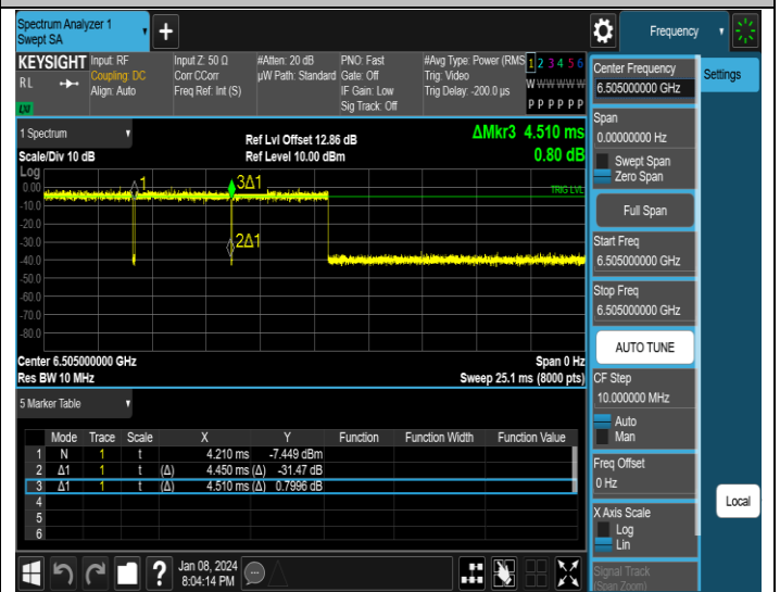
NTNV-11AX160MIMO-Ant4-6505
