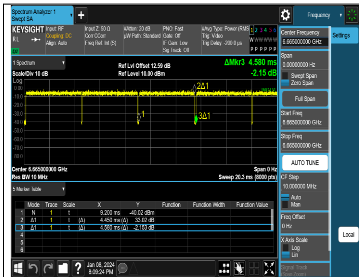
NTNV-11AX160MIMO-Ant3-6665
