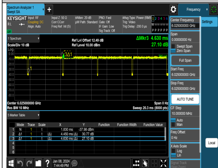
NTNV-11AX160MIMO-Ant3-6025
