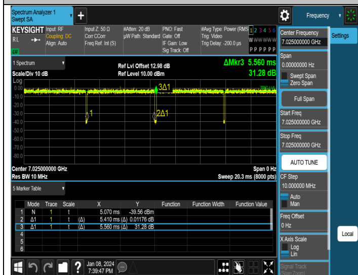
NTNV-11AX80MIMO-Ant3-7025
