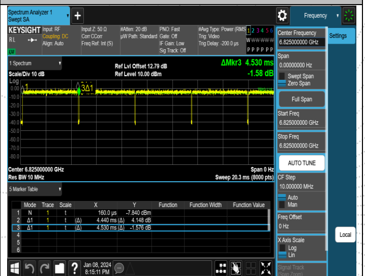
NTNV-11AX160MIMO-Ant4-6825
