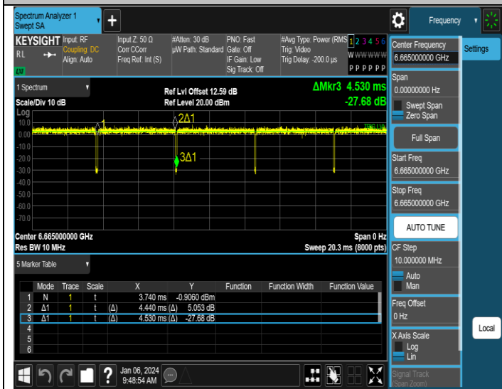
NTNV-11AX160SISO-Ant1-6665
