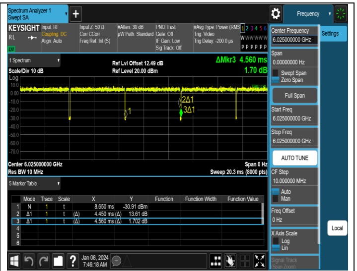
NTNV-11AX160SISO-Ant4-6025
