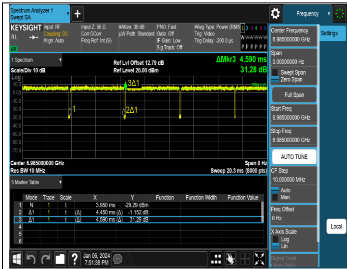
NTNV-11AX160SISO-Ant3-6985
