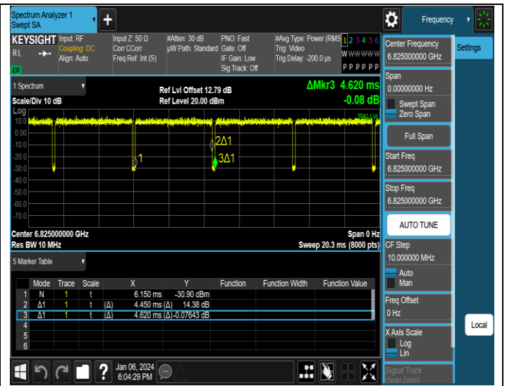
NTNV-11AX160SISO-Ant2-6825
