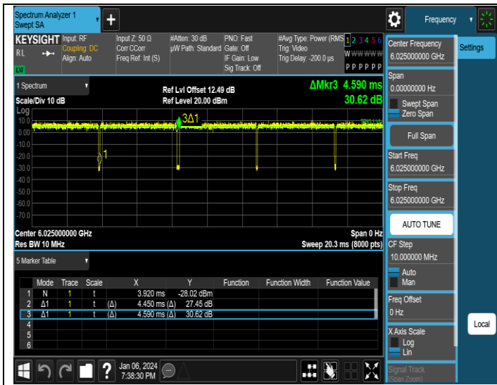
NTNV-11AX160SISO-Ant3-6025
