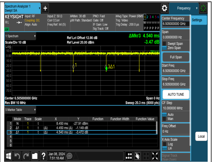
NTNV-11AX160SISO-Ant4-6505
