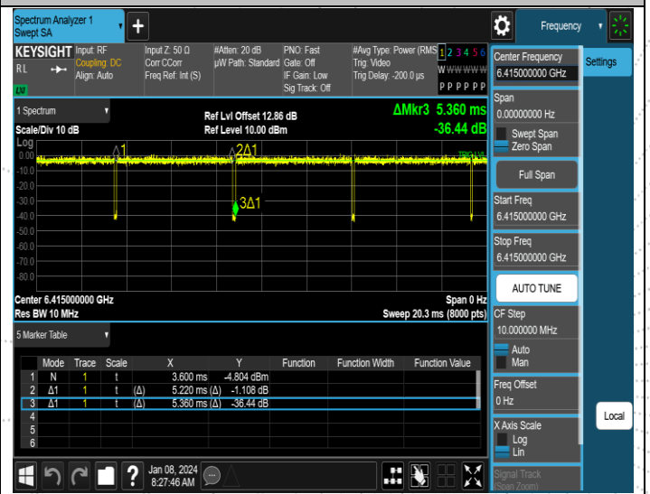
NTNV-11AX20MIMO-Ant2-6415
