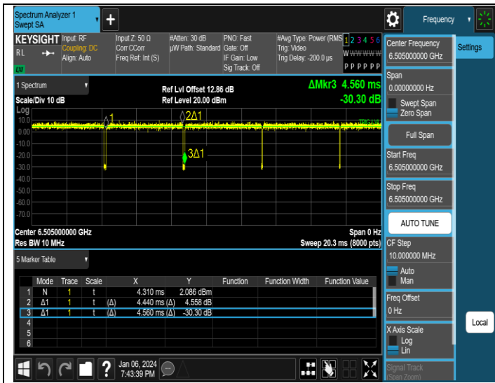
NTNV-11AX160SISO-Ant3-6505
