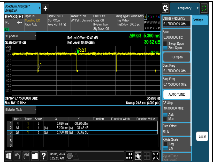
NTNV-11AX20MIMO-Ant2-6175
