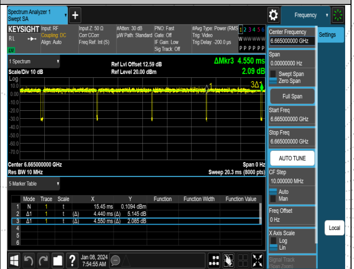
NTNV-11AX160SISO-Ant4-6665
