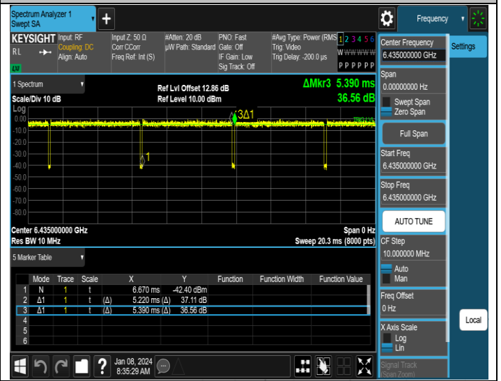
NTNV-11AX20MIMO-Ant2-6435
