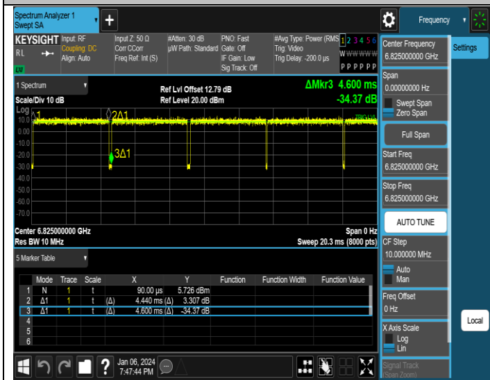
NTNV-11AX160SISO-Ant3-6825
