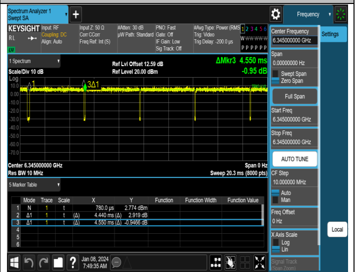
NTNV-11AX160SISO-Ant4-6345
