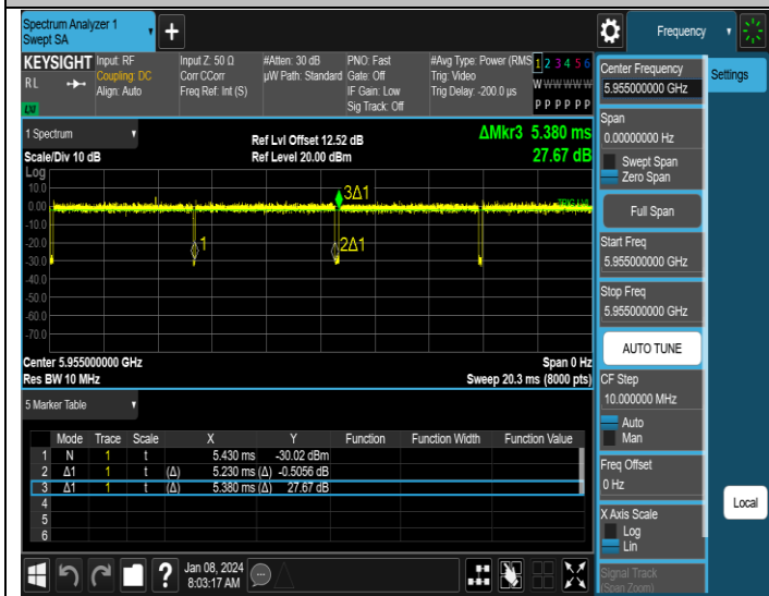
NTNV-11AX20MIMO-Ant1-5955
