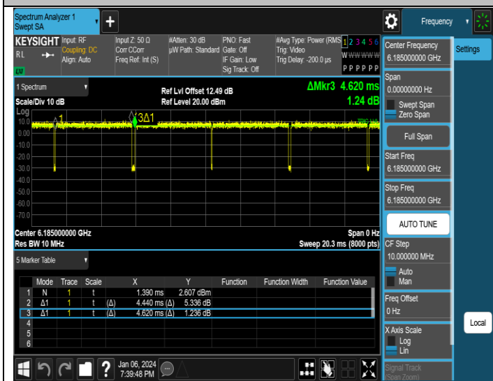
NTNV-11AX160SISO-Ant3-6185
