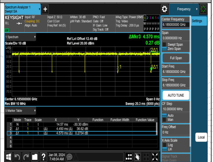
NTNV-11AX160SISO-Ant4-6185
