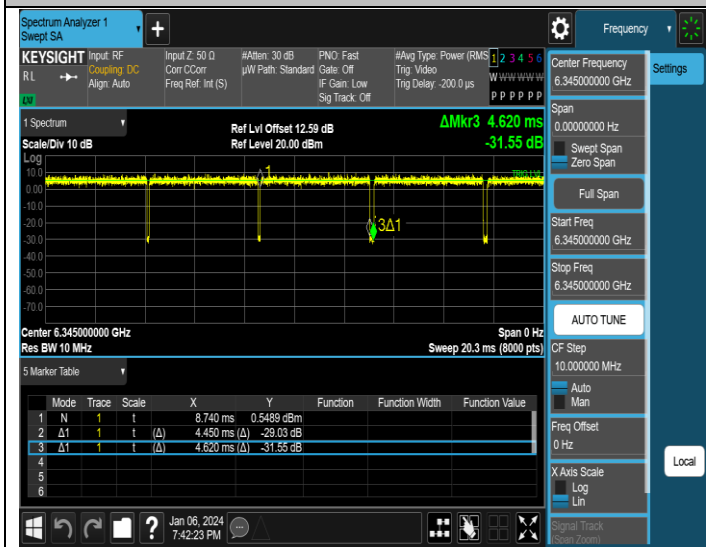
NTNV-11AX160SISO-Ant3-6345
