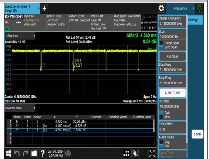
NTNV-11AX160SISO-Ant2-6185
