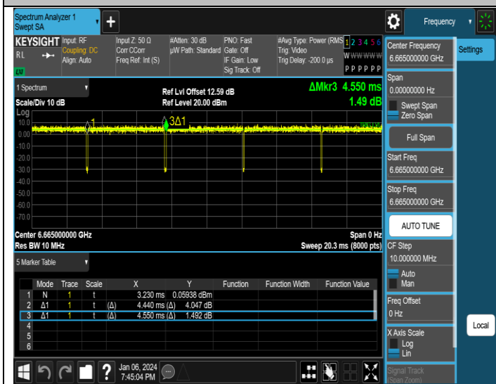
NTNV-11AX160SISO-Ant3-6665
