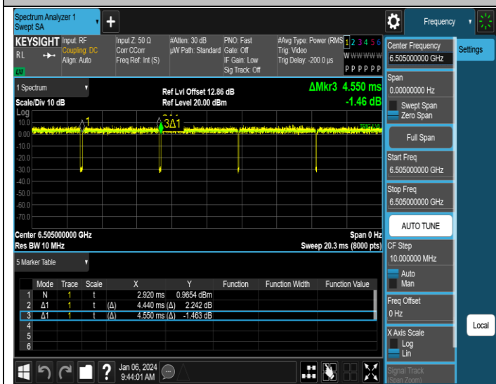
NTNV-11AX160SISO-Ant1-6505
