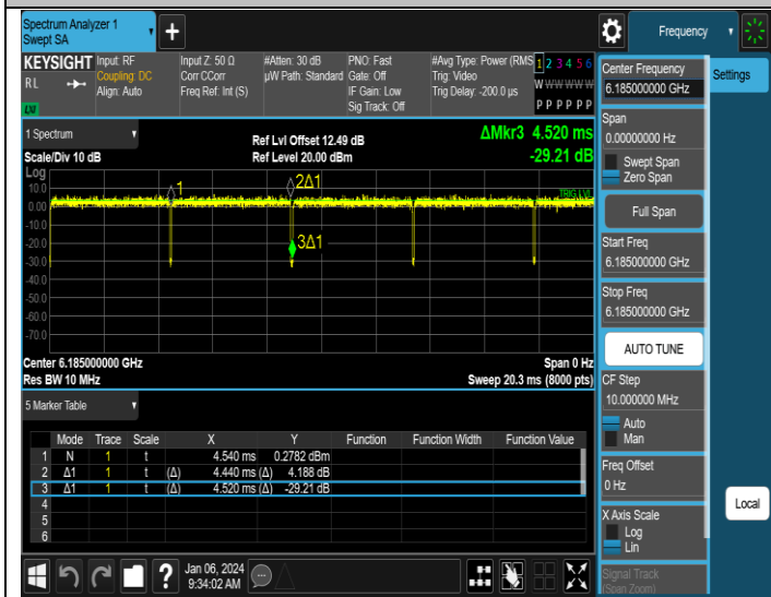
NTNV-11AX160SISO-Ant1-6185
