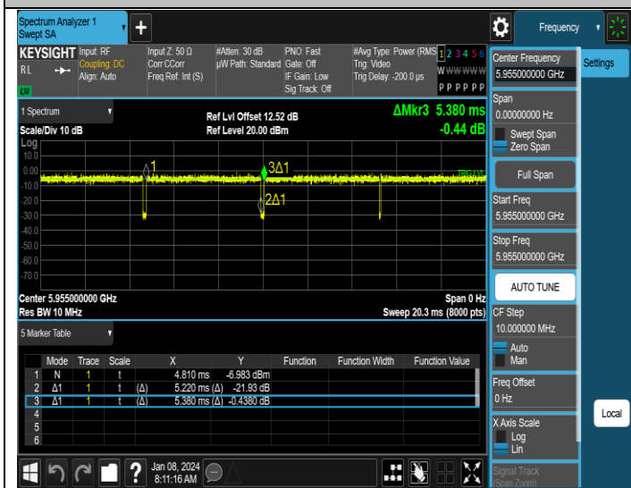
NTNV-11AX20MIMO-Ant3-5955
