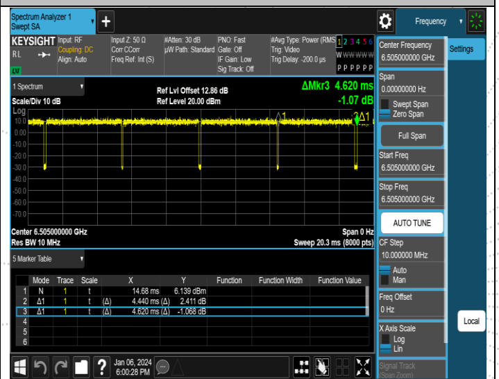
NTNV-11AX160SISO-Ant2-6505
