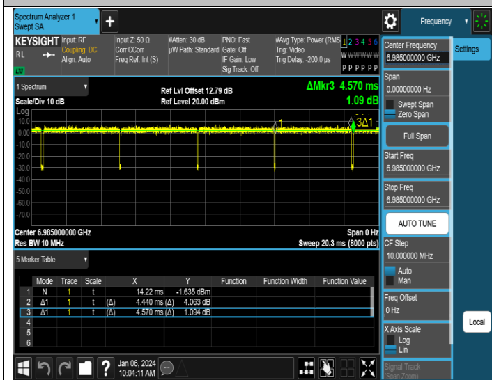
NTNV-11AX160SISO-Ant1-6985
