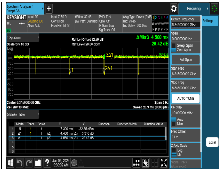
NTNV-11AX160SISO-Ant1-6345
